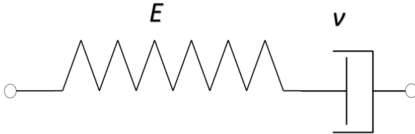
Figure 2.1. Maxwell Model
