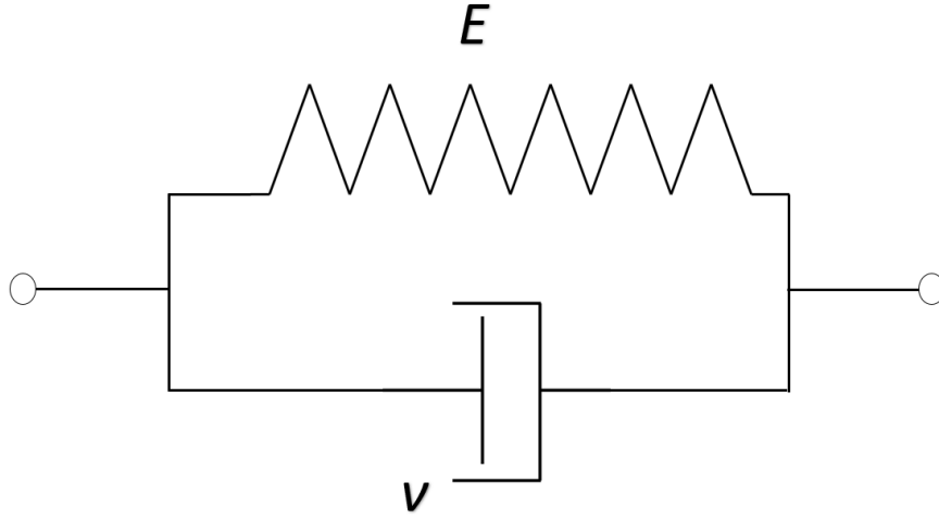
Figure 2.2. Kelvin – Voigt Model
