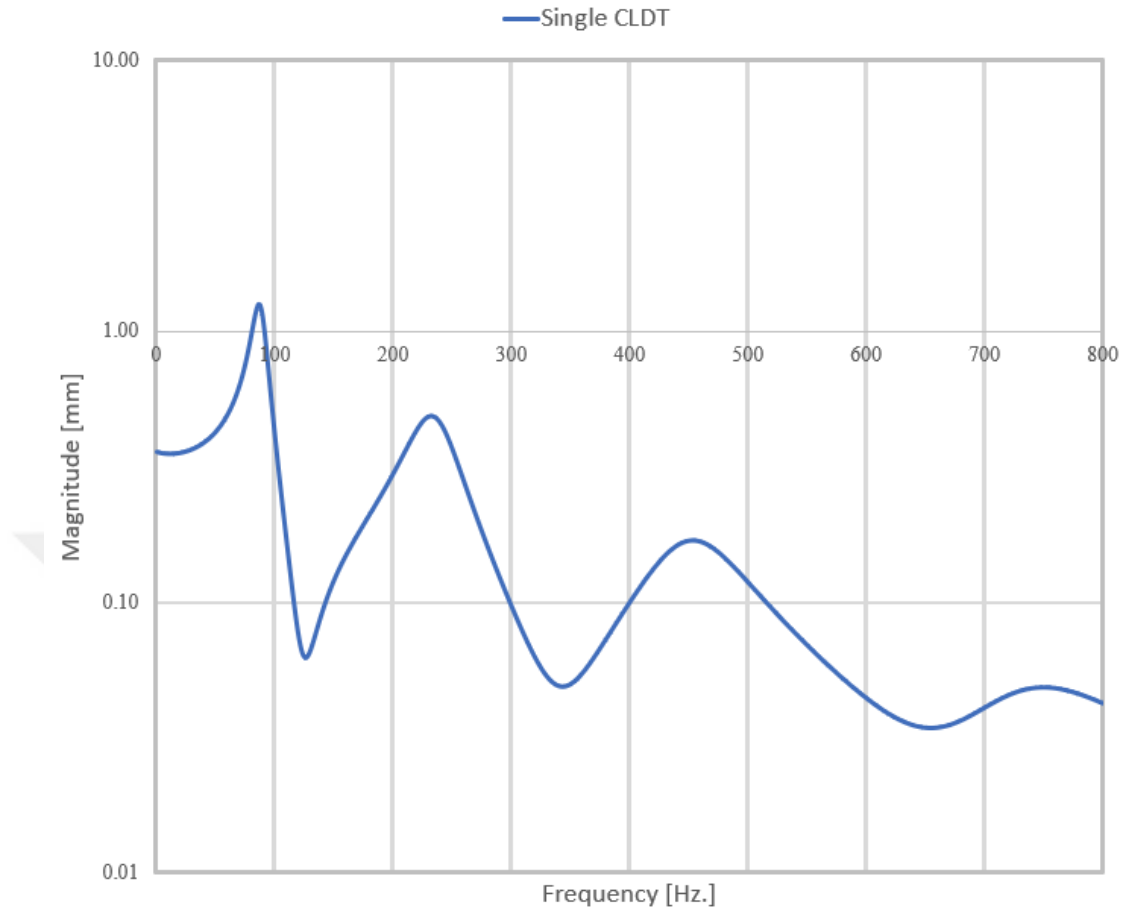
Figure 3.20. The FRF Plot of the Reference Single CLDT Beam
