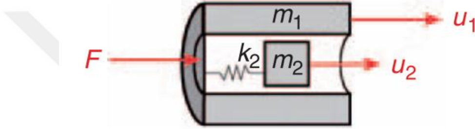
Figure 2.8. 2-DOF mass-in-mass structure [3]
