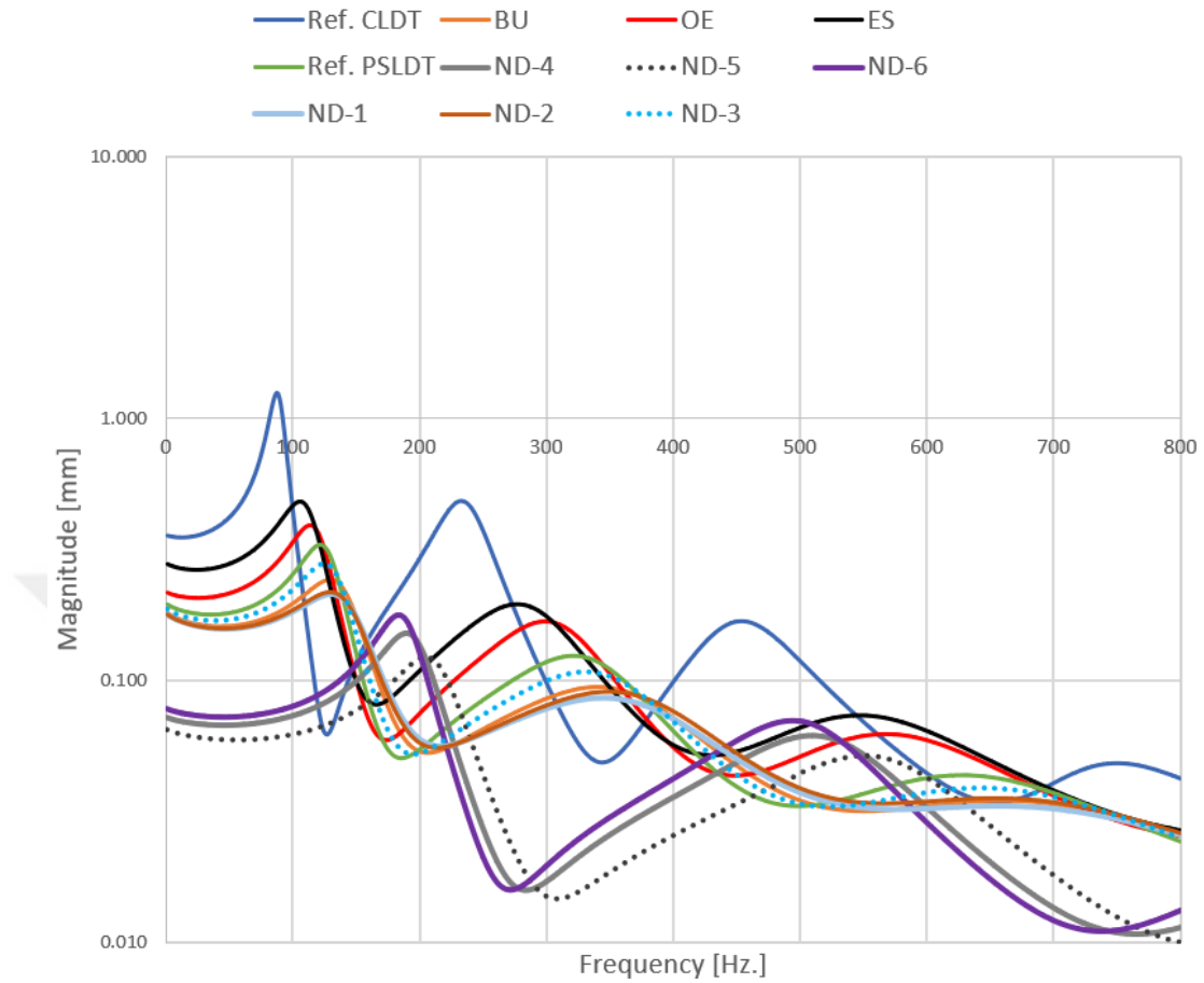
Figure 4.25. The FRF Comparison Plot for Reference Baseline Configurations and Novel Design Alternatives
