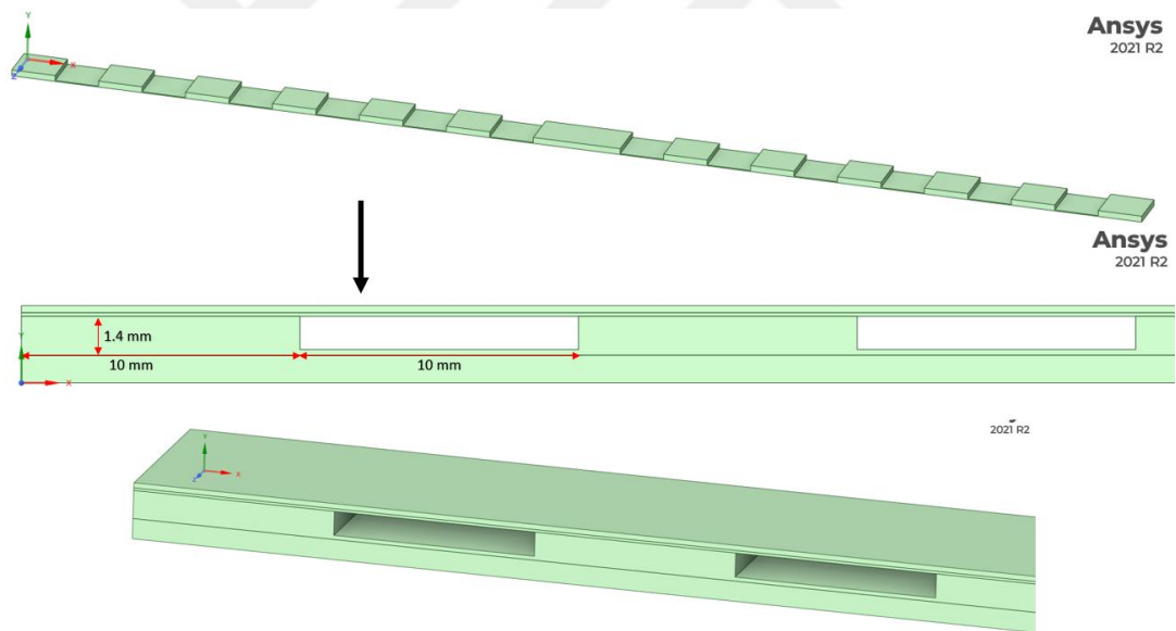
Figure 4.14. Novel Design Alternative (ND-2)
