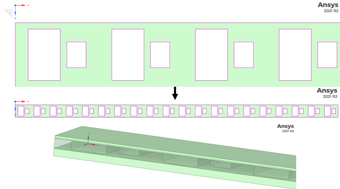
Figure 4.18. Novel Design Alternative (ND-4)
