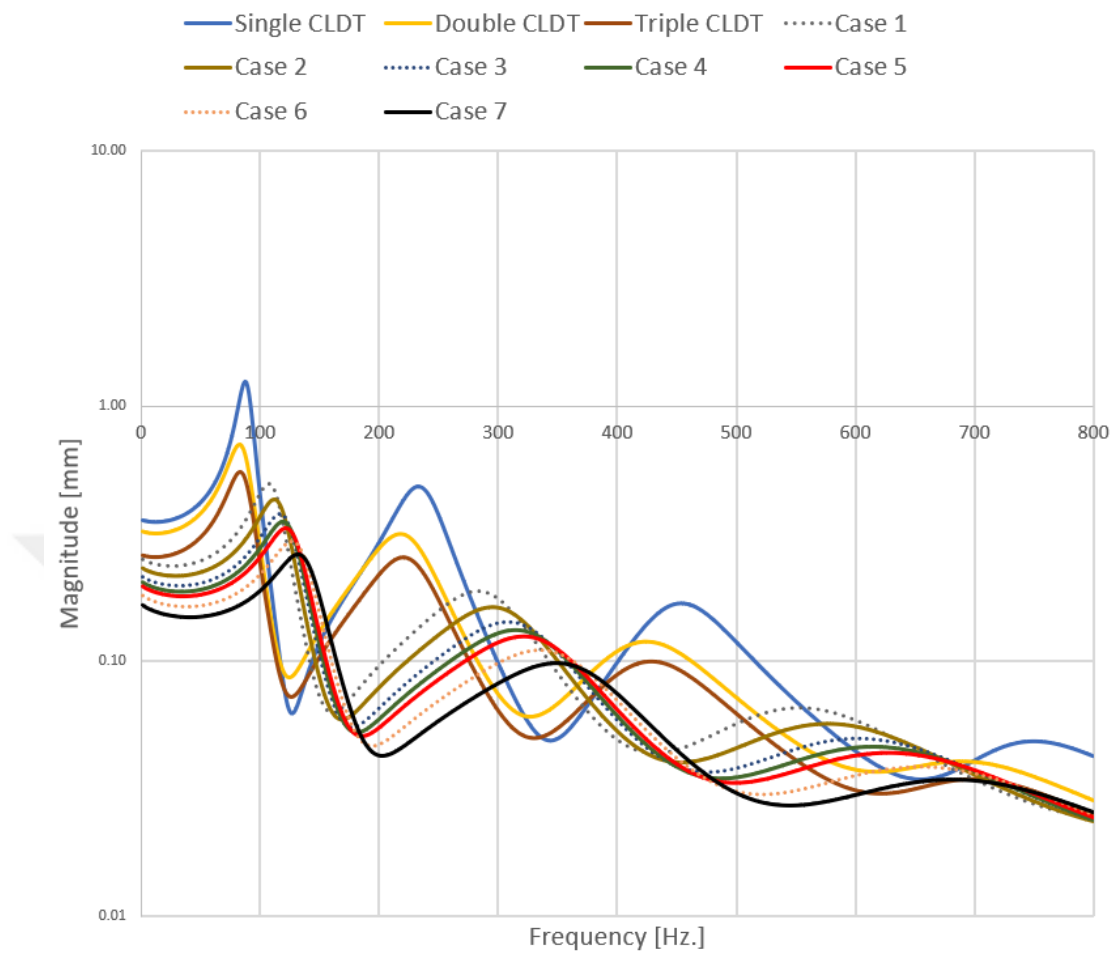
Figure 3.22. The FRF Comparison Plot for the Optimization Cases
