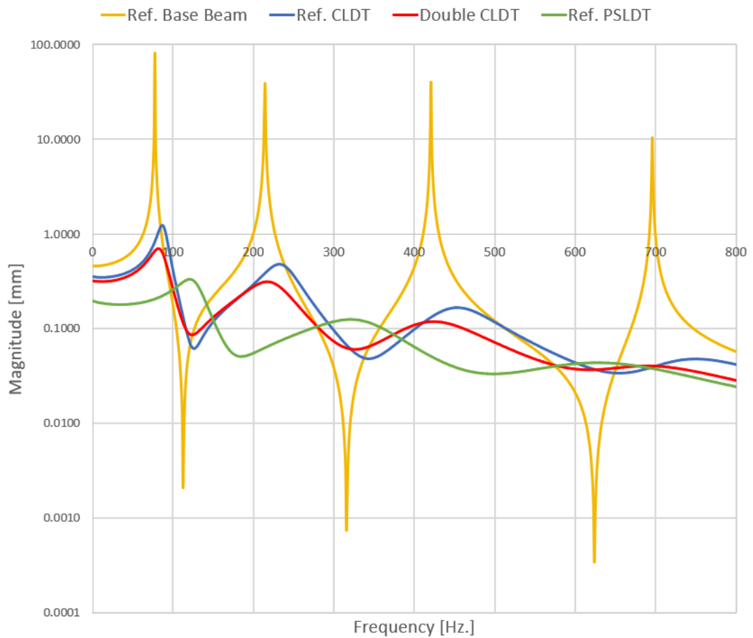
Figure 4.2. The FRF Comparison Plot between Reference Baseline Configurations
