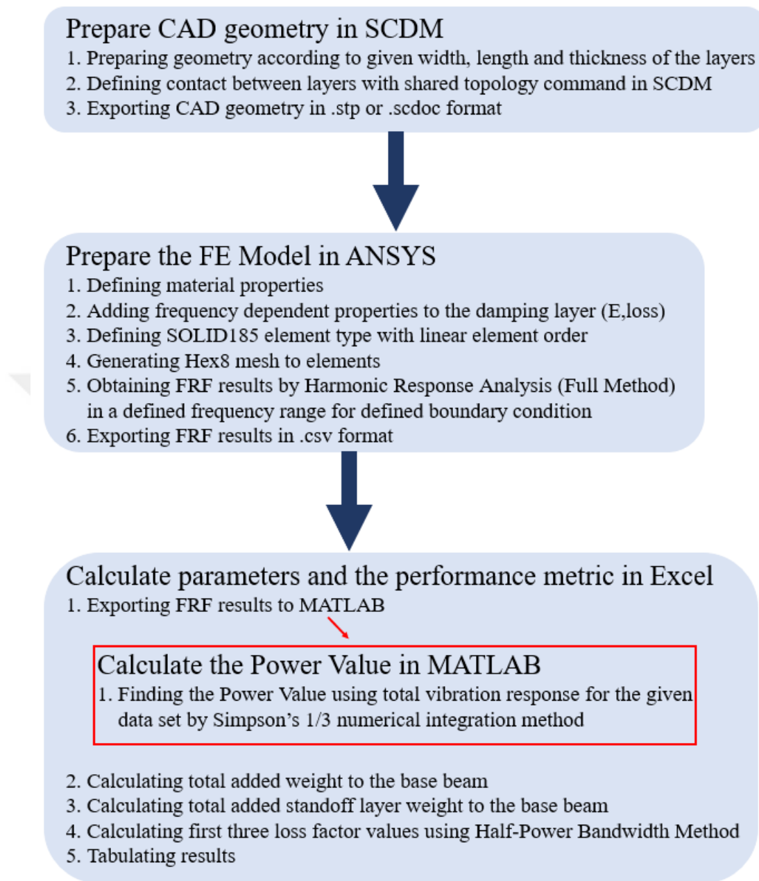
Figure 3.13. The Proposed Methodology to Find Unknown Parameters
