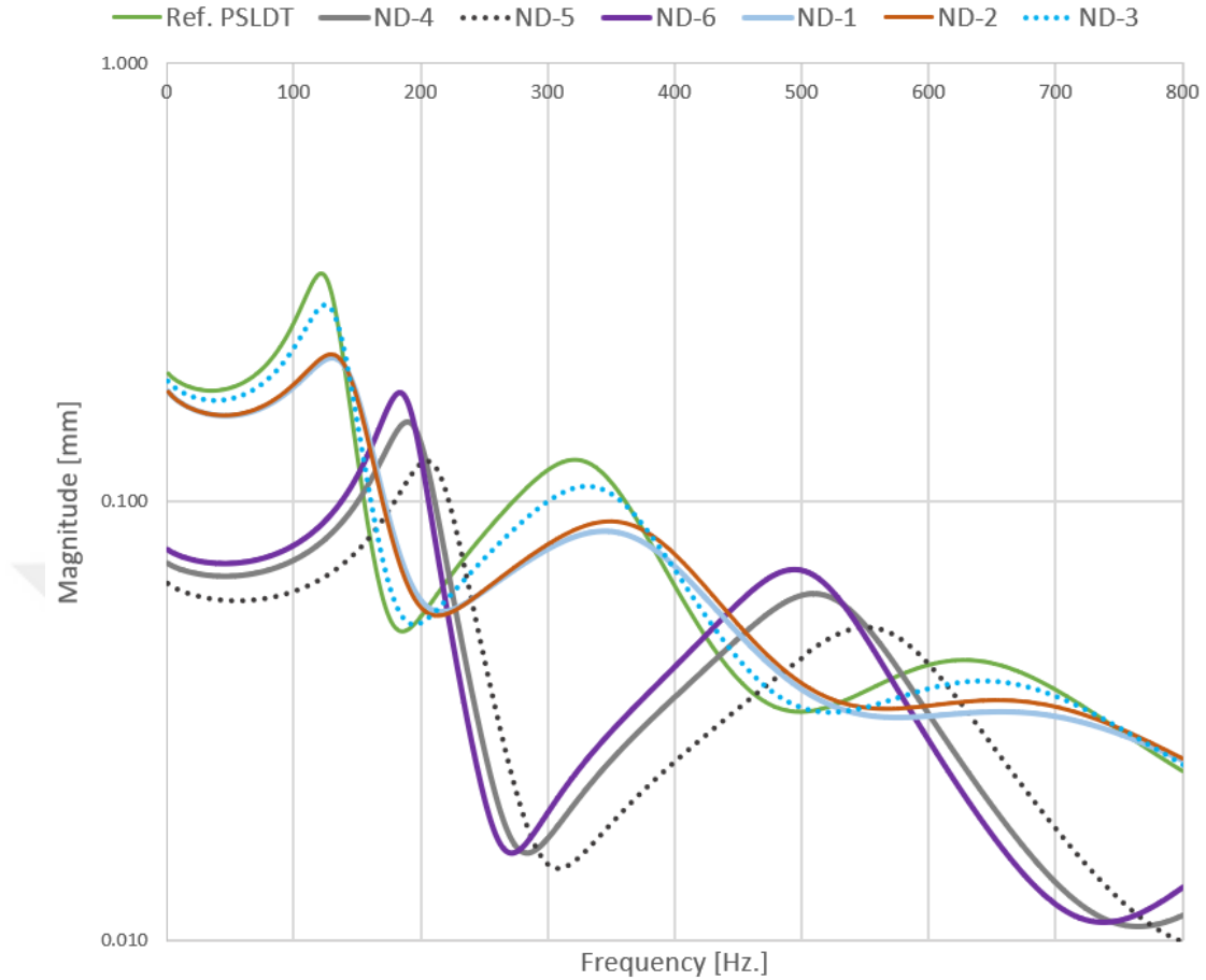
Figure 4.26. The FRF Comparison Plot for Novel Design Alternatives
