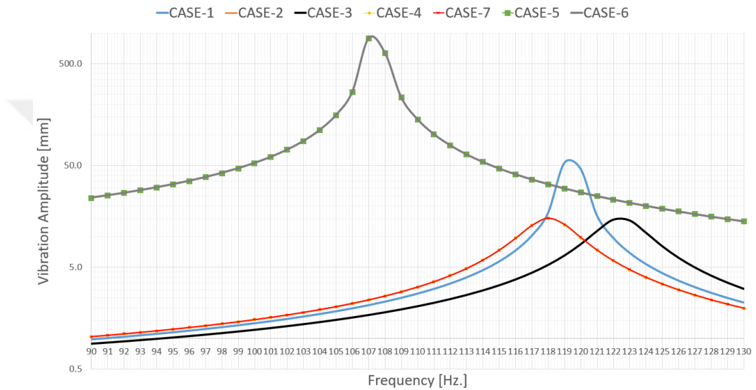
Figure 3.4. The FRF Comparison for Cases in Analysis
