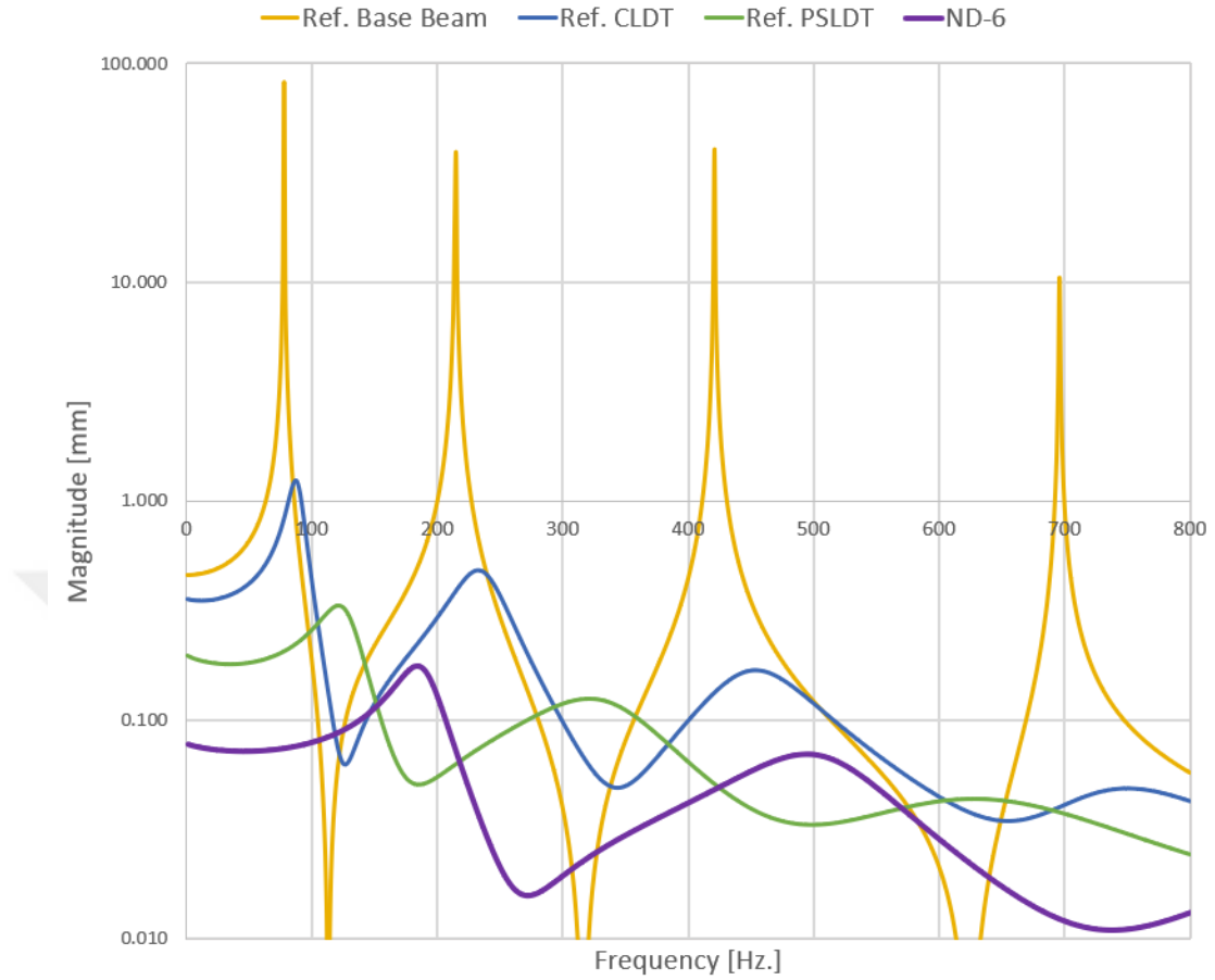
Figure 4.24. The FRF Comparison Plot for Novel Design Alternative (ND-6)
