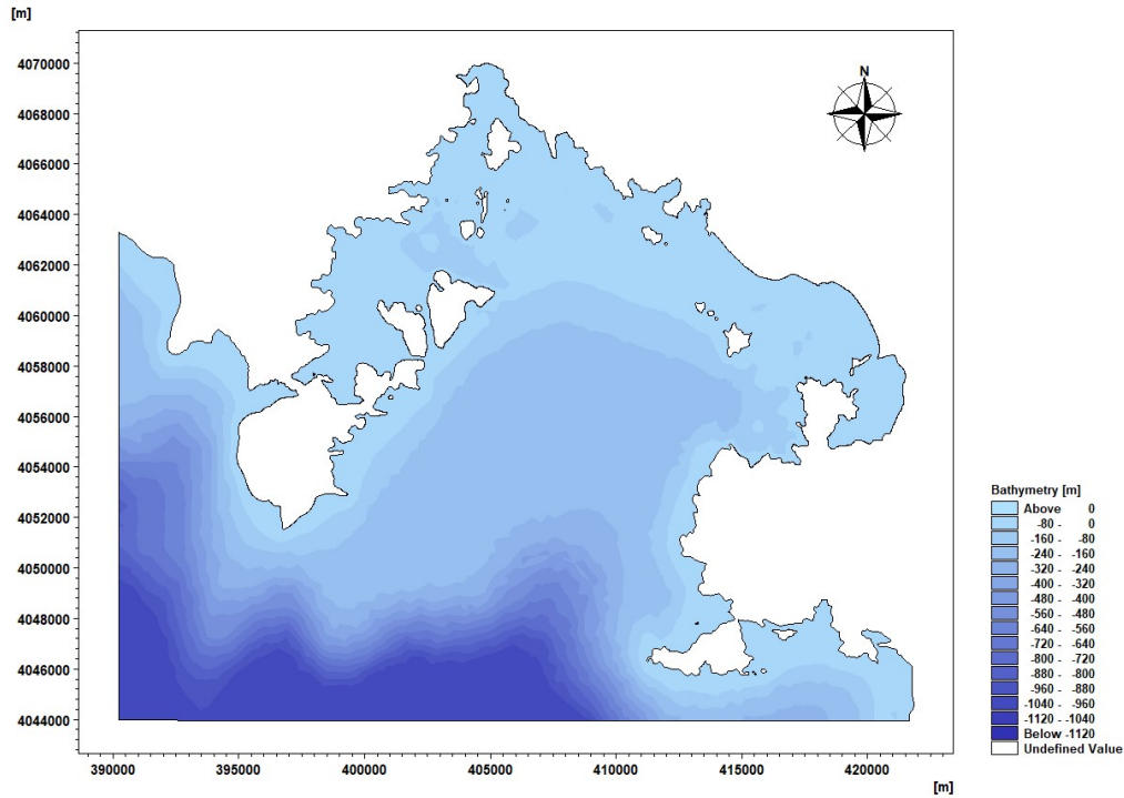
Figure 5.1. Bathymetry of Fethiye and Göcek Bays
