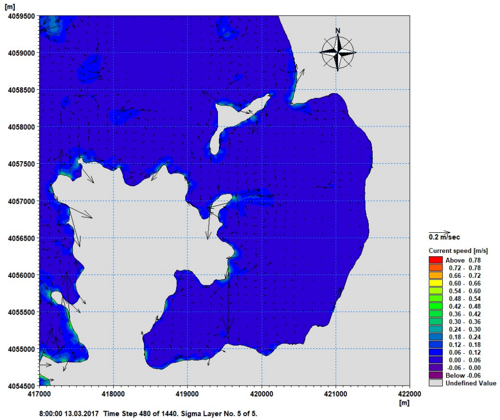
Figure A.1. Circulation pattern at Fethiye Bay at 8 th hour under 24 hours of Coriolis forcing
