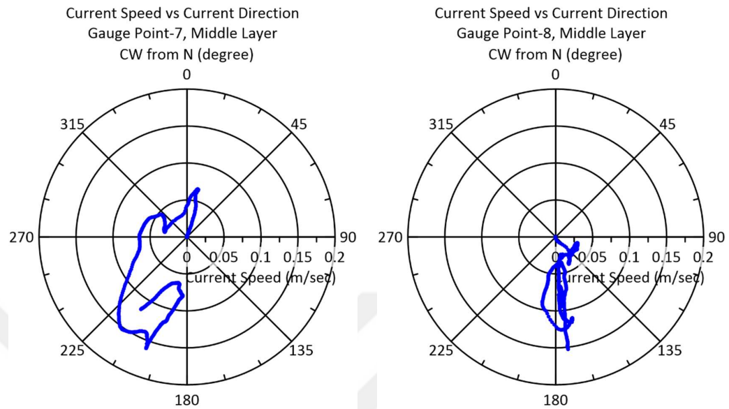
Figure 6.34. Current speed and current direction at Gauge Point 7 and Gauge Point 8 (5 m/sec wind blowing from WSW direction)
