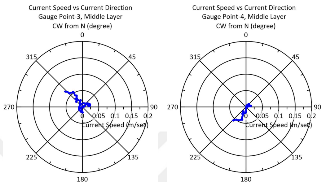
Figure 6.37. Current speed and current direction at Gauge Point 3 and Gauge Point 4 (5 m/sec wind blowing from NNW direction)
