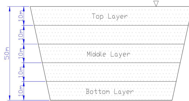
Figure 6.2. Vertical domain
