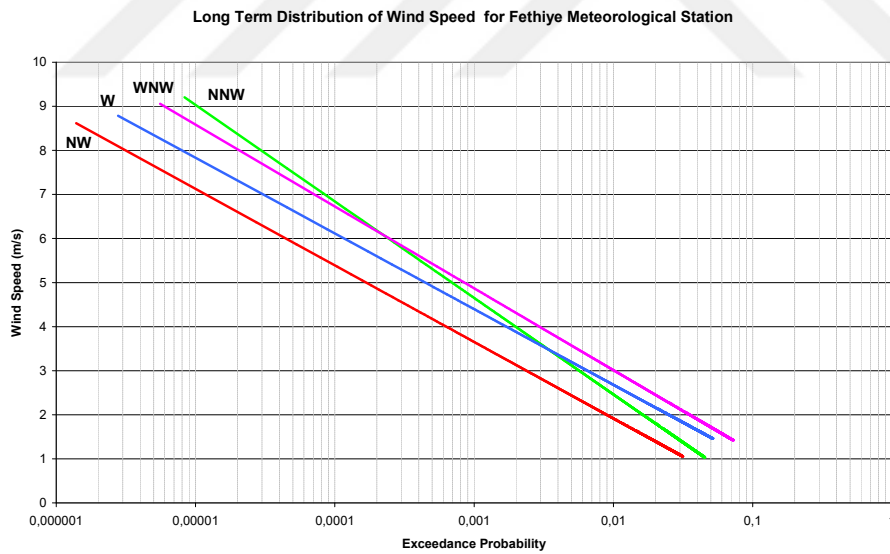
Figure 5.13. Long-term exceedance probability of wind speeds for NW, W, WNW, NNW directions for Fethiye Meteorological Station (Akbaşoğlu, 2011)
