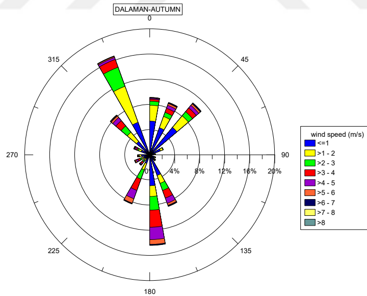
Figure 5.15. Dalaman Wind Rose - Autumn (Akbaşıoğlu, 2011)
