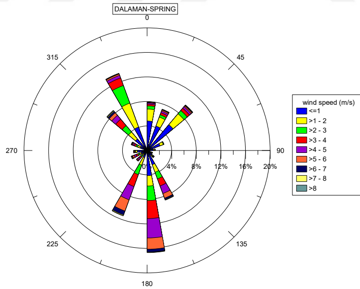
Figure 5.17. Dalaman Wind Rose - Spring (Akbaşoğlu, 2011)
