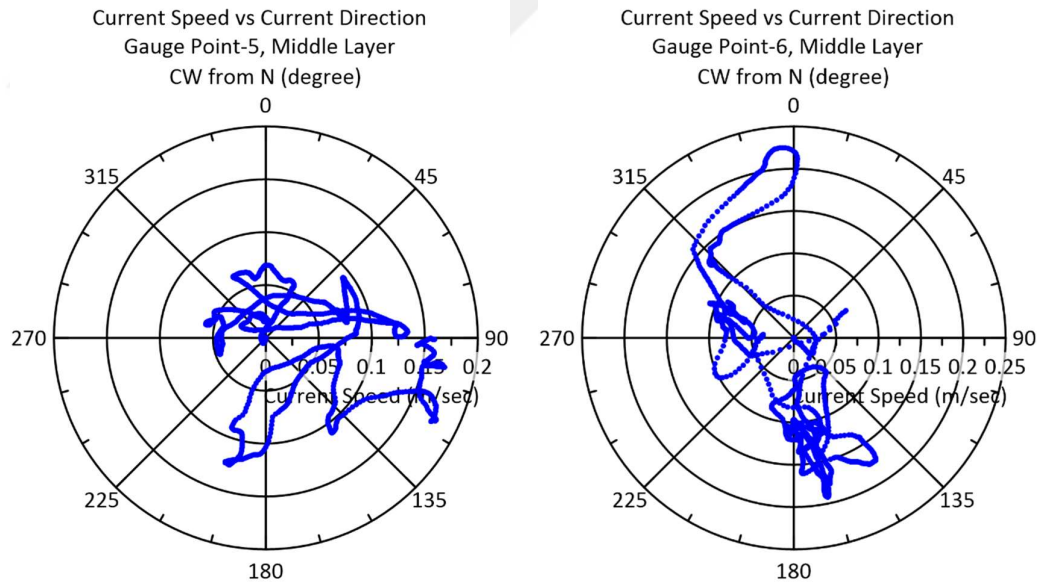
Figure 6.11. Current speed and current direction at Gauge Point 5 and Gauge Point 6 (24-hours simulation of Coriolis force only)
