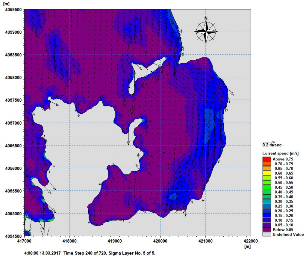
Figure J.1. Circulation pattern at Fethiye Bay at 4 th hour under 12 hours of wind forcing (Wind Speed: 10 m/sec, Wind Direction: NNW)
