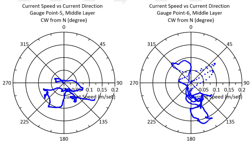
Figure 6.38. Current speed and current direction at Gauge Point 5 and Gauge Point 6 (5 m/sec wind blowing from NNW direction)
