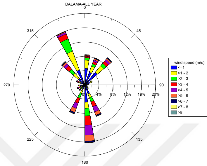
Figure 5.14. Dalaman Wind Rose - All year (Akbaşıoğlu, 2011)
