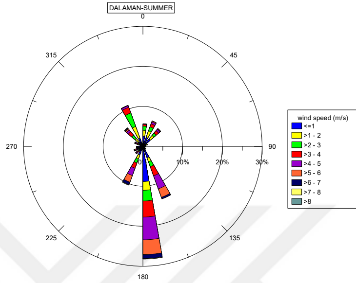
Figure 5.18. Dalaman Wind Rose - Summer (Akbaşıoğlu, 2011)
