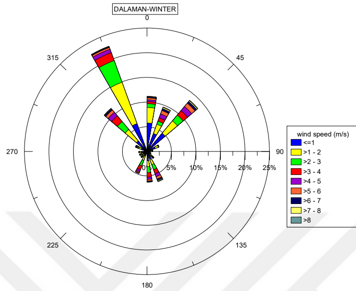
Figure 5.16. Dalaman Wind Rose - Winter (Akbaşoğlu, 2011)
