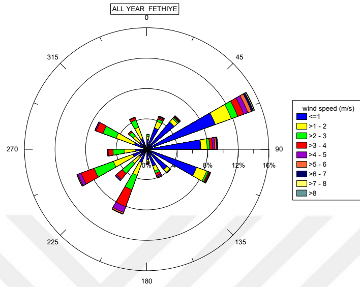
Figure 5.5. Fethiye Wind Rose - All year (Akbaşoğlu, 2011)
