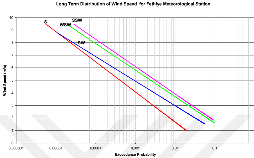
Figure 5.12. Long-term exceedance probability of wind speeds for S, SW, WSW, SSW directions for Fethiye Meteorological Station (Akbaşoğlu, 2011)
