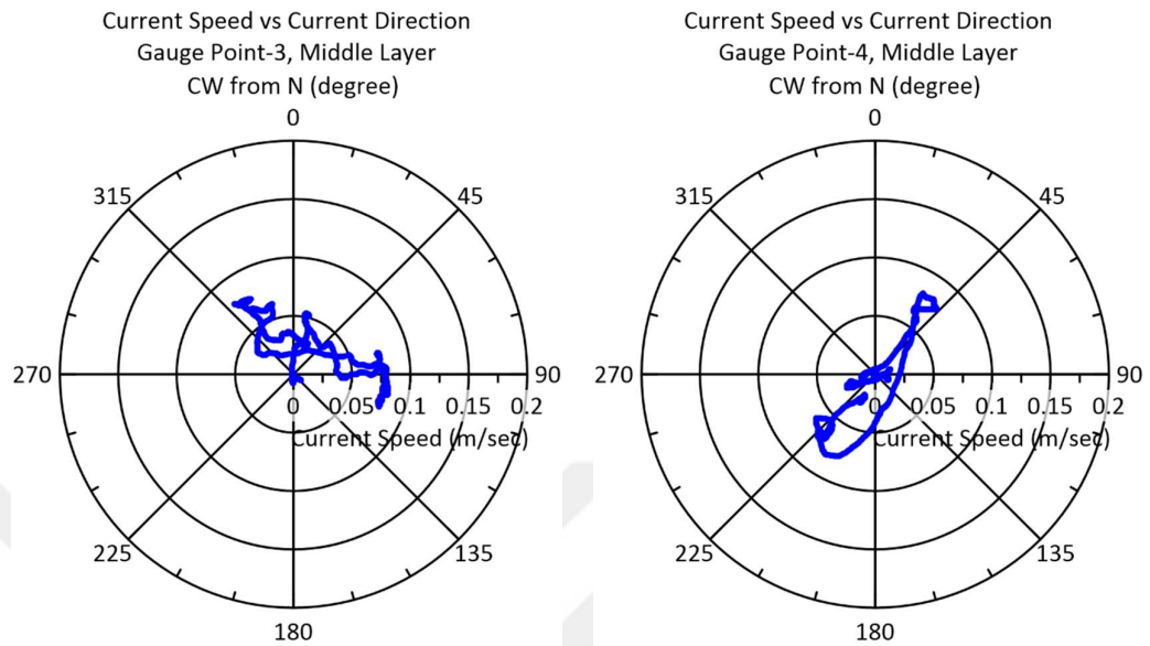
Figure 6.10. Current speed and current direction at Gauge Point 3 and Gauge Point 4 (24-hours simulation of Coriolis force only)
