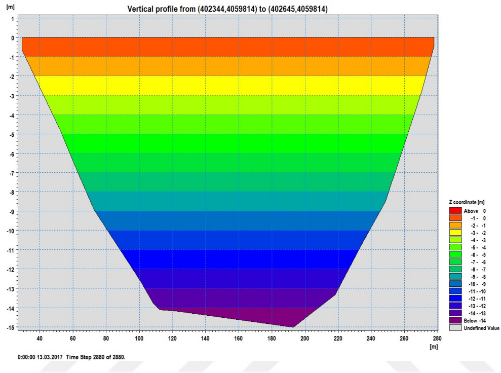
Figure K.8. Cross-section for strait 8
