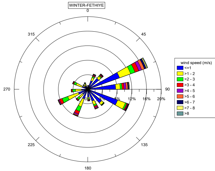
Figure 5.7. Fethiye Wind Rose - Winter (Akbaşıoğlu, 2011)
