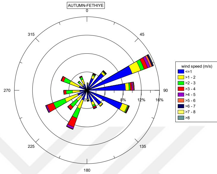
Figure 5.6. Fethiye Wind Rose - Autumn (Akbaşıoğlu, 2011)
