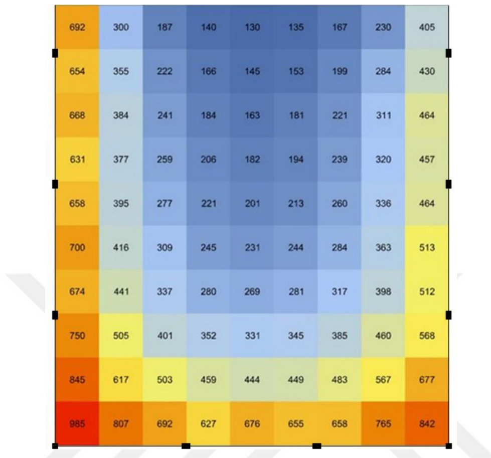
Figure 4.16 Illuminance results in lux of the ground floor of the design case 1 on the 8 th of June at 1 pm
