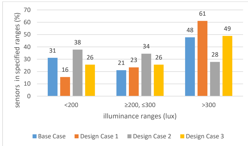
Figure 4.44 The comparison between all cases of the ground floor for all illuminance ranges
