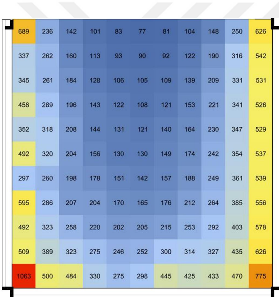
Figure 4.40 Illuminance results in lux of the first floor of the design case 3 on the 8 th of June at 1 pm
