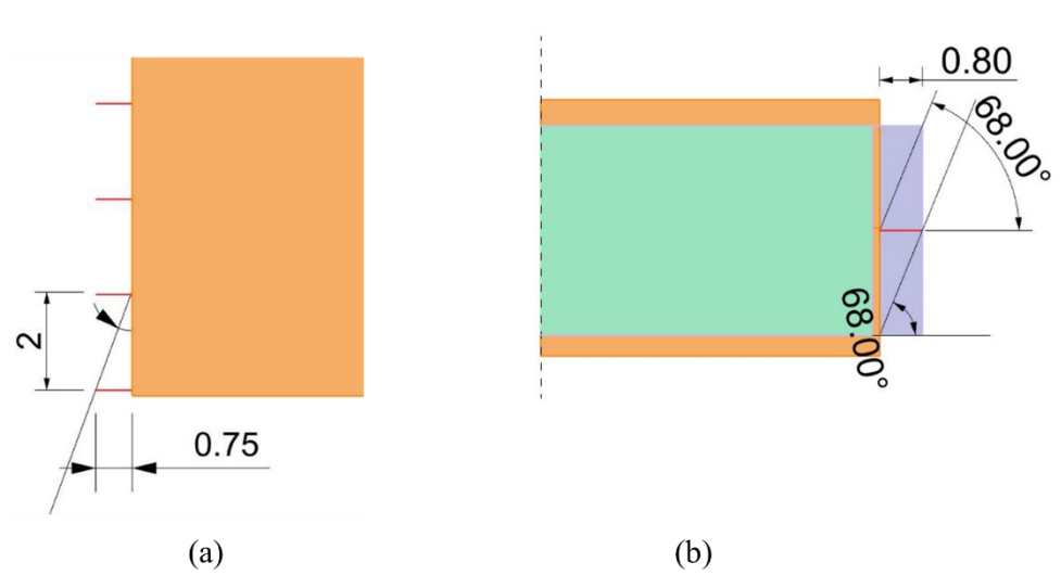
Figure 3.27 Shading calculations of the first floor for the west facade from the plan view (a) and south facade from the section view (b)
