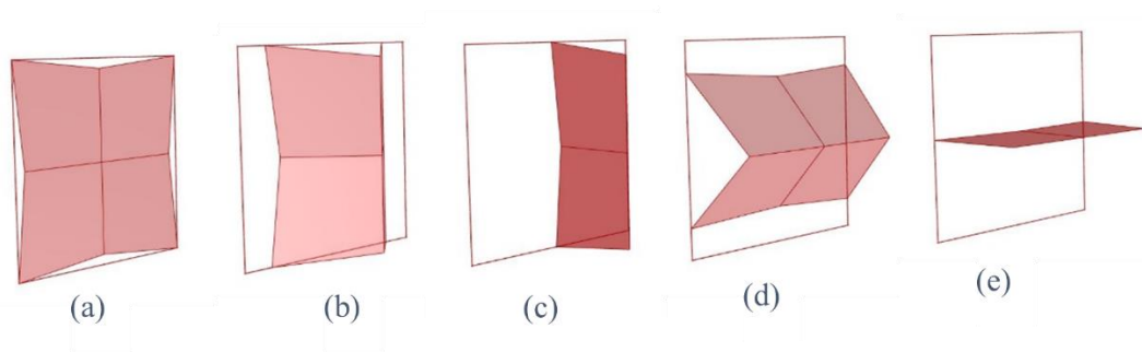
Figure 3.28 Kinetic facade modules adapted from the study of W. T. Sheikh and Asghar (2019) with the options of fully close (a), half-open vertically (b), fully open vertically (c), half-open horizontally (d) and fully open horizontally (e)
