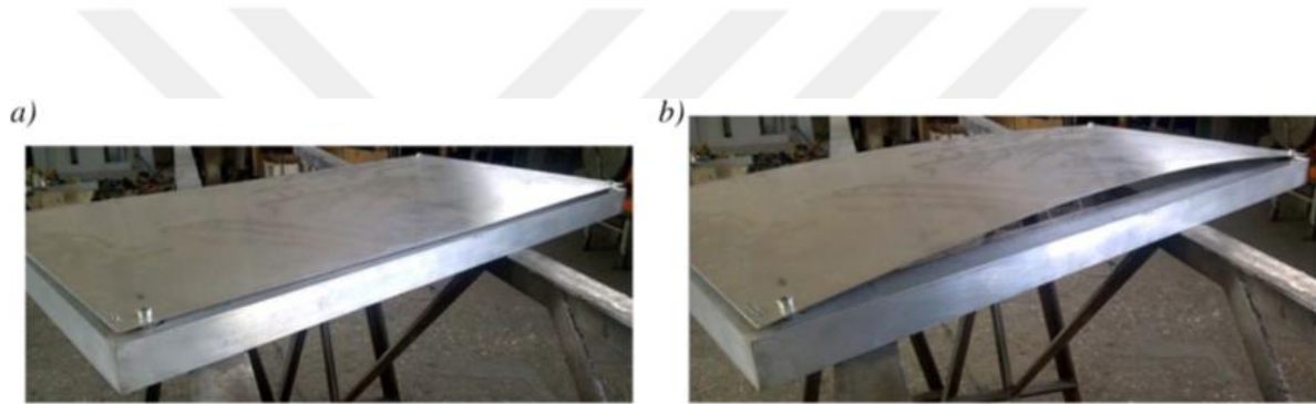
Figure 2.12. Physical model by using aluminum sheets and closed (a) and opened (b) positions (Formentini & Lenci, 2018)
