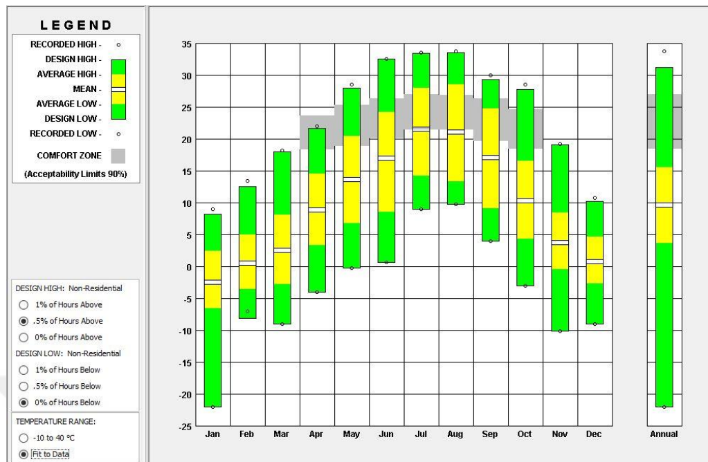
Figure 3.1 Comfort Zone and Temperature Range of Ankara during the year, produced by Climate Consultant 6.0
