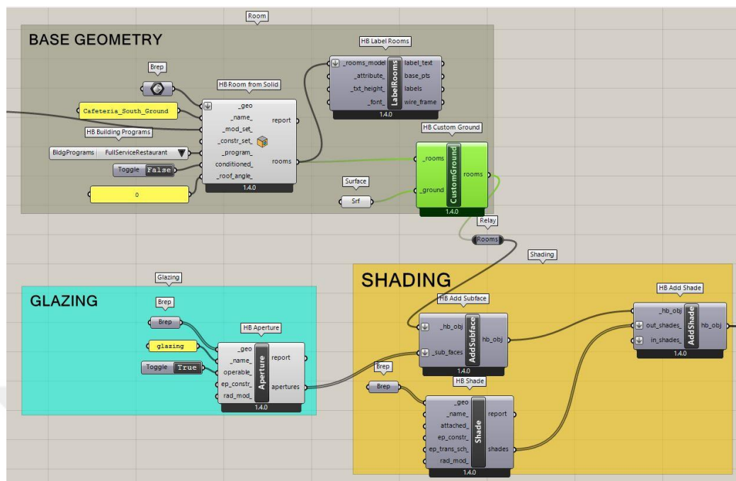
Figure 3.19 Script of the Definition of the Honeybee Model with the rooms, glazing, and shading
