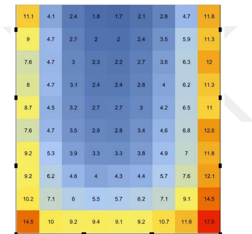
Figure 4.37 Daylight factor results of the ground floor of the design case 3
