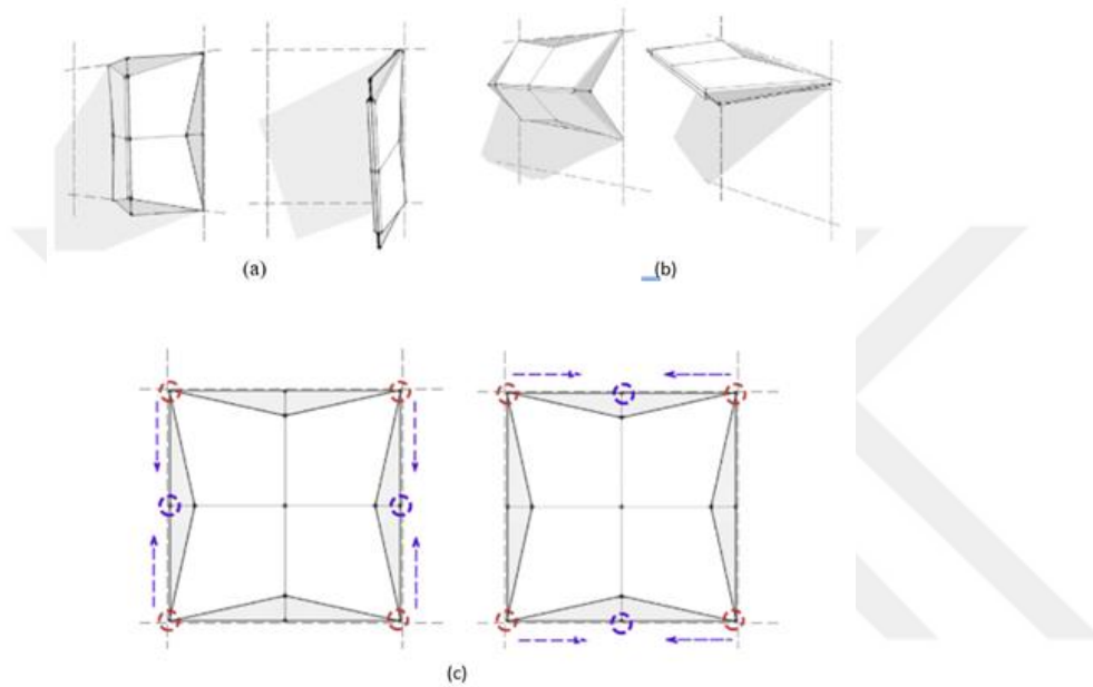
Figure 2.11. Horizontal shading (a), vertical shading (b), and kinematics (c) of Oxalis Oregana-inspired facade morphology (W. T. Sheikh & Asghar, 2019)
