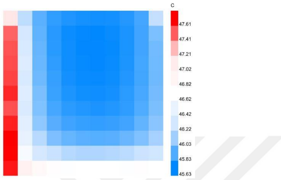
Figure 4.4 Operative Temperature Results of the First Floor of the Base Case on the 30 th of July at between 11 am to 14 pm, in Honeybee
