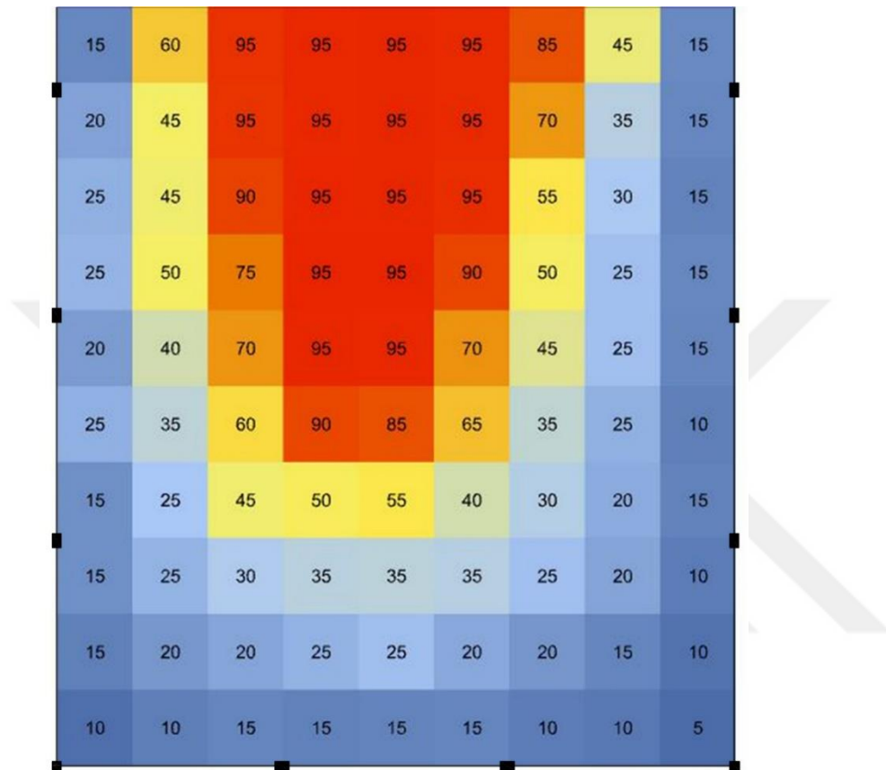
Figure 4.38 UDI results of the ground floor of the design case 3
