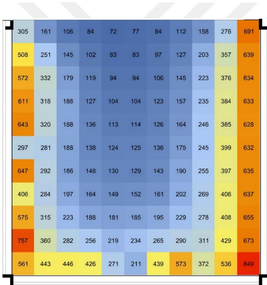
Figure 4.13 Illuminance results in lux of the first floor of the 2x2 modules with metal on the 8 th of June at 1 pm
