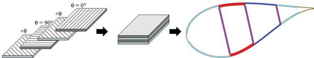
Figure 3.20. The illustration stacking of multiple lamina and the classical lamination theories' effective material used in Co-Blade (reproduced from [60])
