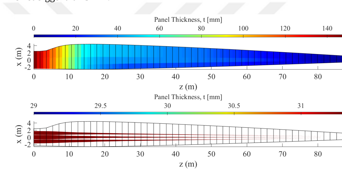
Figure 4.40. Blade shell (up) and shear web (bottom) thickness of the upscaled + optimized NREL 5 at 10 MW
