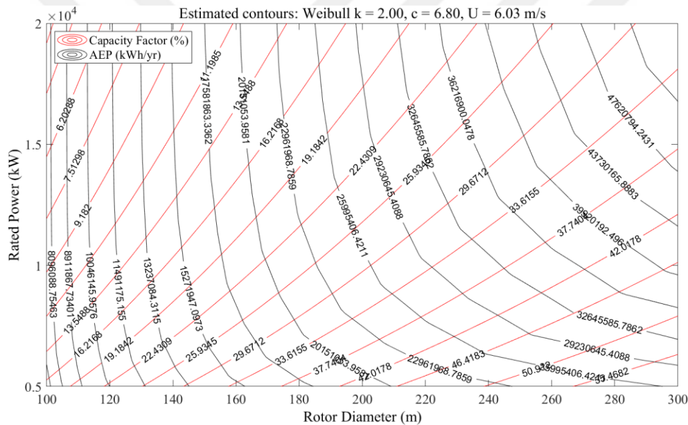
Figure 4.44. Estimated AEP and Capacity factor for various rotor sizes and rated power ranges.
