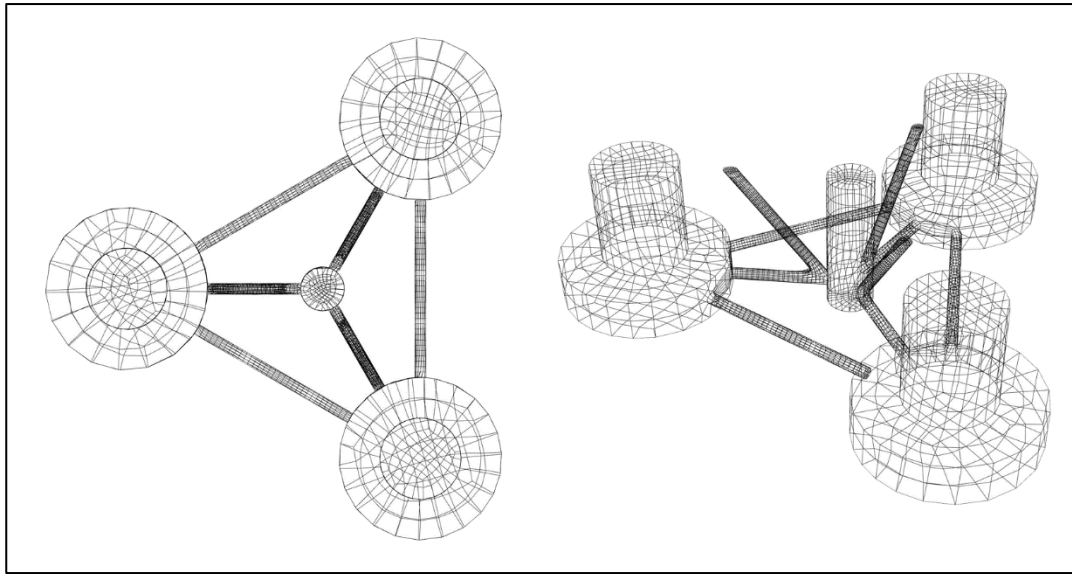
Figure 4.26. Example of .gdf meshing before transformed in HAMS'
