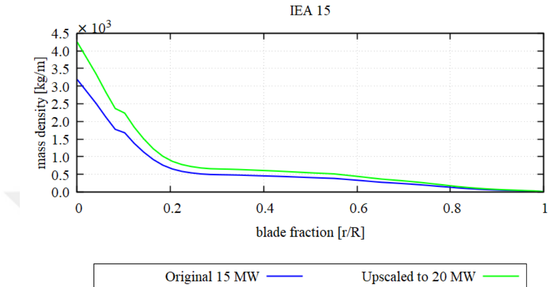
Figure 4.20. Blade mass density distribution of IEA 15 and its upscaled blade up to 20 MW
