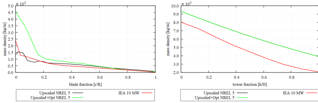
Figure 5.23. Blade and tower's mass density distribution of 10 MW rated power of upscaled NREL 5, upscaled + optimized NREL 5, and IEA 10
