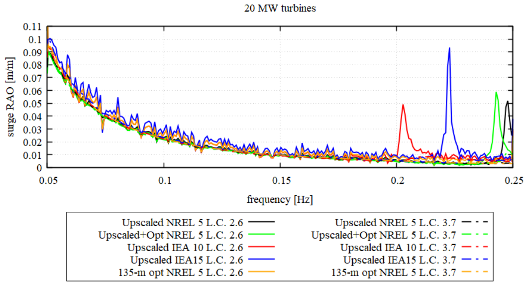
Figure 5.53. Surge RAO of 20 MW upscaled NREL 5, upscaled + optimized NREL 5, upscaled IEA 10, upscaled IEA 15, and 135 meters optimized NREL 5
