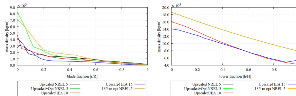
Figure 5.51. Blade & tower's mass density of 20 MW upscaled NREL 5, upscaled + optimized NREL 5, upscaled IEA10, upscaled IEA15, 135m optimized NREL5
