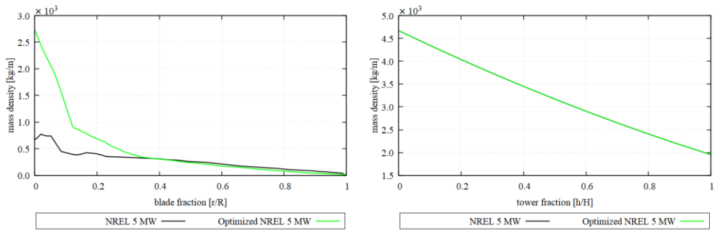
Figure 5.9. Blade and tower's mass density distribution of 5 MW rated power of NREL 5 and Optimized NREL 5 MW
