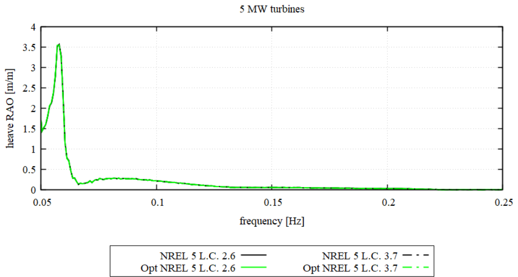
Figure 5.13. Heave RAO of NREL 5 MW and Optimized NREL 5 MW
