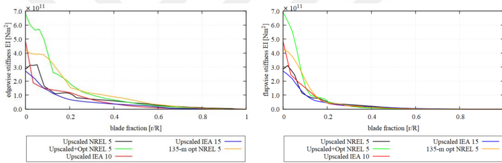
Figure 5.50. Edgewise-flapwise stiffness of 20 MW upscaled NREL 5, upscaled + optimized NREL 5, upscaled IEA 10, upscaled IEA 15, 135m optimized NREL5
