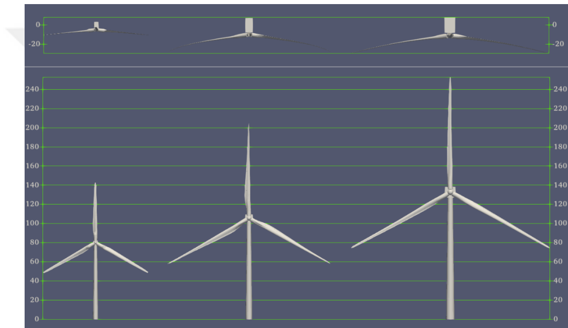
Figure 3.7. NREL 5 MW, IEA 10 MW, and IEA 15 MW Reference Wind Turbines
