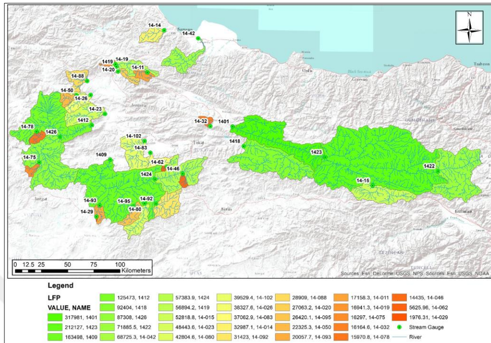
Figure 6.12. Distribution of Longest Flow Path Across Study Catchments
