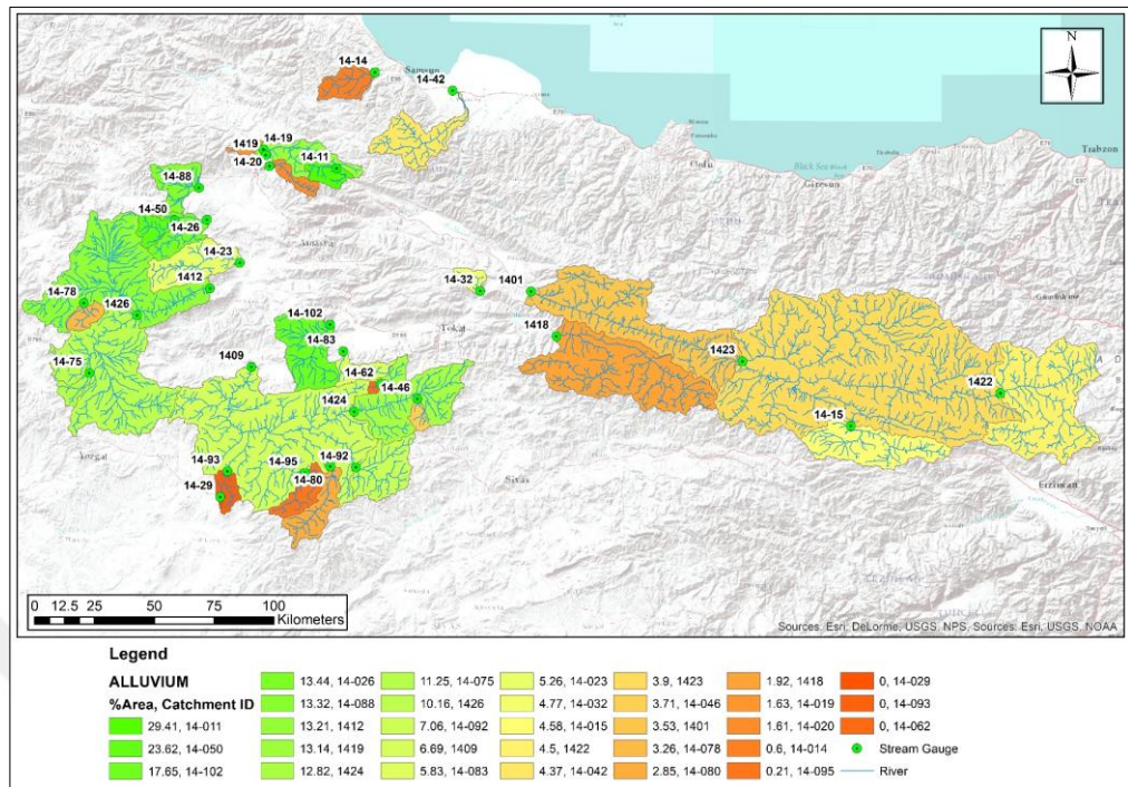
Figure 6.1. Alluvium (%) Distribution Across Study Catchments.
