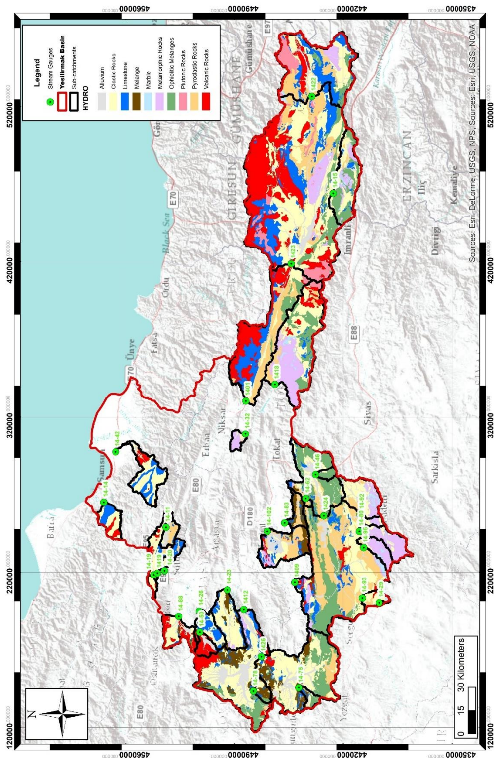
Figure 4.4. Geology of Study Catchments.
