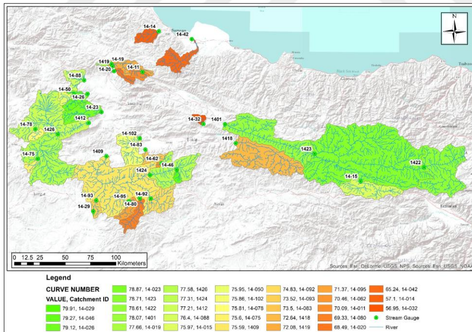
Figure 6.8. Runoff Curve Number Distribution Across Study Catchments
