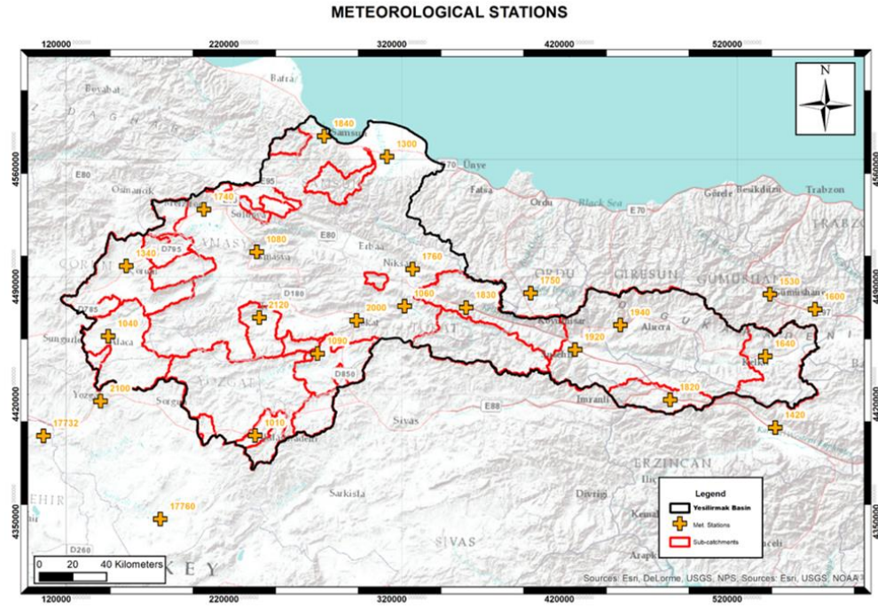
Figure 2.7. Meteorological Stations Meteorological Stations for Potential Evapotranspiration
