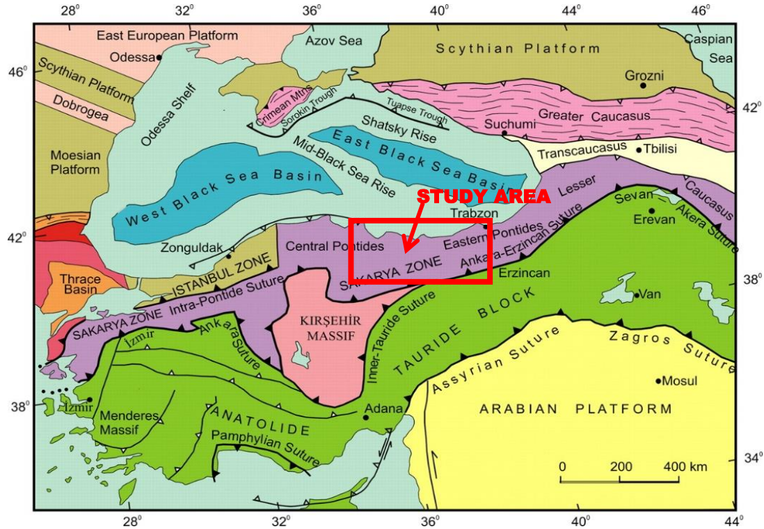
Figure 4.1. Tectonic map of northeastern mediterranean region showing the major sutures and continental blocks. Sutures are shown by heavy lines with the polarity of former subduction zones indicated by filled triangles. Heavy lines with open triangles represent active subduction zones (Okay and Tüysüz, 1999).
