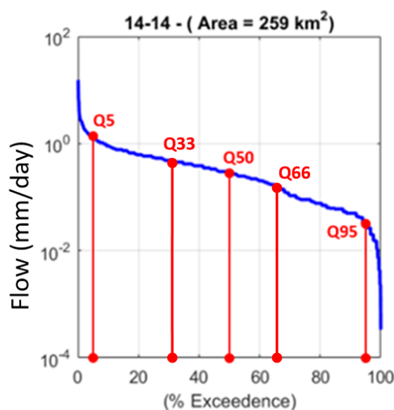
Figure 5.1. Example of Flow Duration Curve for Catchment 14-14
