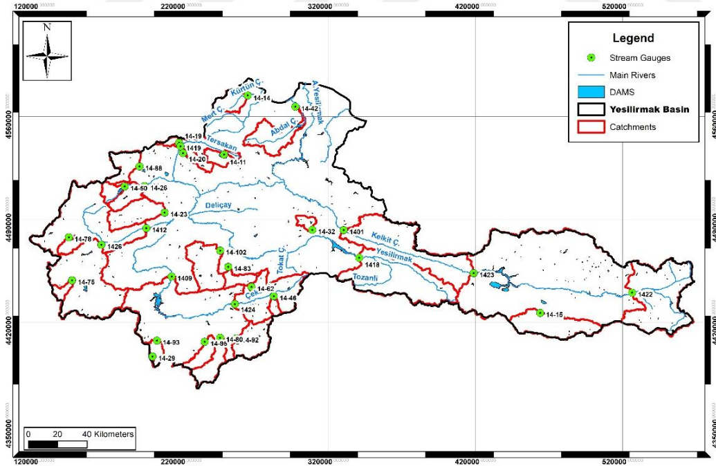
Figure 1.5. Dams in Yeşilirmak Basin
