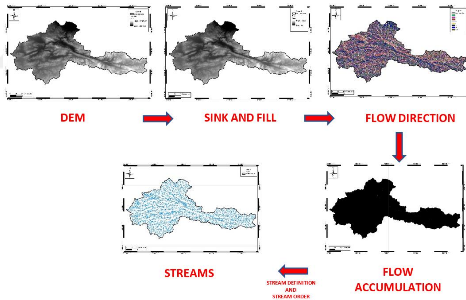
Figure 1.6. Stream Extraction from Digital Elevation Model
