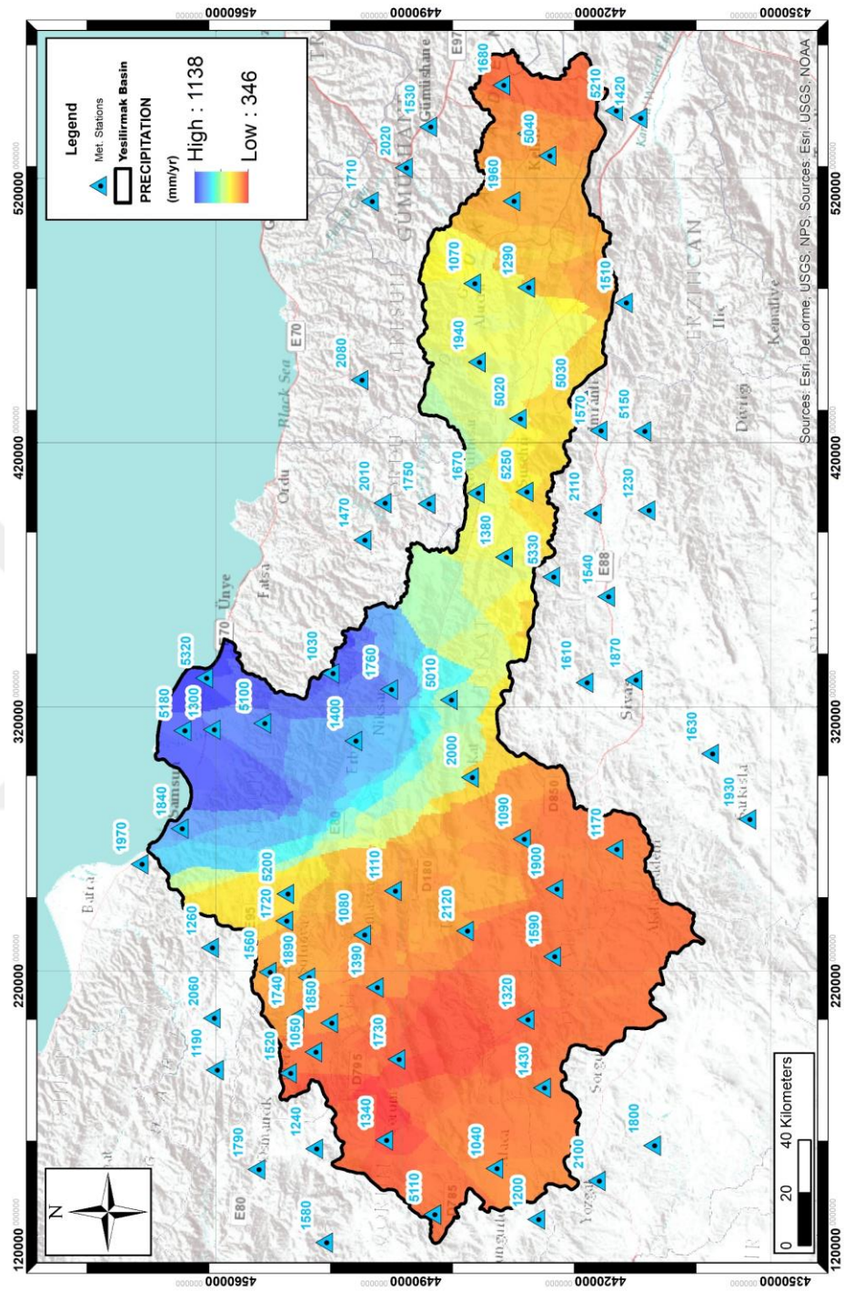
Figure 2.2. Mean Annual Precipitation of Yeşilirmak Basin
