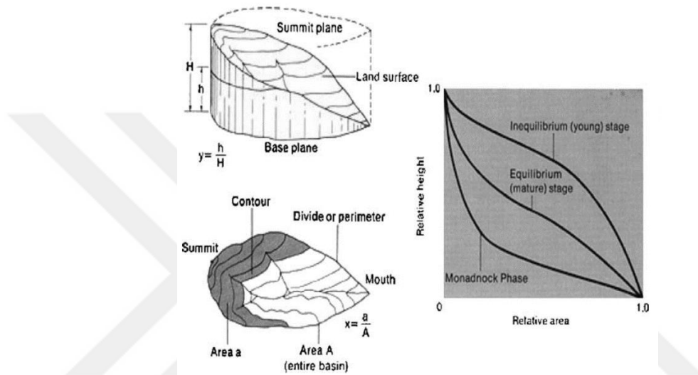
Figure 6.10. Hypsometry Curve and Hypsometry Integral Concept (Ritter et al. 2002)
