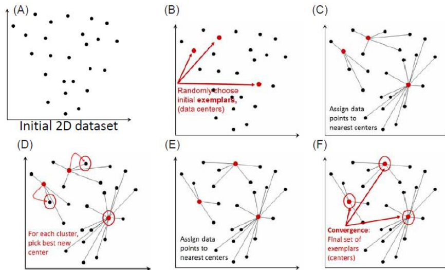
Figure 7.1. K-Means Clustering Algorithm Scheme (Dueck, 2009)
