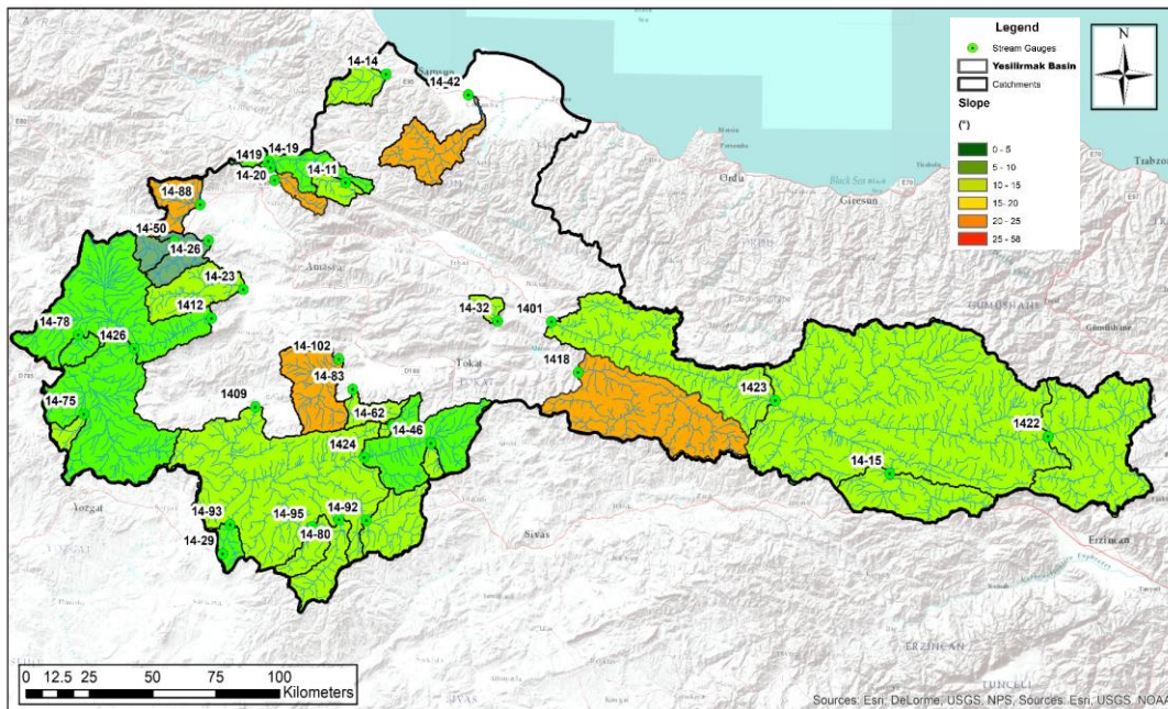
Figure 6.17. Slope Map of Study Catchments
