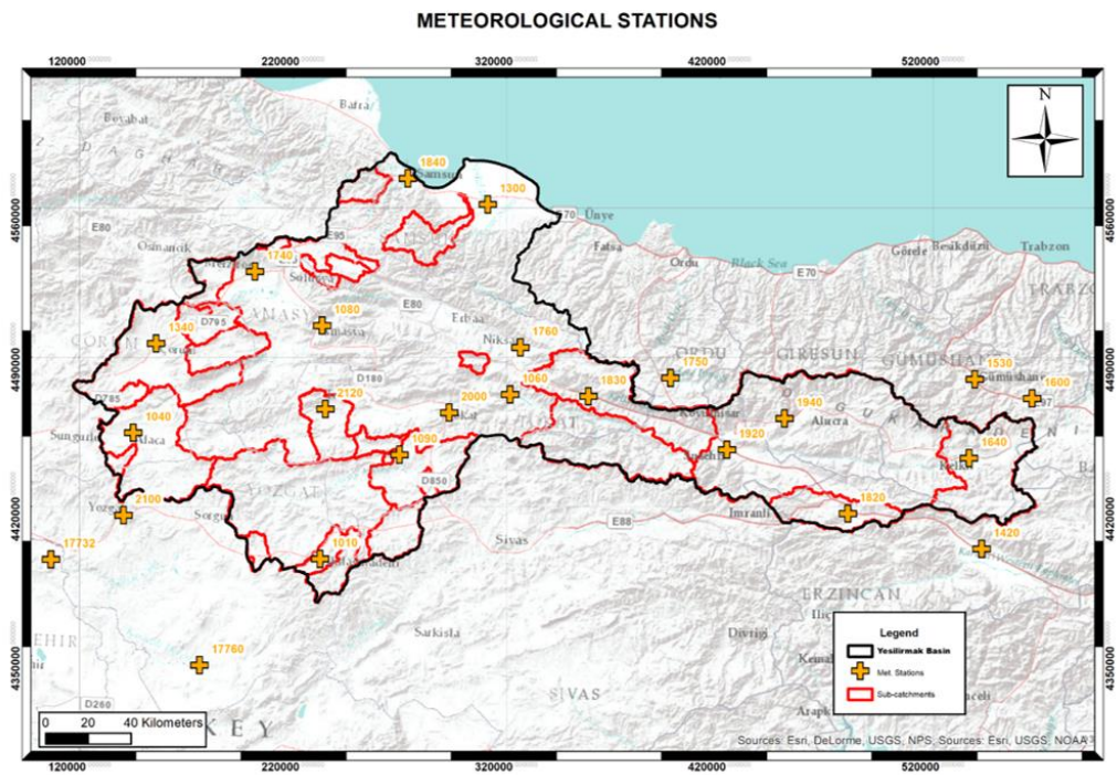
Figure 2.4. Meteorological Stations for Temperature
