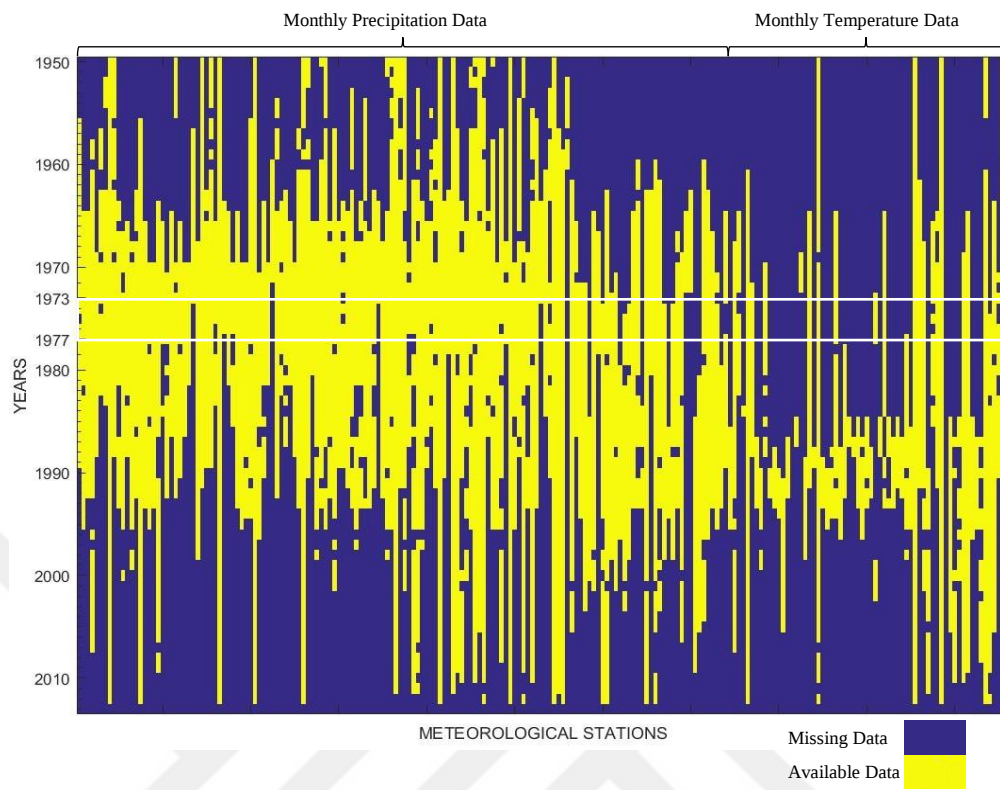
Figure 1.4. Available Meteorological Data
