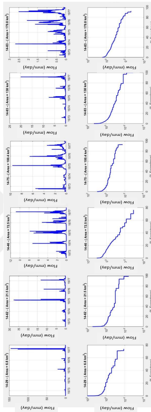
Figure 3.6. Hydrographs and Flow Duration Curves of Catchments Located at the South of Basin
