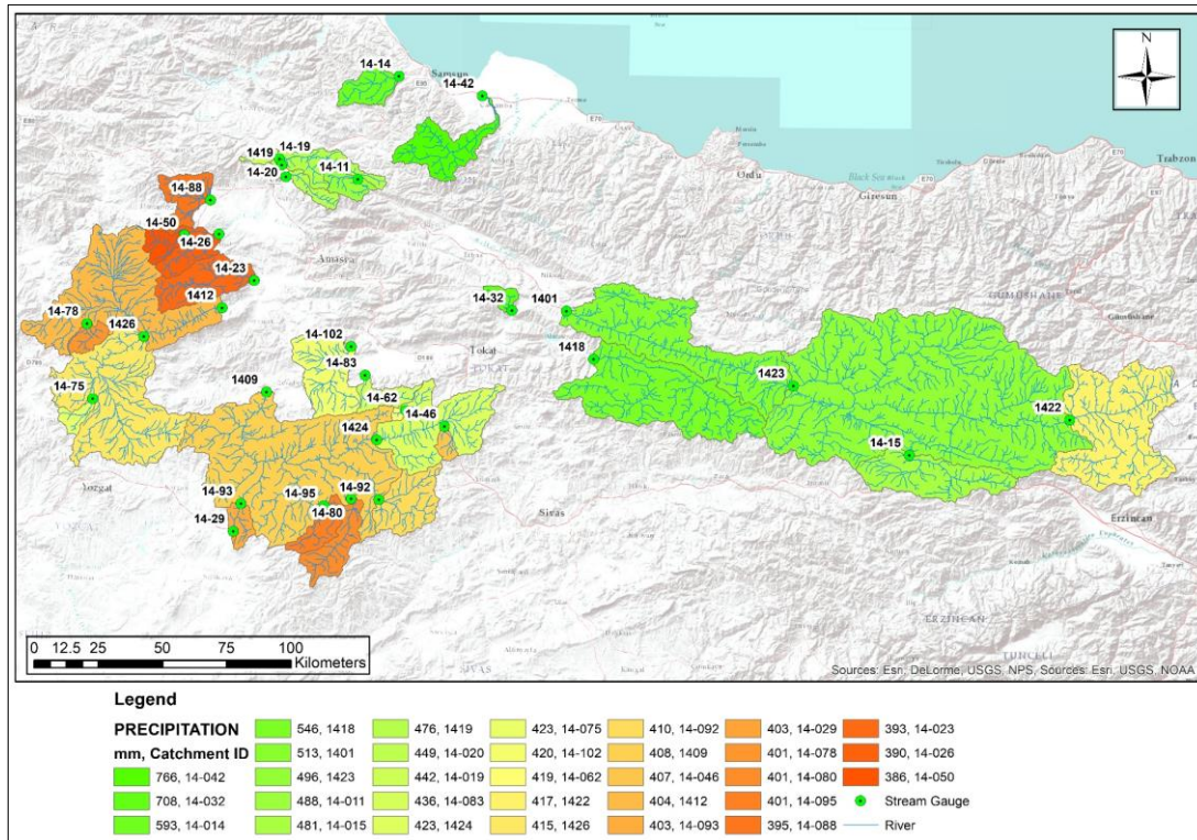
Figure 6.18. Precipitation Distribution Across Study Catchments
