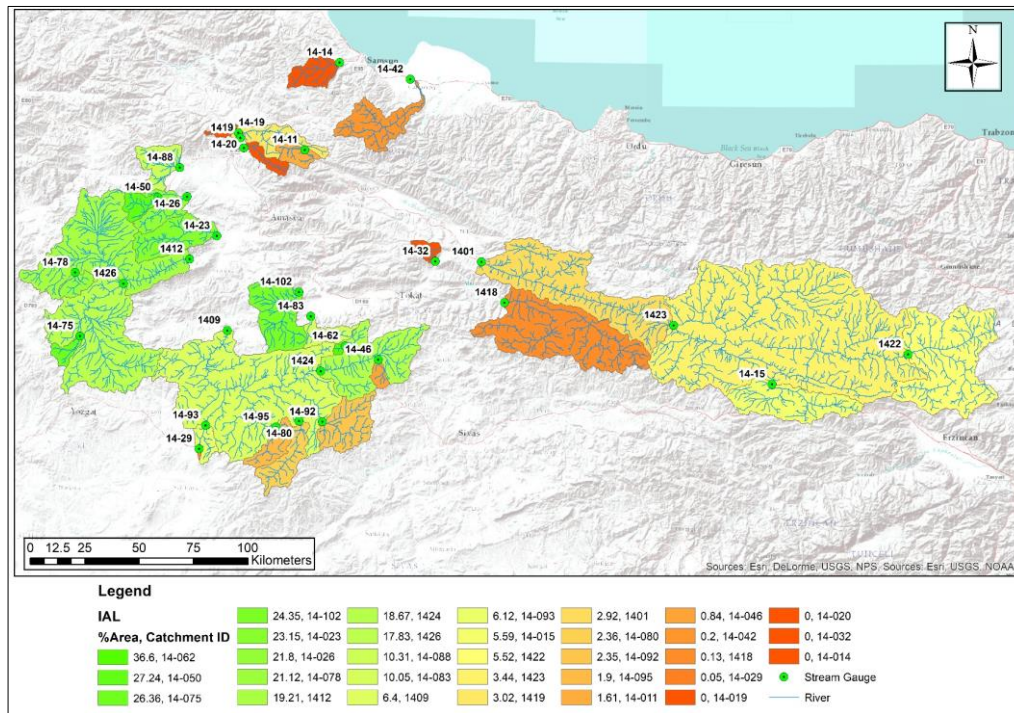
Figure 6.9. Irrigated Arable Lands Distribution Across Study Catchments
