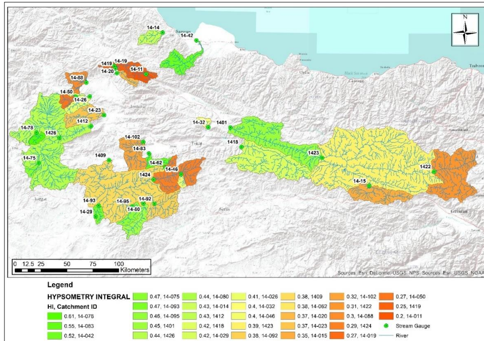
Figure 6.11. Hypsometry Integral Distribution Across Study Catchments
