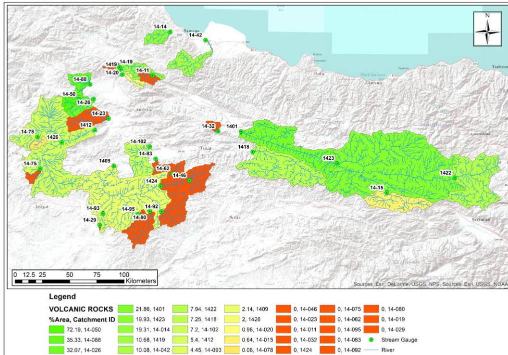
Figure 6.3. Volcanic Rocks (%) Distribution Across Study Catchments.
