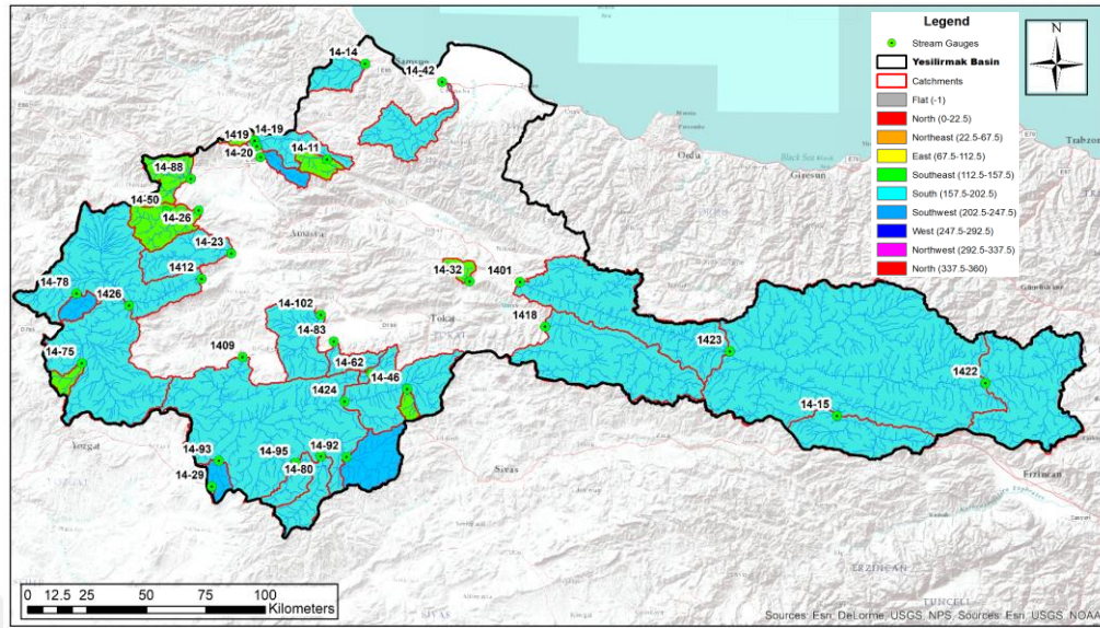
Figure 6.16. Aspect Map of Study Catchments
