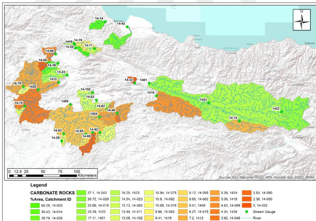
Figure 6.2. Carbonate Rocks (%) Distribution Across Study Catchments.
