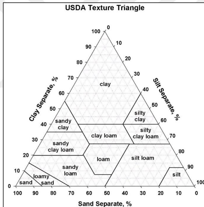
Figure 6.7. USDA Texture Triangle (USDA, 1986)
