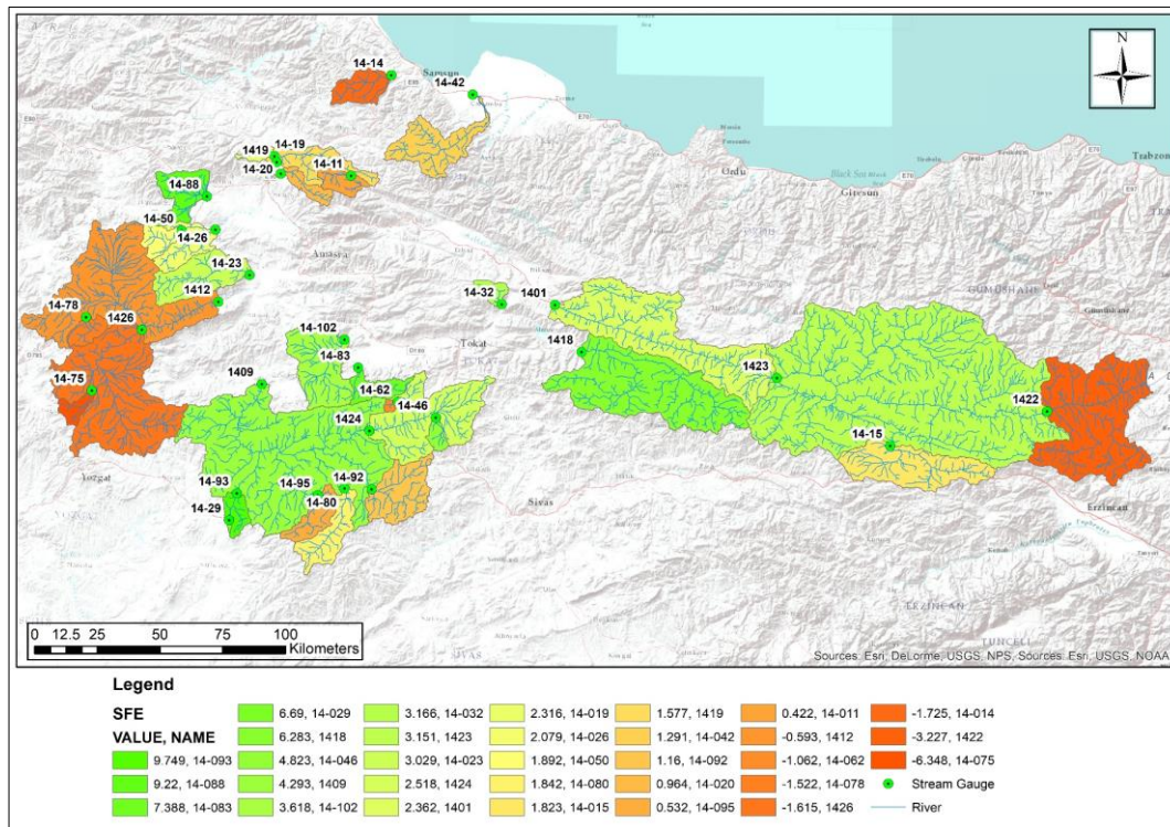
Figure 5.8 Streamflow Elasticity Distribution Across Study Catchments
