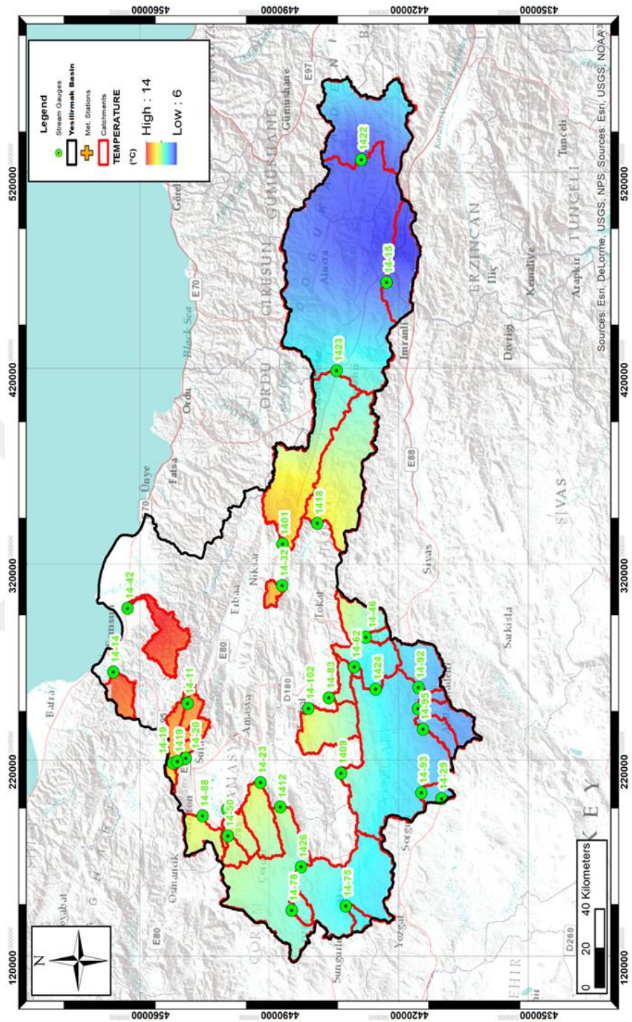
Figure 2.6. Mean Annual Temperature of Study Catchments
