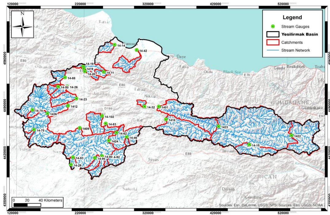
Figure 1.2. Studied Catchments in Yeşilirmak Basin
