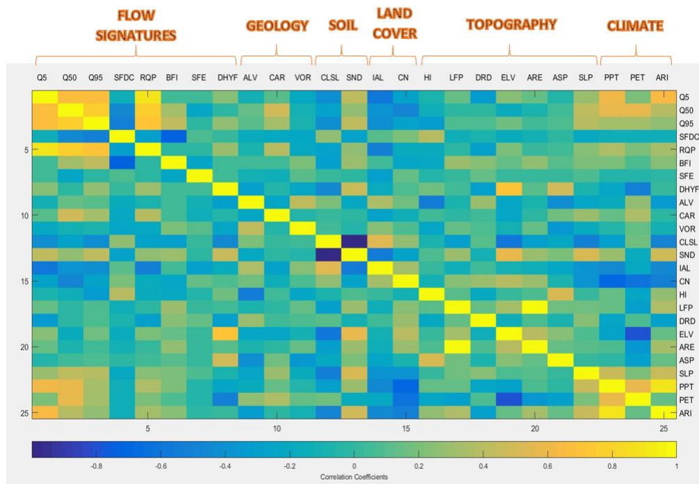
Figure 8.2. Signature Relationship Matrix (see Table 8.1 for abbreviations).
