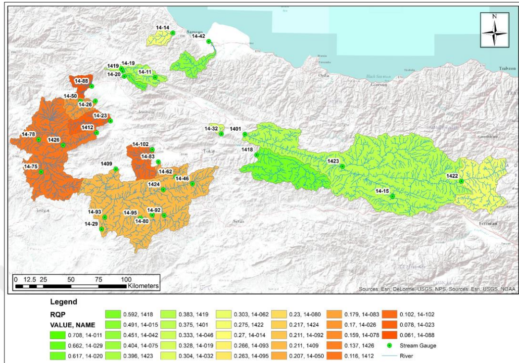
Figure 5.6 Runoff Ratio Distribution Across Study Catchments
