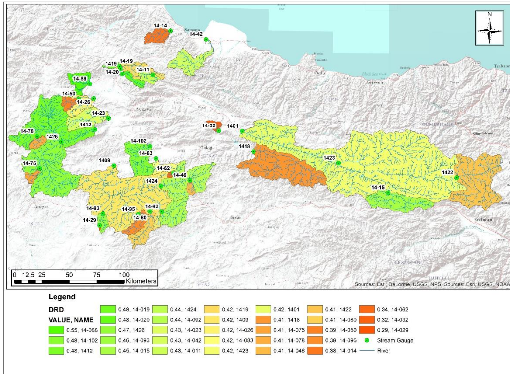
Figure 6.13. Drainage Density Distribution Across Study Catchments
