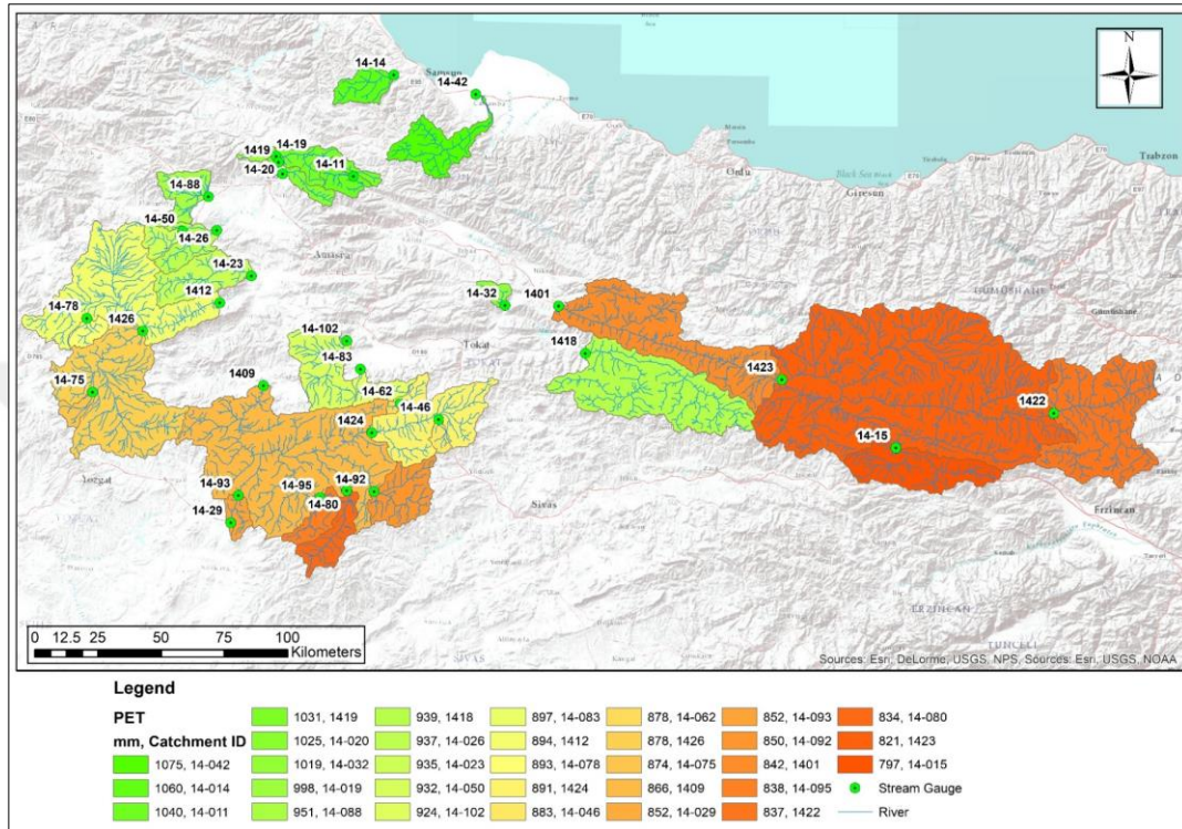
Figure 6.19. Potential Evapotranspiration Distribution Across Study Catchments
