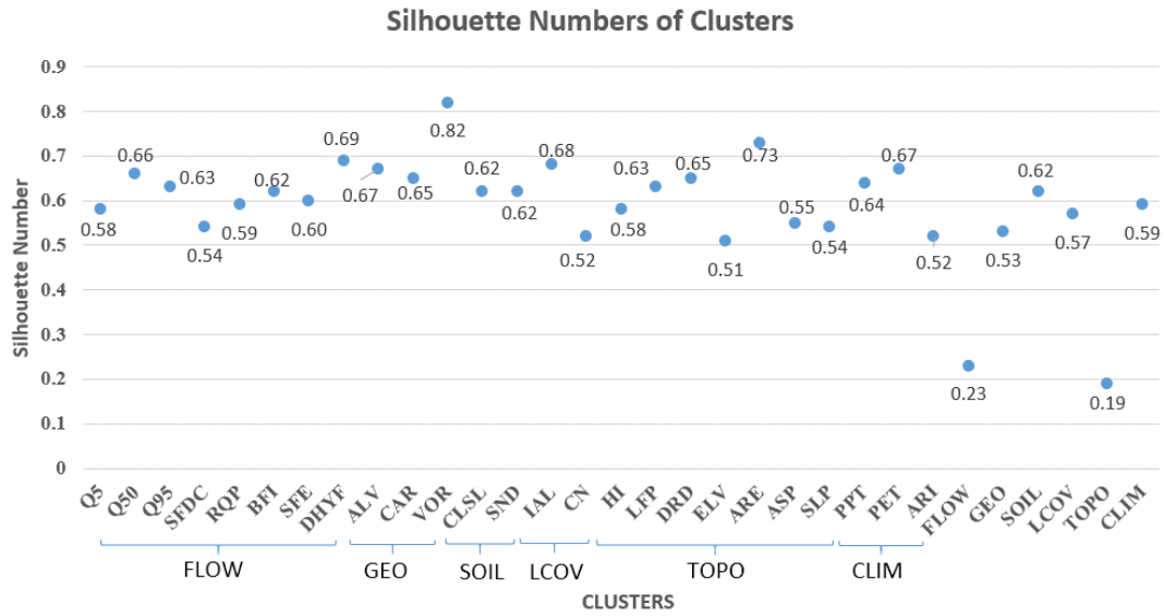
Figure 8.1. Silhouette Numbers of Clusters (see Table 8.1 for abbreviations).
