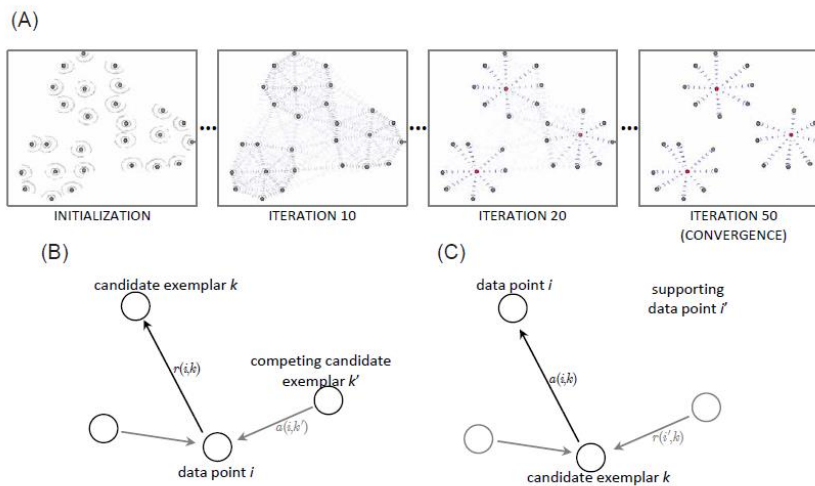
Figure 7.2. Affinity Propagation Clustering Algorithm Scheme (Dueck, 2009)
