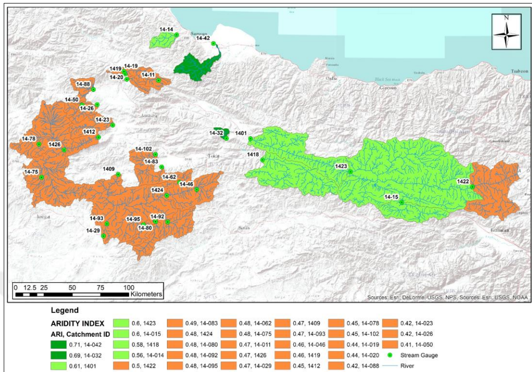
Figure 6.20. Aridity Index Distribution Across Study Catchments
