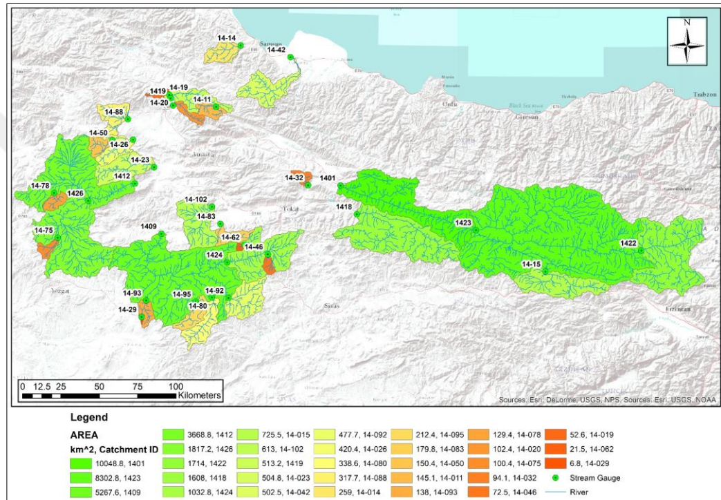
Figure 6.15. Area Distributions of Study Catchments
