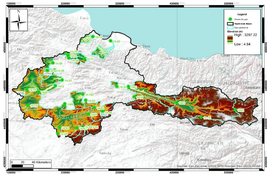
Figure 6.14. Elevation Distribution Across Study Catchments
