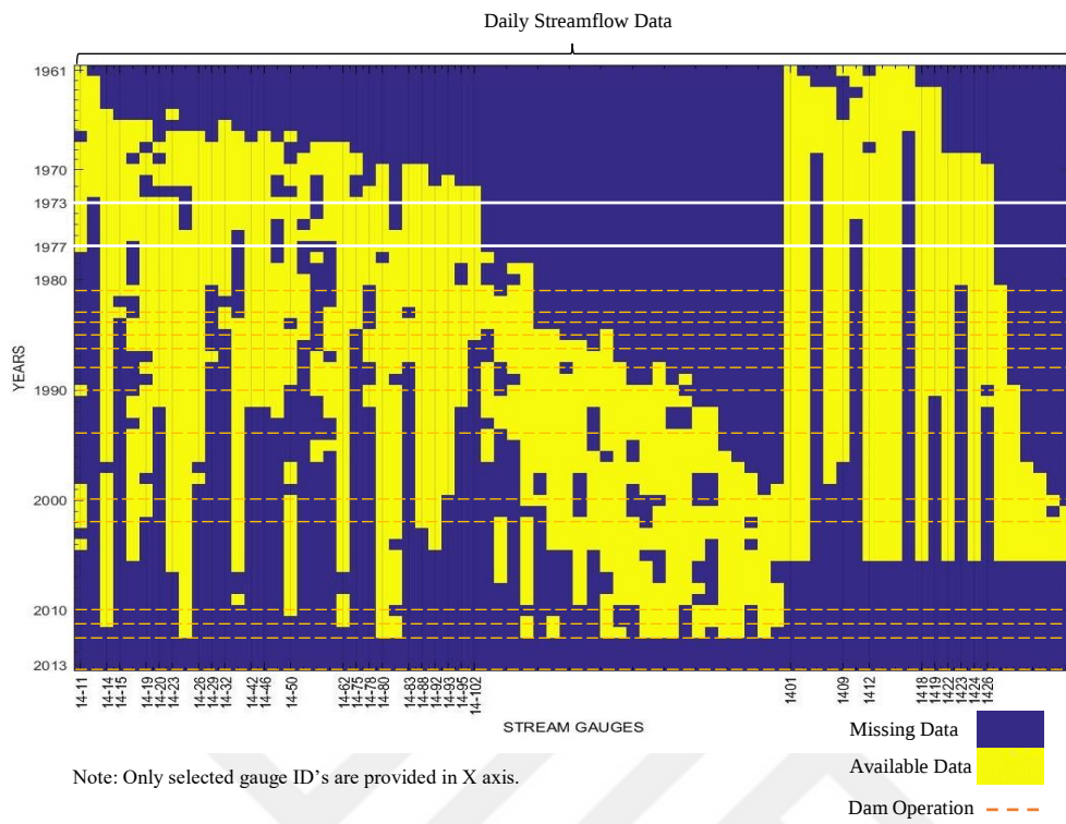
Figure 1.3. Available Streamflow Data
