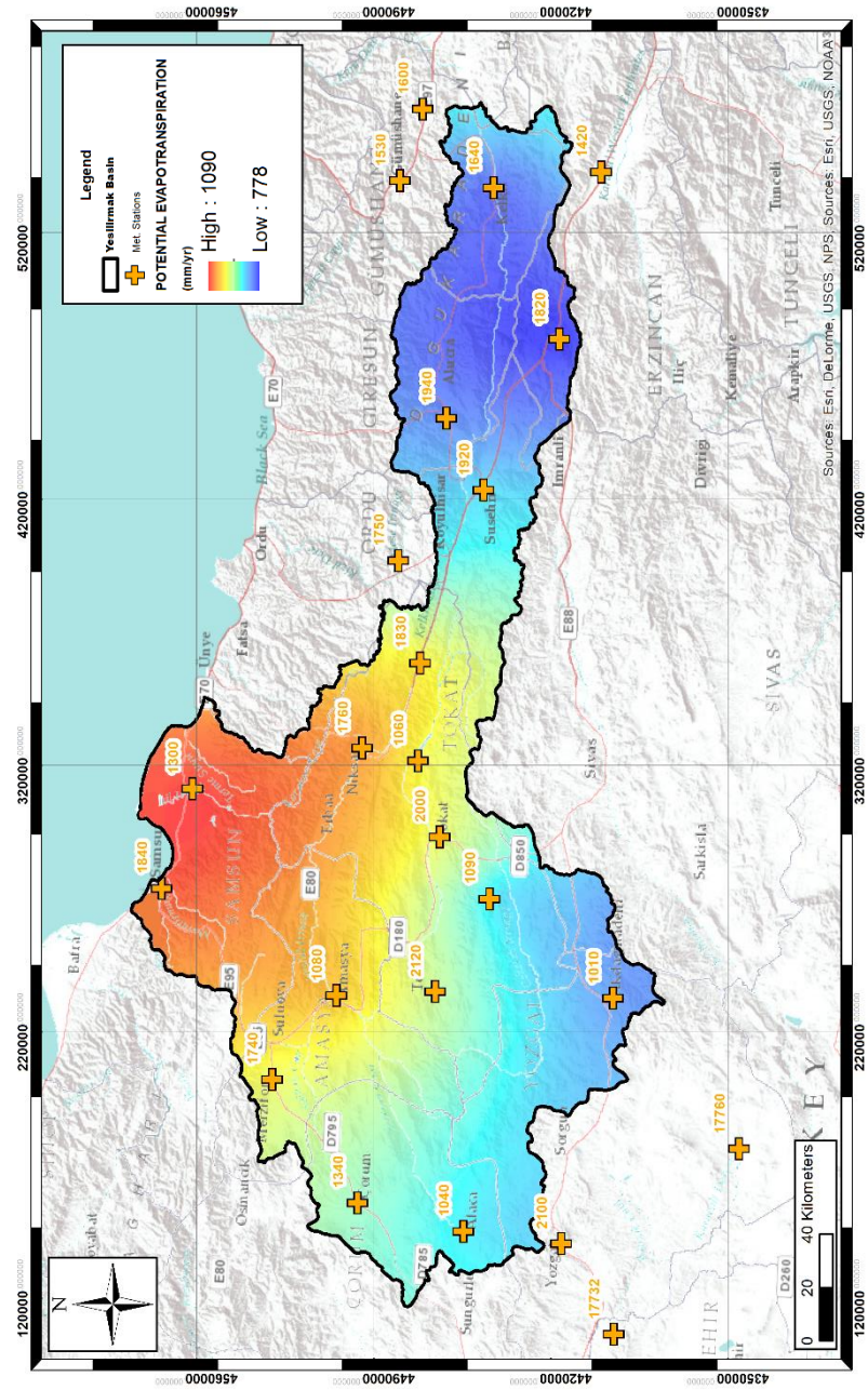
Figure 2.8. Potential Evapotranspiration in Yeşilirmak Basin
