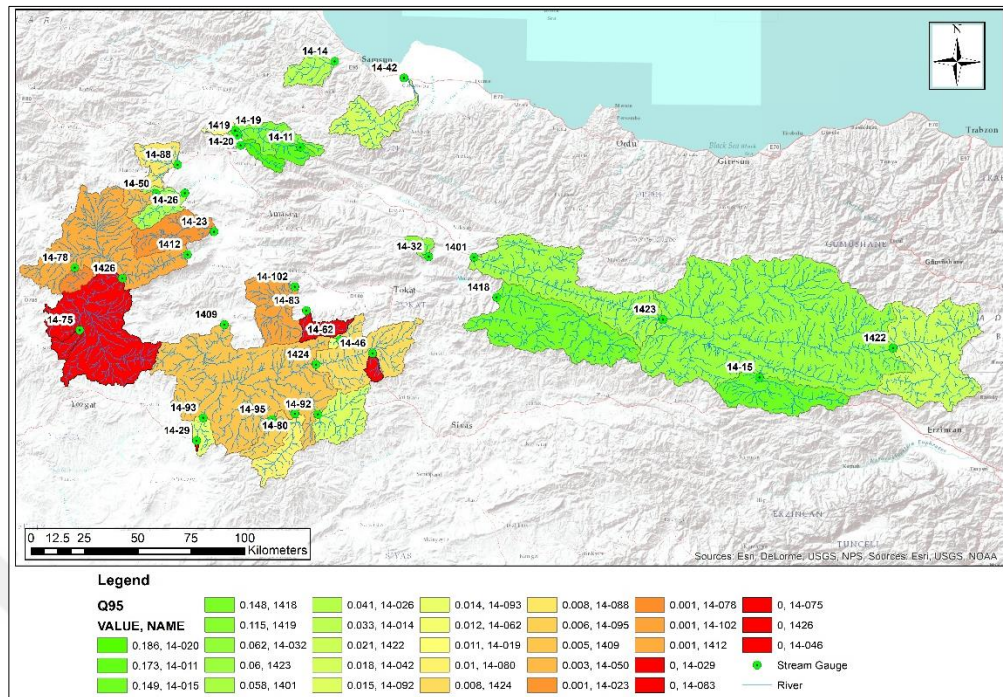
Figure 5.4 Q95 Distribution Across Study Catchments
