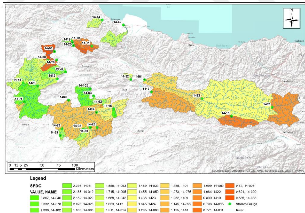
Figure 5.5 Slope of Flow Duration Curve Distribution Across Study Catchments
