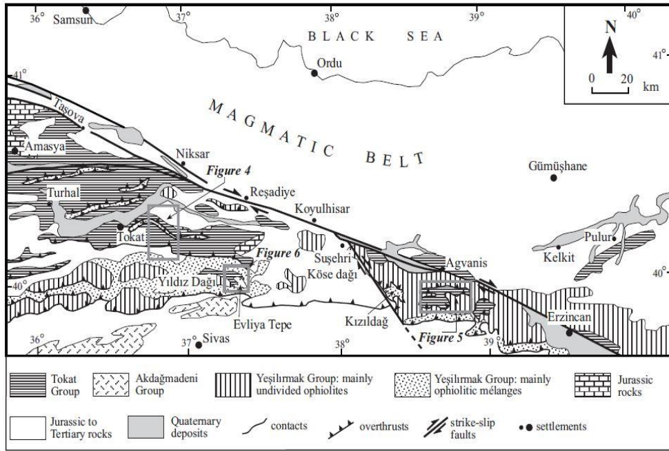
Figure 4.2. Simplified geological maps of the area between Tokat, Sivas and Erzincan (after Yilmaz 1980, 1982b; Özcan et al. 1980; Özcan and Aksay 1996; Yilmaz, 2004)
