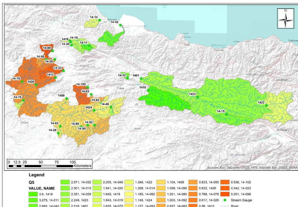
Figure 5.2. Q5 Distribution Across Study Catchments
