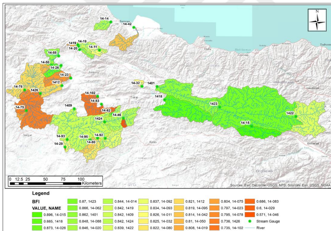
Figure 5.7 Baseflow Index Distribution Across Study Catchments
