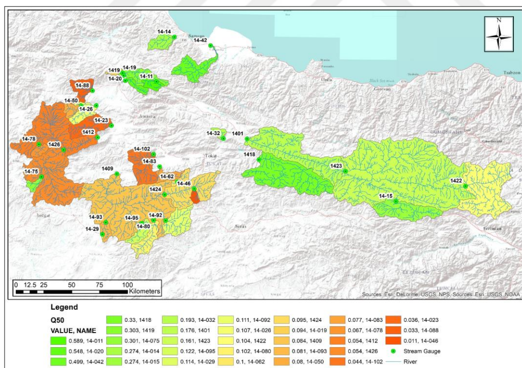
Figure 5.3 Q50 Distribution Across Study Catchments
