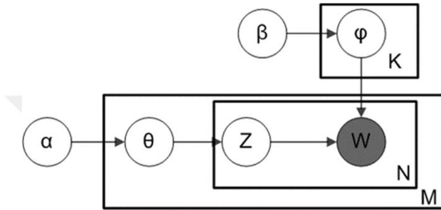
Figure 2.5. The Plate Diagram of LDA M is number of documents, N is the number words, K is number of topics 46 .
