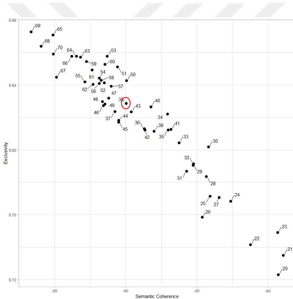
Figure 4.2. Semantic Coherence – Exclusivity score dispersion for topic models with number of topics from 20 to 70. Selected topic model with 38 topics is encircled with red.
