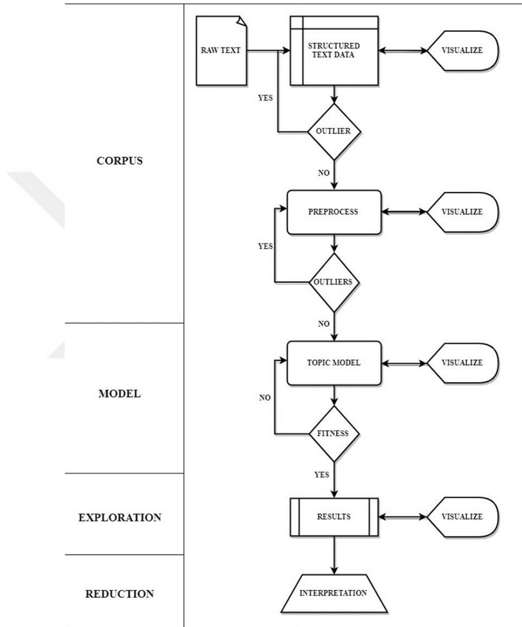
Figure 1.3. Layout of Methodology
