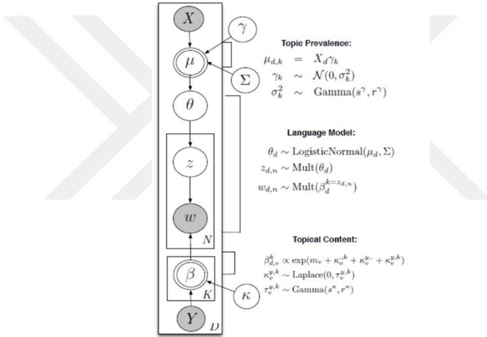
Figure 2.6. . Plate Diagram for the Structural Topic Model.
