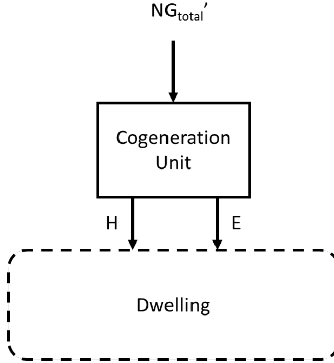
Figure C.3. Power and heat supply schematics for Projection 7
