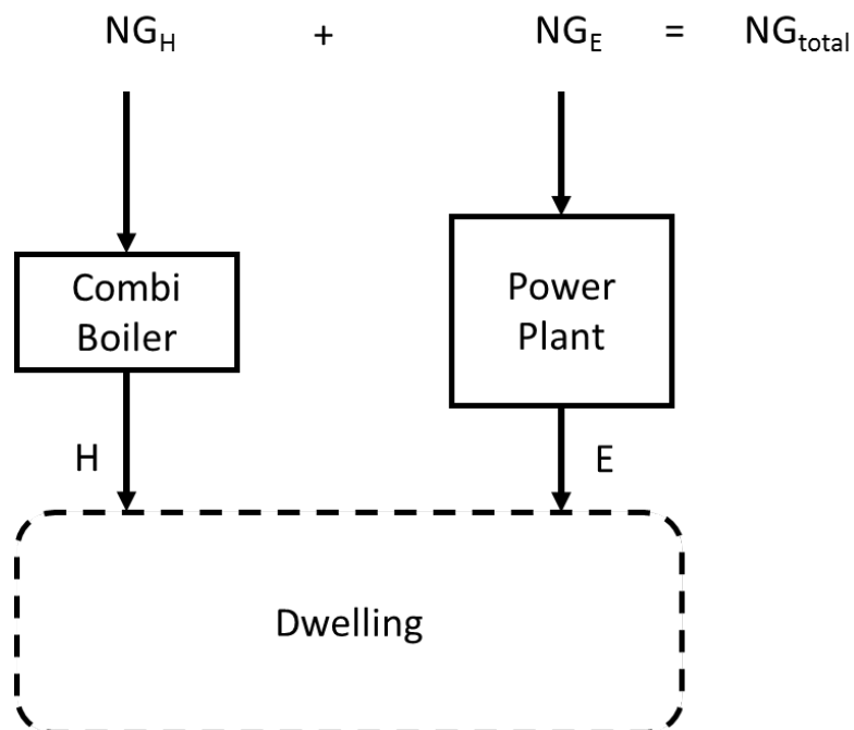
Figure C.2. Power and heat supply schematics for Projections 1-6
