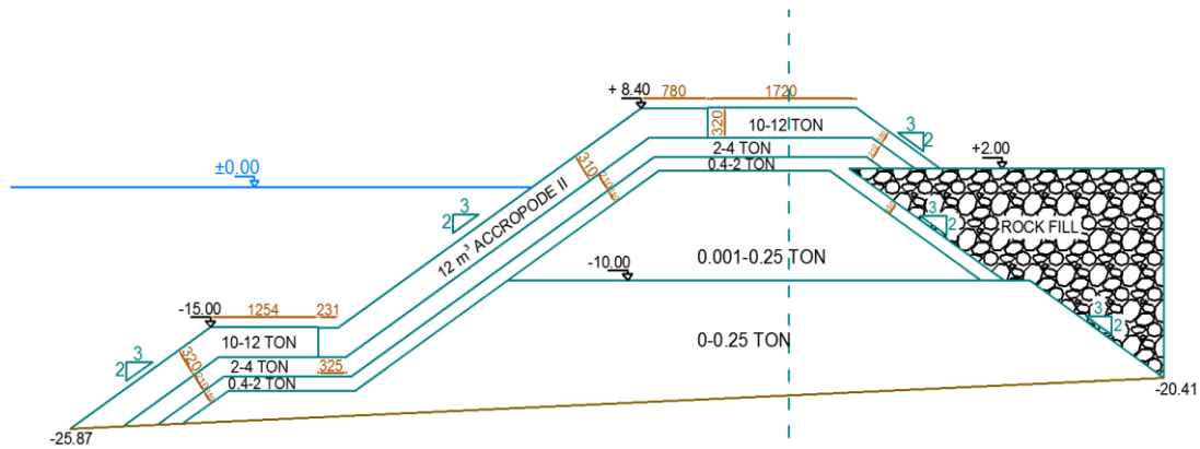
Figure 6.27 Cross-section of Accropode™ II Alt-2
