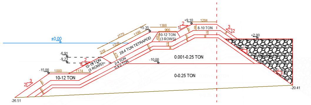
Figure 6.5 Cross-section of Rock-Alt-2
