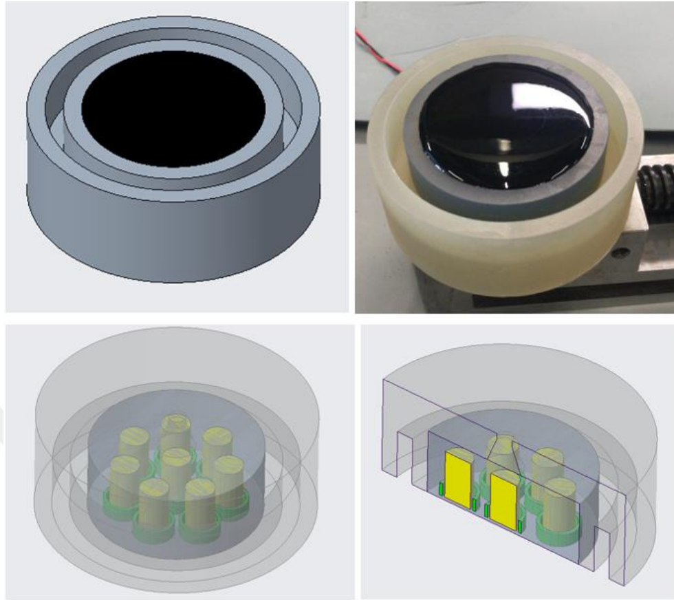
Figure 2.50 Sensor
