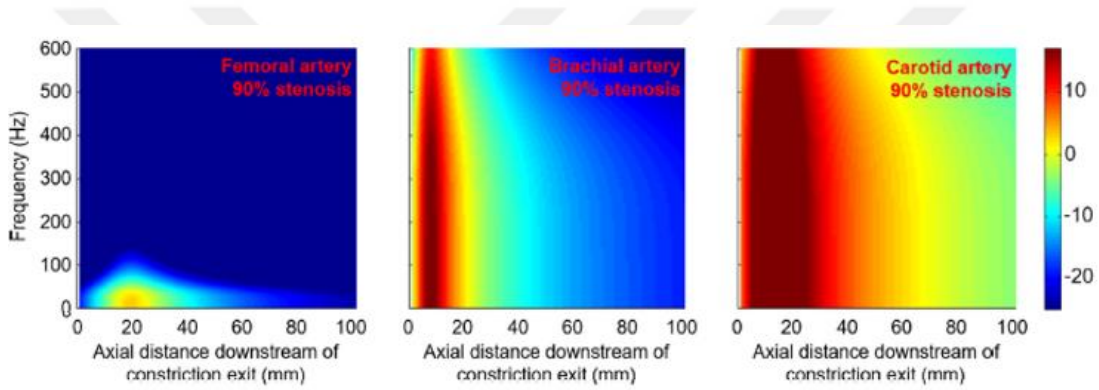
Figure 2.4 Acoustic pressure (dB reference: 1 Pa) fields as a function of axial position and frequency. Pressure fields are obtained at peak blood flow rates for 90% stenosis in the femoral, brachial, and common carotid arteries. [32]
