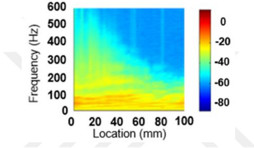
Figure 2.1 Empirical result for radial velocity (dB Reference 1 Mm/S) On Phantom. [52]
