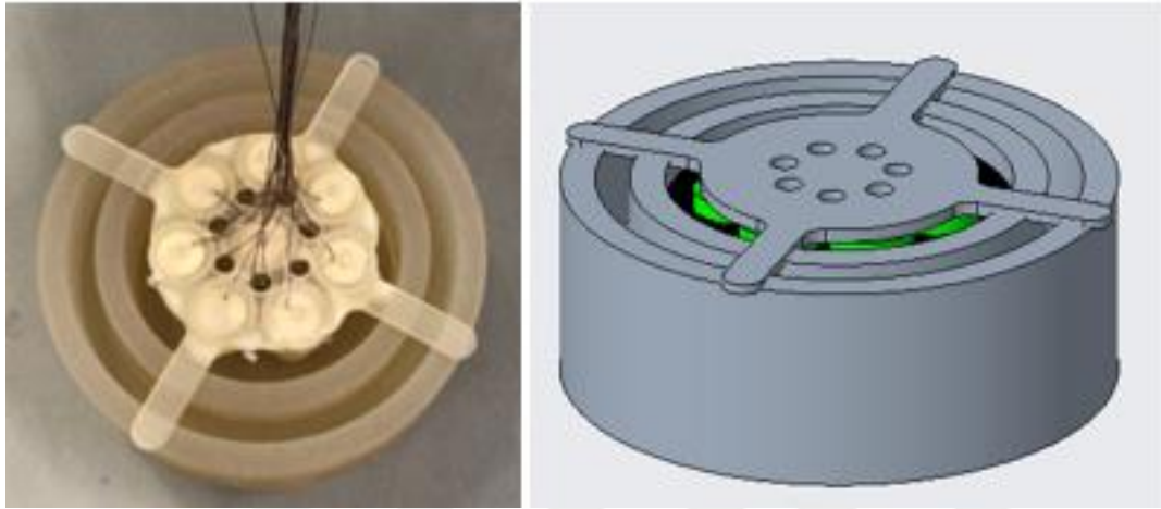
Figure 2.47 Positioning of ceramics before the first step of polyurethane filling
