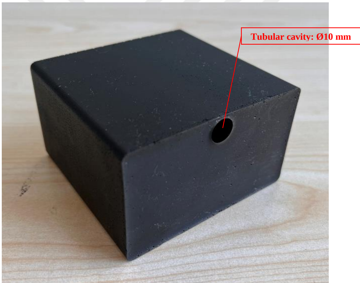
Figure 3.2 Tissue model
