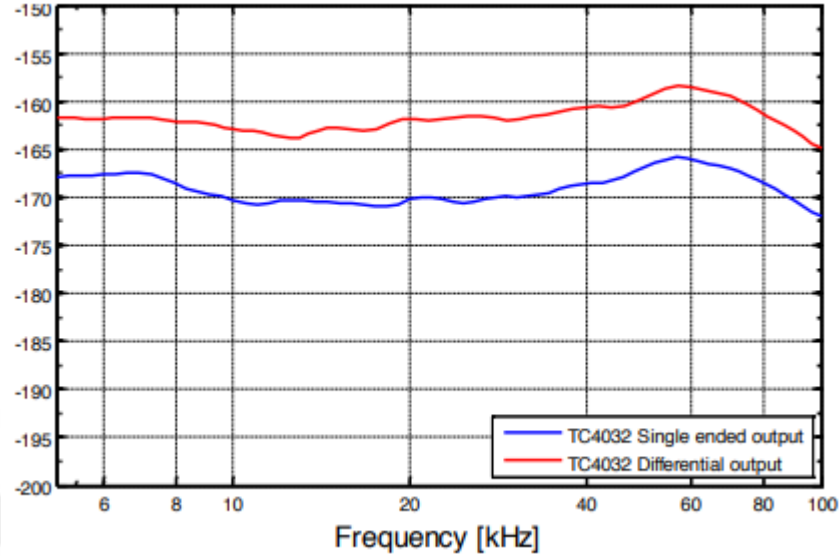
Figure 2.6 Receiving sensitivity of TC 4032 [dB re 1V/ \mu Pa @ 1m][60]
