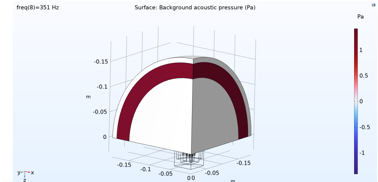
Figure 2.31 Background Pressure Field section where the acoustic pressure is defined in the pressure acoustic section in front of the sensor.
