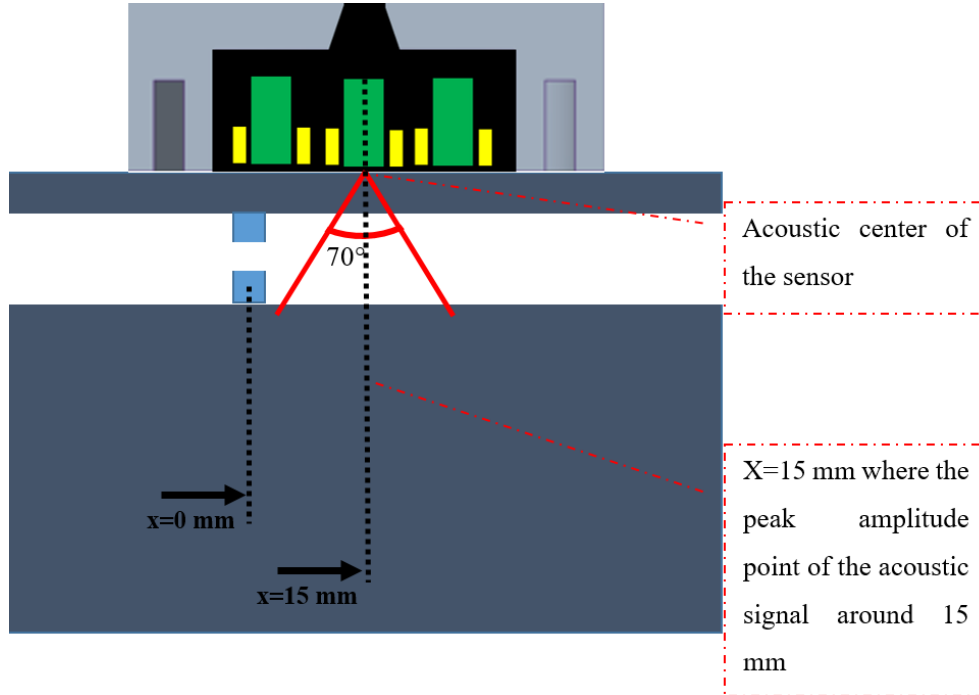
Figure 4.11 The orientation of the test setup where the sensor is centered at x=15 mm
