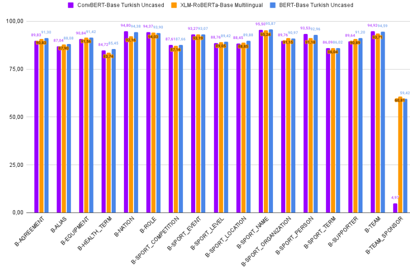
Figure 4.14: Label-wise F1-Scores of ConBERT-Base Turkish Uncased, XLM-RoBERTa-Base Multilingual Model and BERT-Base Turkish Uncased on TurkishSportsNER-Parent-BIO data set
