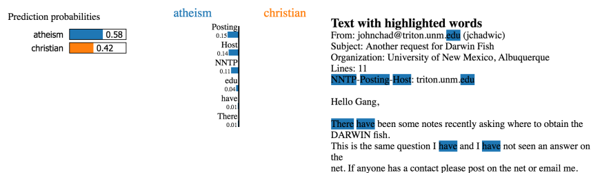
Figure 3.6: Explanation example of a text classification by LIME. Sourced by [3]
