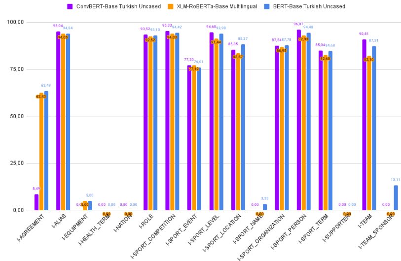
Figure 4.13: Label-wise Recall Values of ConBERT-Base Turkish Uncased, XLM-RoBERTa-Base Multilingual Model and BERT-Base Turkish Uncased on TurkishSportsNER-Parent-BIO data set
