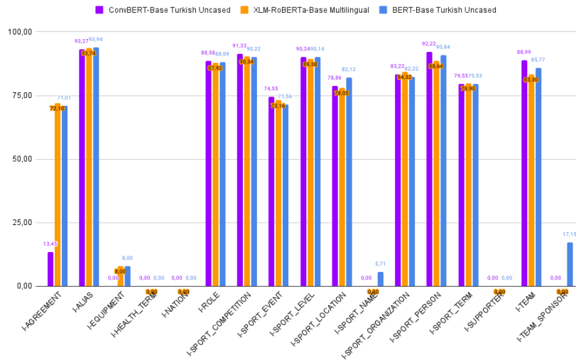
Figure 4.15: Label-wise F1-Scores of ConBERT-Base Turkish Uncased, XLM-RoBERTa-Base Multilingual Model and BERT-Base Turkish Uncased on TurkishSportsNER-Parent-BIO data set
