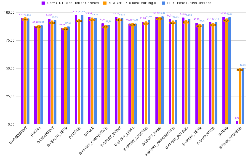
Figure 4.12: Label-wise Recall Values of ConBERT-Base Turkish Uncased, XLM-RoBERTa-Base Multilingual Model and BERT-Base Turkish Uncased on TurkishSportsNER-Parent-BIO data set
