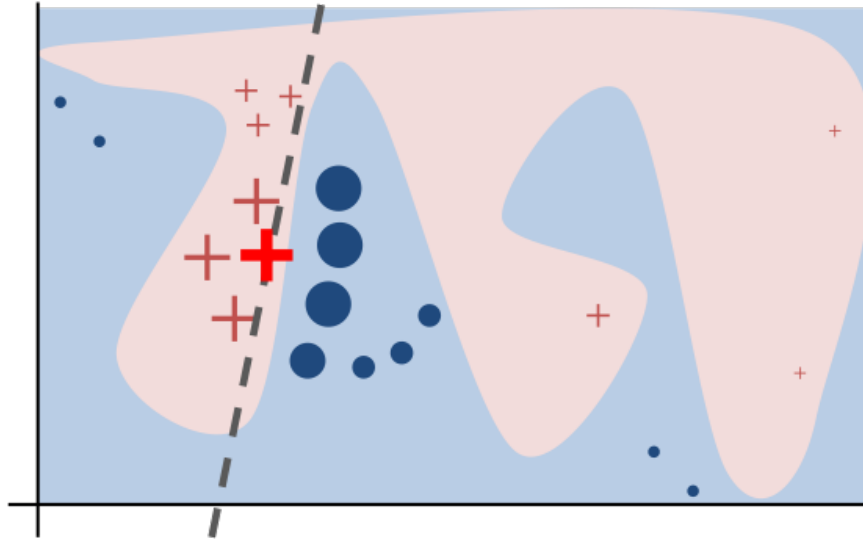
Figure 3.5: LIME Process. Sourced by [3]
