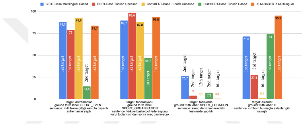
Figure 4.27: Prediction probability of ground truth annotation by LIME (In the x-axis, target word explained by LIME, ground truth label and sentence were given. The height of the bar indicates the probability assigned to correct label by the model according to LIME. )
