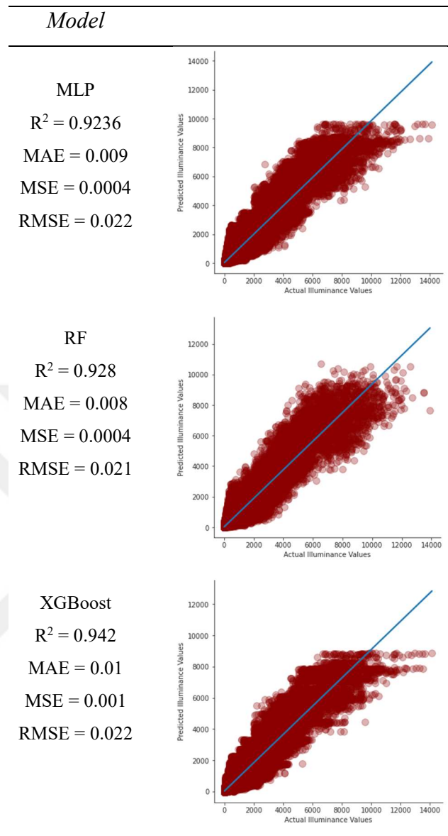
Figure 4.1 The performances of hyperparameter-tuned models
