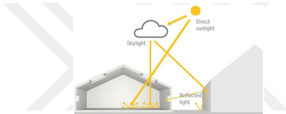
Figure 2.11. Components of daylighting (Roy, 2014)
