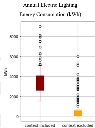
(b) : Total annual electric lighting energy consumption
