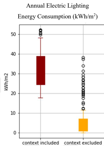
(a) : Annual electric lighting energy consumption per square meter
