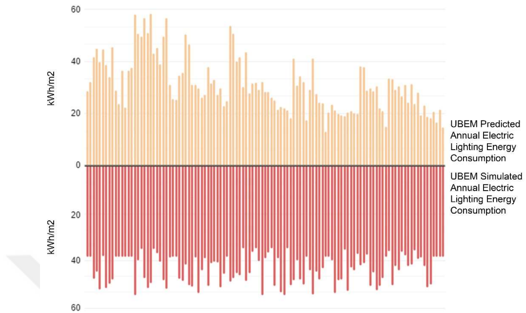
Figure 4.7 Comparison of annual electric lighting consumption in cases of UBEM predicted and simulated
