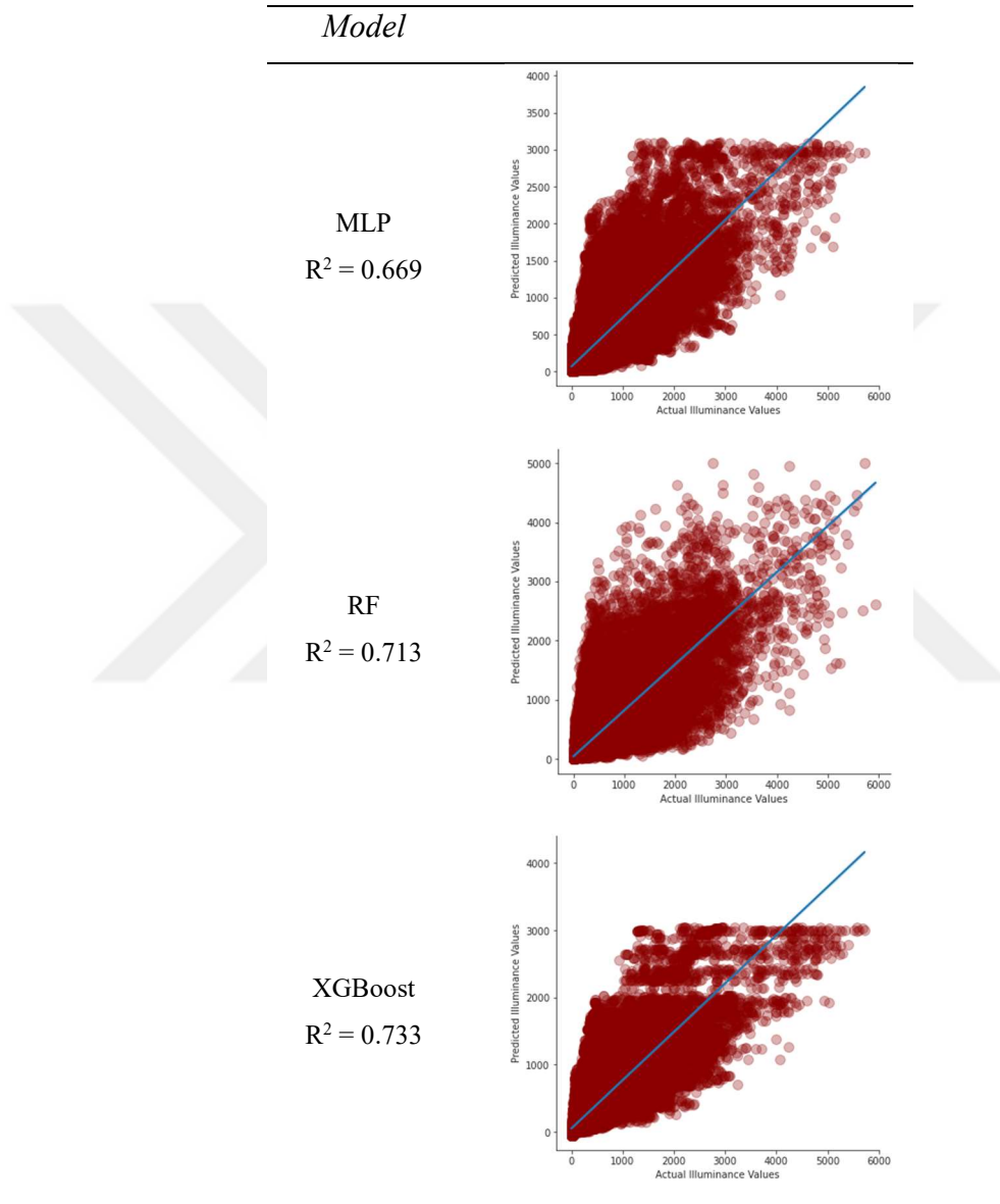
Figure 3.6 The graphs of the actual and predicted illuminance values
