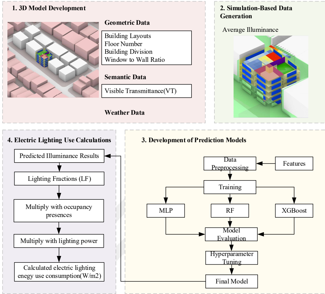
Figure 3.1. An overview of the proposed methodology
