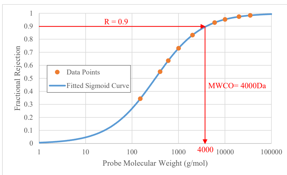
Figure 2.10 Example MWCO Curve Using PEG Probe Molecules of Differing MW For the curve in Figure 2.10, the MWCO value corresponds to 4000Da.
