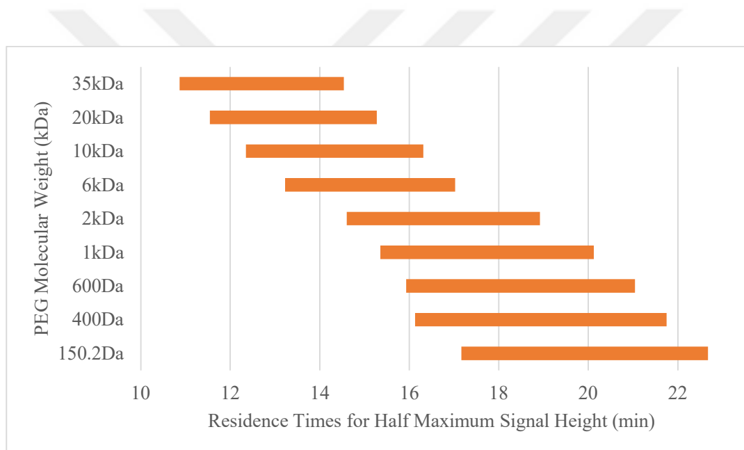
Figure 2.11 Residence Times for Half-Maximum RID Signal Heights
