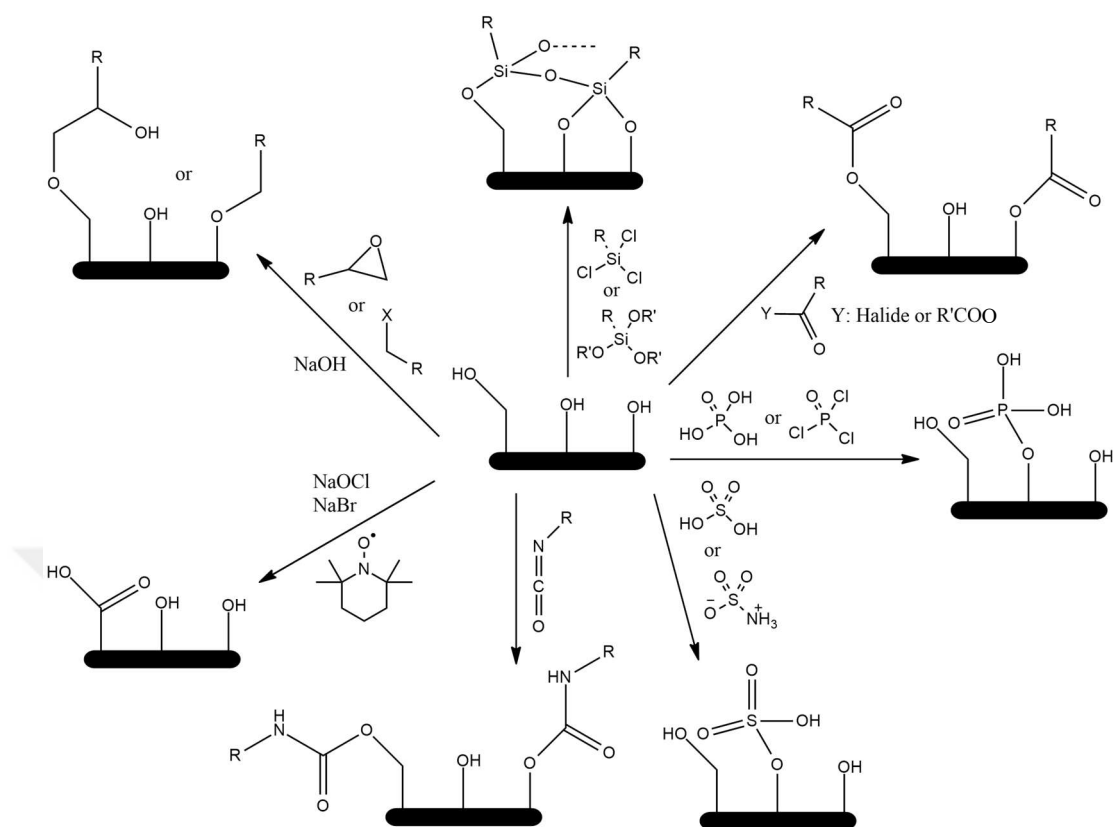
Figure 1.11 Chemical Derivatization of Nanocellulose
