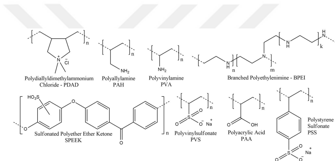
Figure 1.12 Polyelectrolyte Structures
