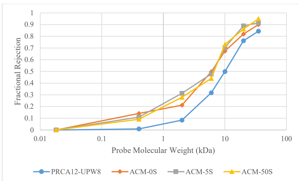
Figure 3.11 MWCO Curves of All-Cellulose Membranes
