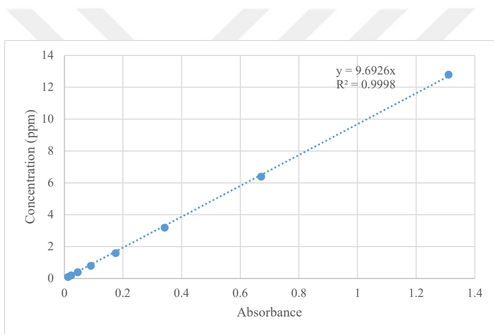
Figure 5.6 RB Calibration Curve in UPW at 550nm Wavelength
