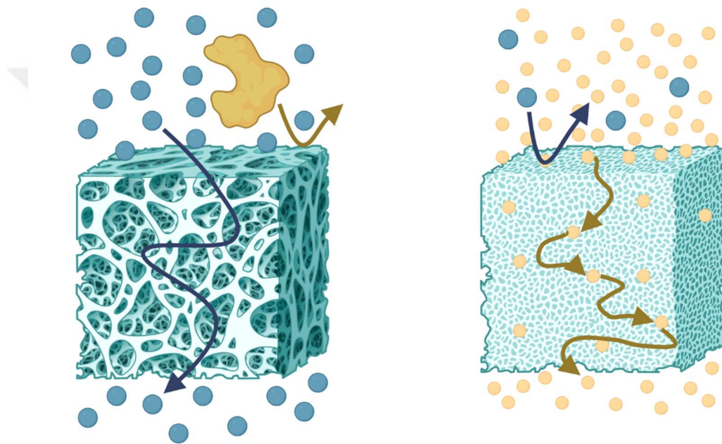
Figure 1.5 Illustration of Transport Across a Membrane: Pore-flow mode (left) and solution-diffusion mode (right)
