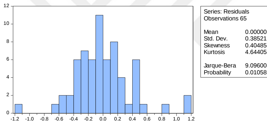
Figure 9: Histogram of the residuals and the Jarque-Bera statistic for testing normality-Model 1 ( Group 2 )
