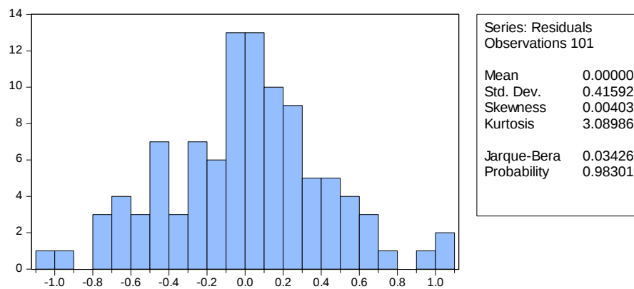
Figure 18: Histogram of the residuals and the Jarque-Bera statistic for testing normality- Model 4 ( Group 1 )
