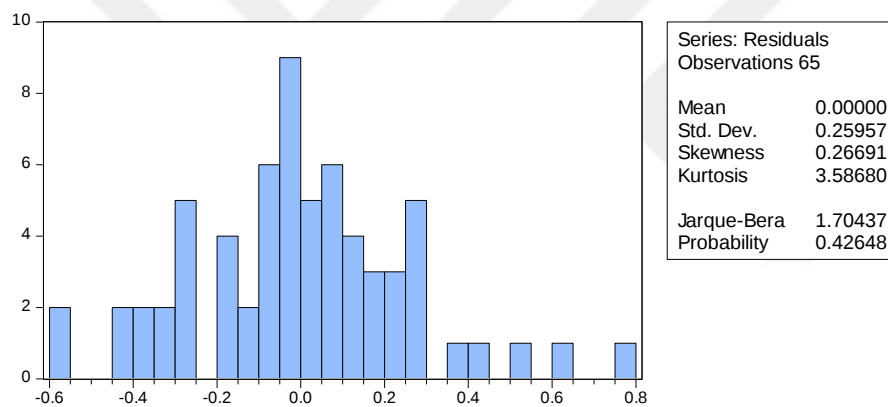
Figure 17: Histogram of the residuals and the Jarque-Bera statistic for testing normality- Model 3 ( Group 2 )
