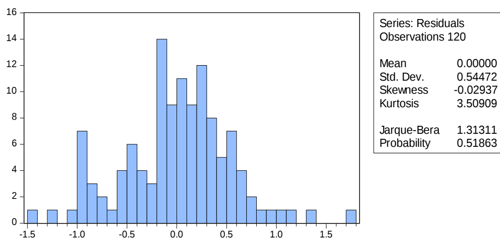
Figure 2: Histogram of the residuals and the Jarque-Bera statistic for testing normality- Model*(Group 1)
