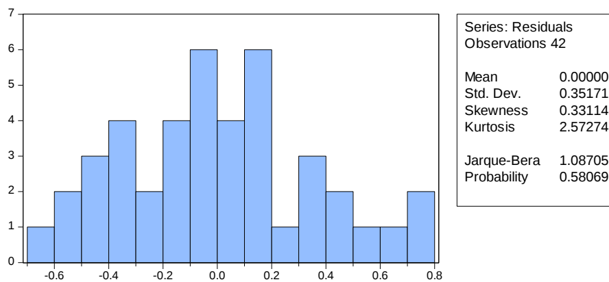
Figure 12: Histogram of the residuals and the Jarque-Bera statistic for testing normality- Model 2 ( Group 1.2 )
