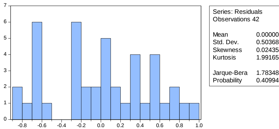
Figure 8: Histogram of the residuals and the Jarque-Bera statistic for testing normality-Model 1 ( Group 1.2 )
