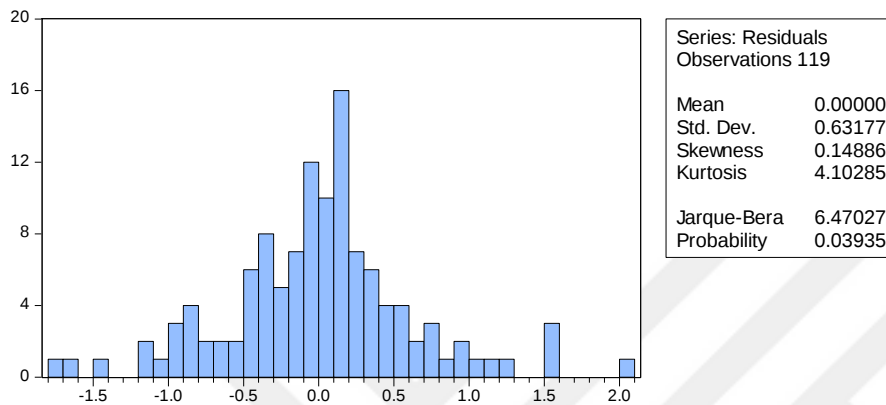
Figure 6: Histogram of the residuals and the Jarque-Bera statistic for testing normality-Model 1 ( Group 1 )
