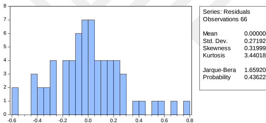
Figure 13: Histogram of the residuals and the Jarque-Bera statistic for testing normality- Model 2 ( Group 2 )
