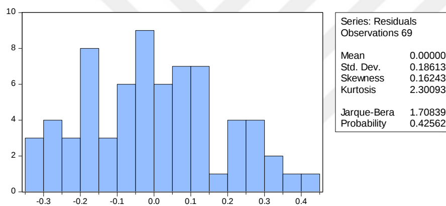
Figure 19: Histogram of the residuals and the Jarque-Bera statistic for testing normality- Model 4 ( Group 1.1 )
