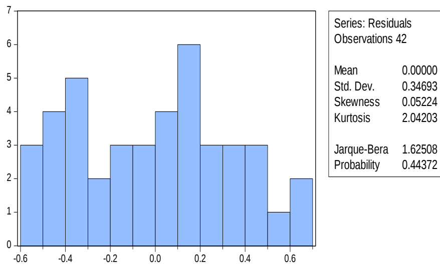
Figure 4: Histogram of the residuals and the Jarque-Bera statistic for testing normality- Model*(Group 1.2)
