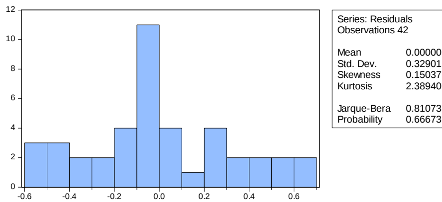
Figure 16: Histogram of the residuals and the Jarque-Bera statistic for testing normality- Model 3 ( Group 1.2 )
