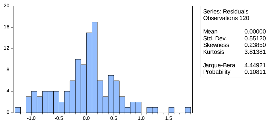
Figure 14: Histogram of the residuals and the Jarque-Bera statistic for testing normality- Model 3 ( Group 1 )
