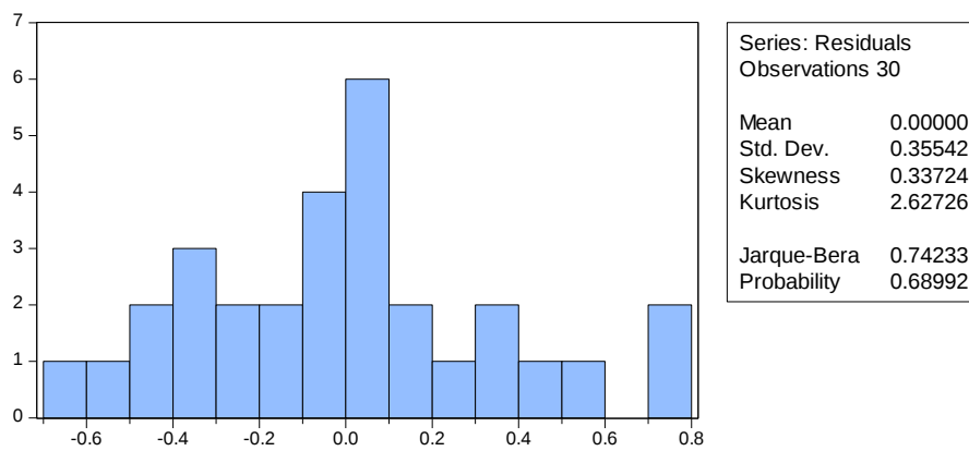
Figure 20: Histogram of the residuals and the Jarque-Bera statistic for testing normality- Model 4 ( Group 1.2 )
