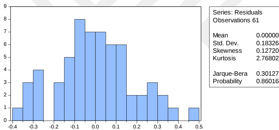
Figure 21: Histogram of the residuals and the Jarque-Bera statistic for testing normality-Model 4 ( Group 2 )
