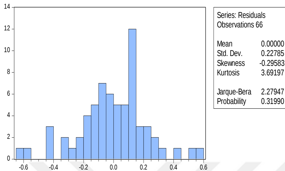
Figure 5: Histogram of the residuals and the Jarque-Bera statistic for testing normality- Model*(Group 2)
