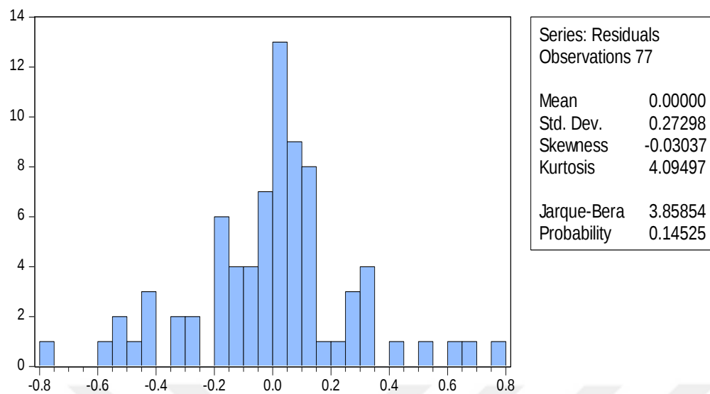
Figure 3: Histogram of the residuals and the Jarque-Bera statistic for testing normality- Model*(Group 1.1)
