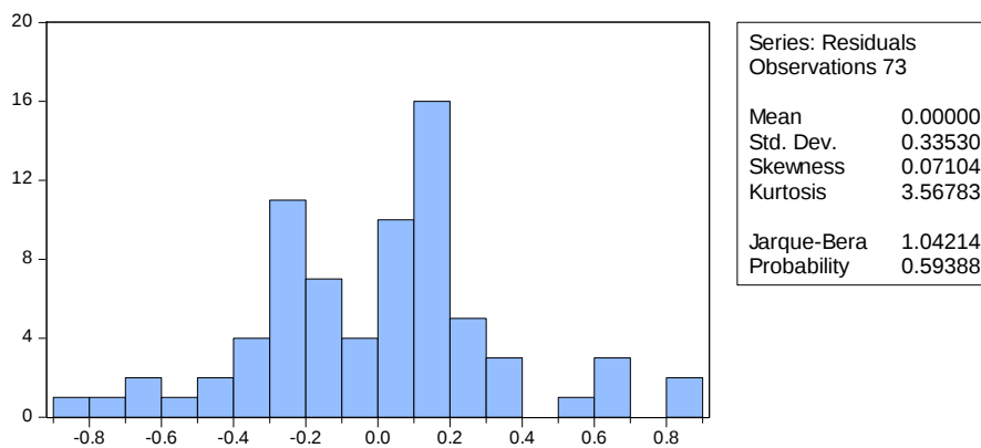
Figure 7: Histogram of the residuals and the Jarque-Bera statistic for testing normality- Model 1 ( Group 1.1 )
