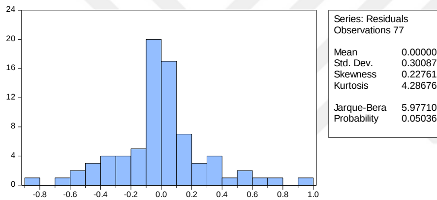
Figure 11: Histogram of the residuals and the Jarque-Bera statistic for testing normality- Model 2 ( Group 1.1 )
