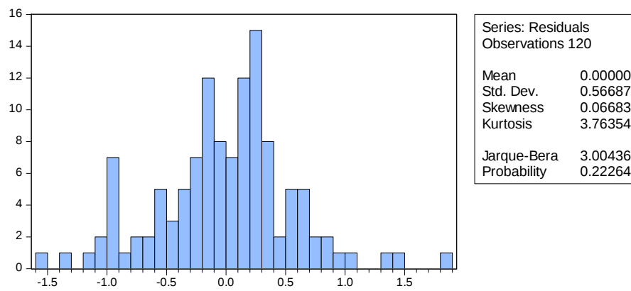
Figure 10: Histogram of the residuals and the Jarque-Bera statistic for testing normality- Model 2 ( Group 1 )
