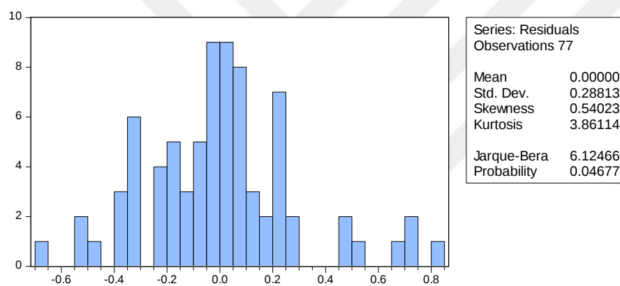
Figure 15: Histogram of the residuals and the Jarque-Bera statistic for testing normality- Model 3 ( Group 1.1 )
