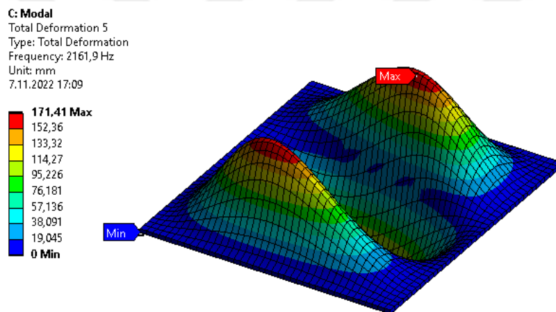
Figure 4-77. Fourth mode shape of the fiber-reinforced [0_2/-45_2/45_2/90_2]_s laminated clamped plate with a/b = 1 , h/a = 0.016 using ANSYS
