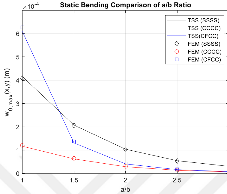
Figure 4-90. Effects of a/b ratio on the maximum deflection of the fiber-reinforced [0_2/-45_2/45_2/90_2]_s laminated simply supported, clamped, and single free three clamped plate with q = 0.01 MPa, h/a = 0.016 using trigonometric series solution (TSS) with M=12 and N=12 and ANSYS
