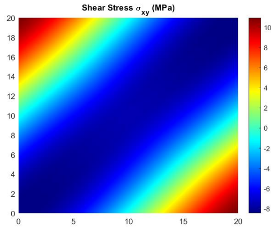
Figure 4-27. \sigma_{xy} distribution determined by trigonometric series solution with M , N=12 at z = 1.6 mm of 0^\circ ply in fiber-reinforced laminated simply supported plate \sigma_{xy} distribution that is determined by using trigonometric series solution (TSS) of -45^\circ ply at z = 1.2 mm is expressed in Figure 4-28. Maximum shear stress occurred in 45^\circ or -45^\circ fiber oriented plies.
