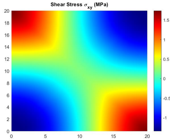
Figure 4-27. \sigma_{xy} distribution determined by trigonometric series solution with M , N=12 at z = 1.6 mm of 0^\circ ply in fiber-reinforced laminated simply supported plate \sigma_{xy} distribution that is determined by using trigonometric series solution (TSS) of -45^\circ ply at z = 1.2 mm is expressed in Figure 4-28. Maximum shear stress occurred in 45^\circ or -45^\circ fiber oriented plies.
