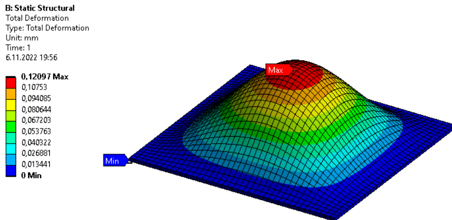
Figure 4-11. Distribution of deformation of the fiber-reinforced [0_2/-45_2/45_2/90_2]_s laminated clamped plate with q = 0.01 MPa, a/b = 1 , h/a = 0.016 using ANSYS
