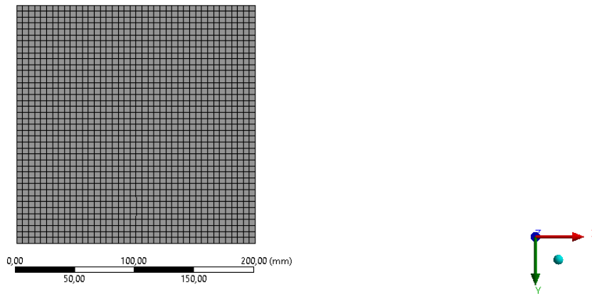
Figure 4-3. Mesh model of fiber-reinforced plate in ANSYS
