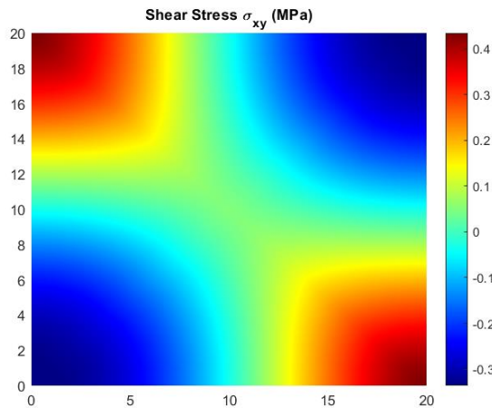
Figure 4-30. \sigma_{xy} distribution determined by trigonometric series solution with M , N=12 at z = 0.4 mm of 90^\circ ply in fiber-reinforced laminated simply supported plate
