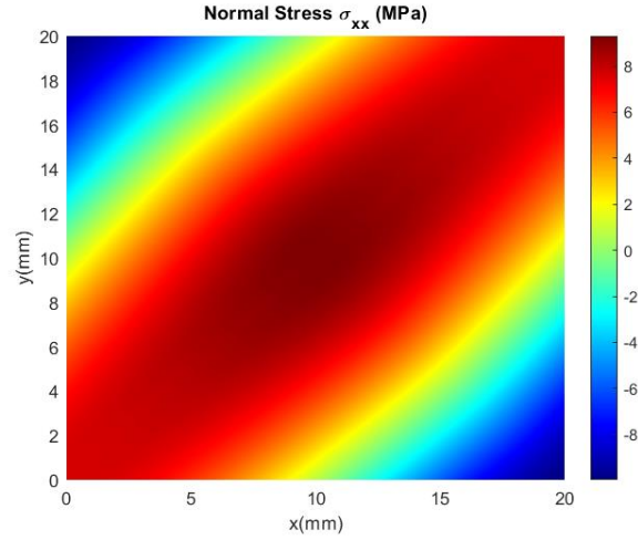
Figure 4-20. \sigma_{xx} distribution determined by trigonometric series solution with M , N=12 at z = 1.2 mm of -45^\circ ply in fiber-reinforced laminated simply supported plate
