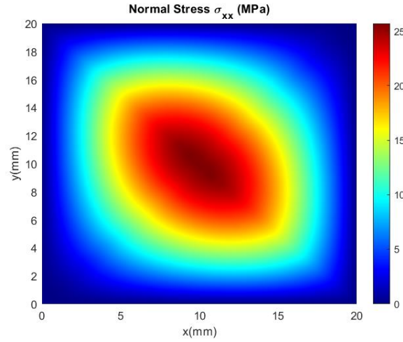
Figure 4-19. \sigma_{xx} distribution determined by trigonometric series solution with M , N=12 at z = 1.6 mm of 0^\circ ply in fiber-reinforced laminated simply supported plate
