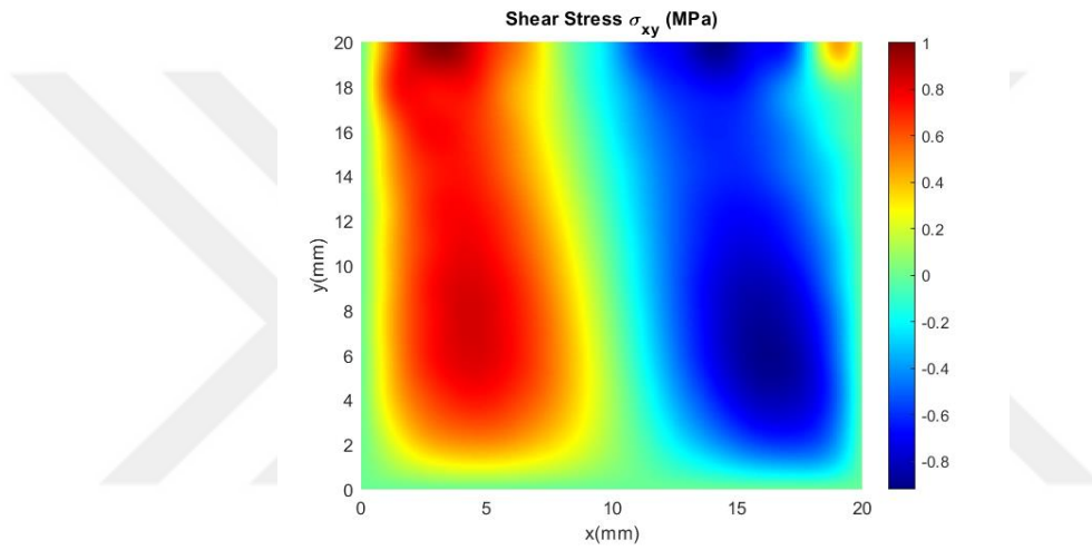
Figure 4-57. \sigma_{xy} distribution determined by trigonometric series solution with M, N=12 at z = 1.6 mm of 0^\circ ply in fiber-reinforced laminated single free and three clamped plate
