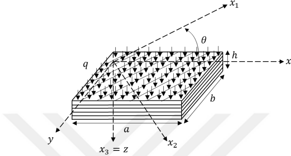
Figure 4-6. Bending problem geometry of fiber-reinforced [0_2/-45_2/45_2/90_2]_s laminated plate
