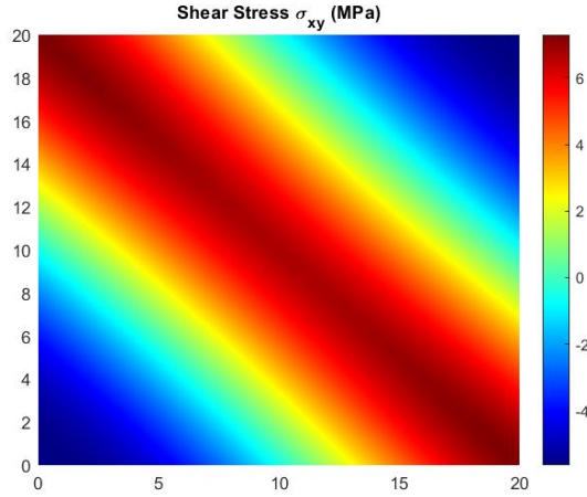
Figure 4-29. \sigma_{xy} distribution determined by trigonometric series solution with M , N=12 at z = 0.8 mm of 45^\circ ply in fiber-reinforced laminated simply supported plate
