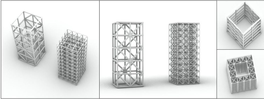
Figure 30 Truss System and Proposed Cellular Structure (developed by author).
