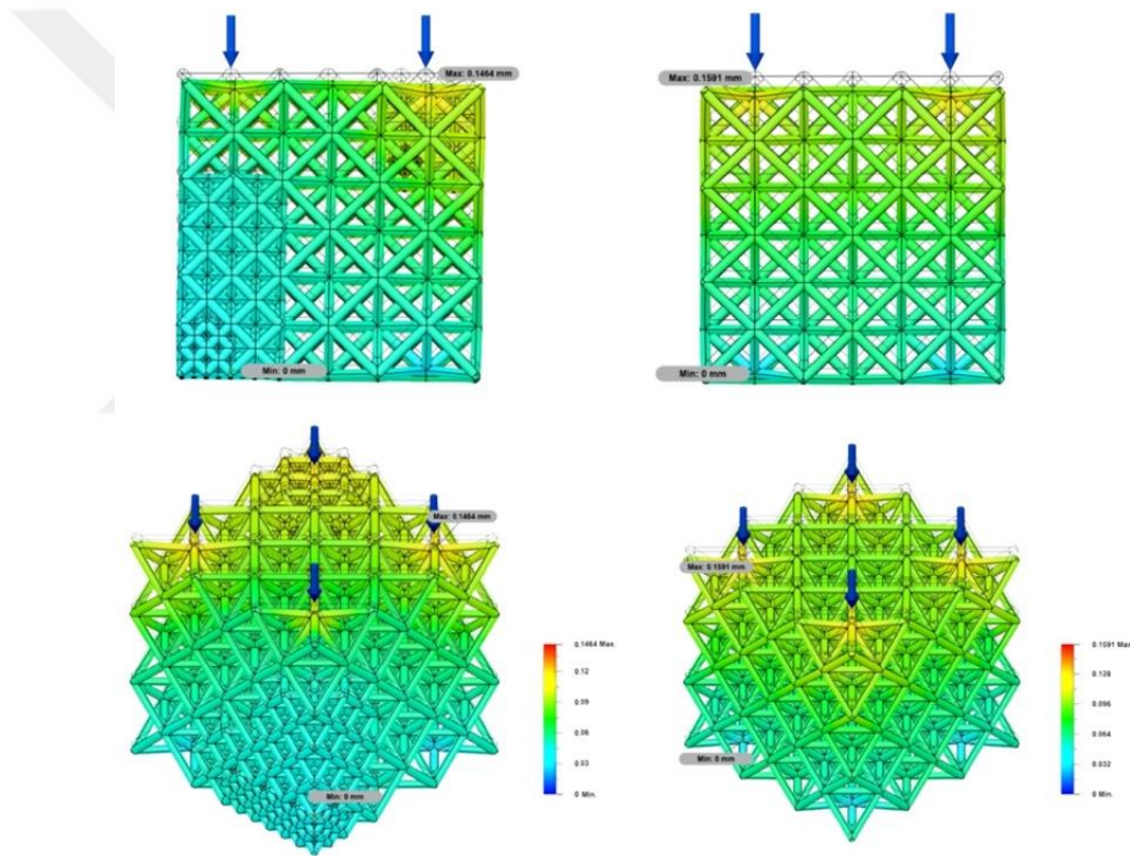
Figure 29 Comparison of uniform lattice structure and lattice generated by octree algorithm (developed by author)
