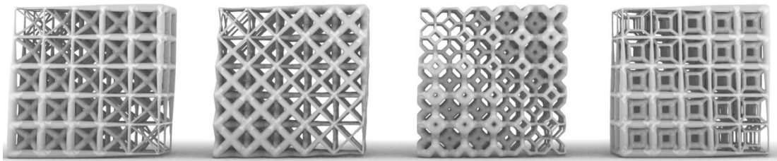
Figure 27 Variable density different type unit cell structures (developed by author).
