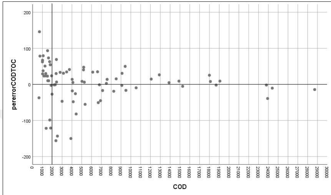
Figure C.1. Percent error chart for COD and TOC regression model
