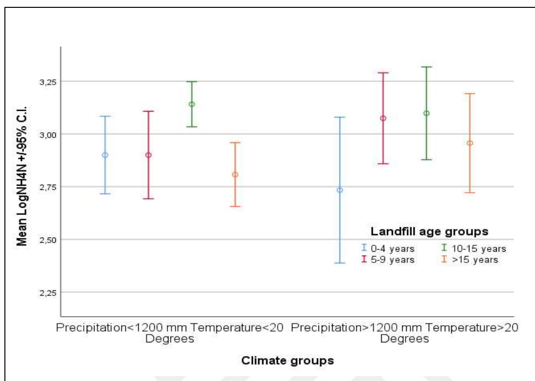
Figure 6.17. Confidence interval for mean values of LogNH 4 -N for each group
