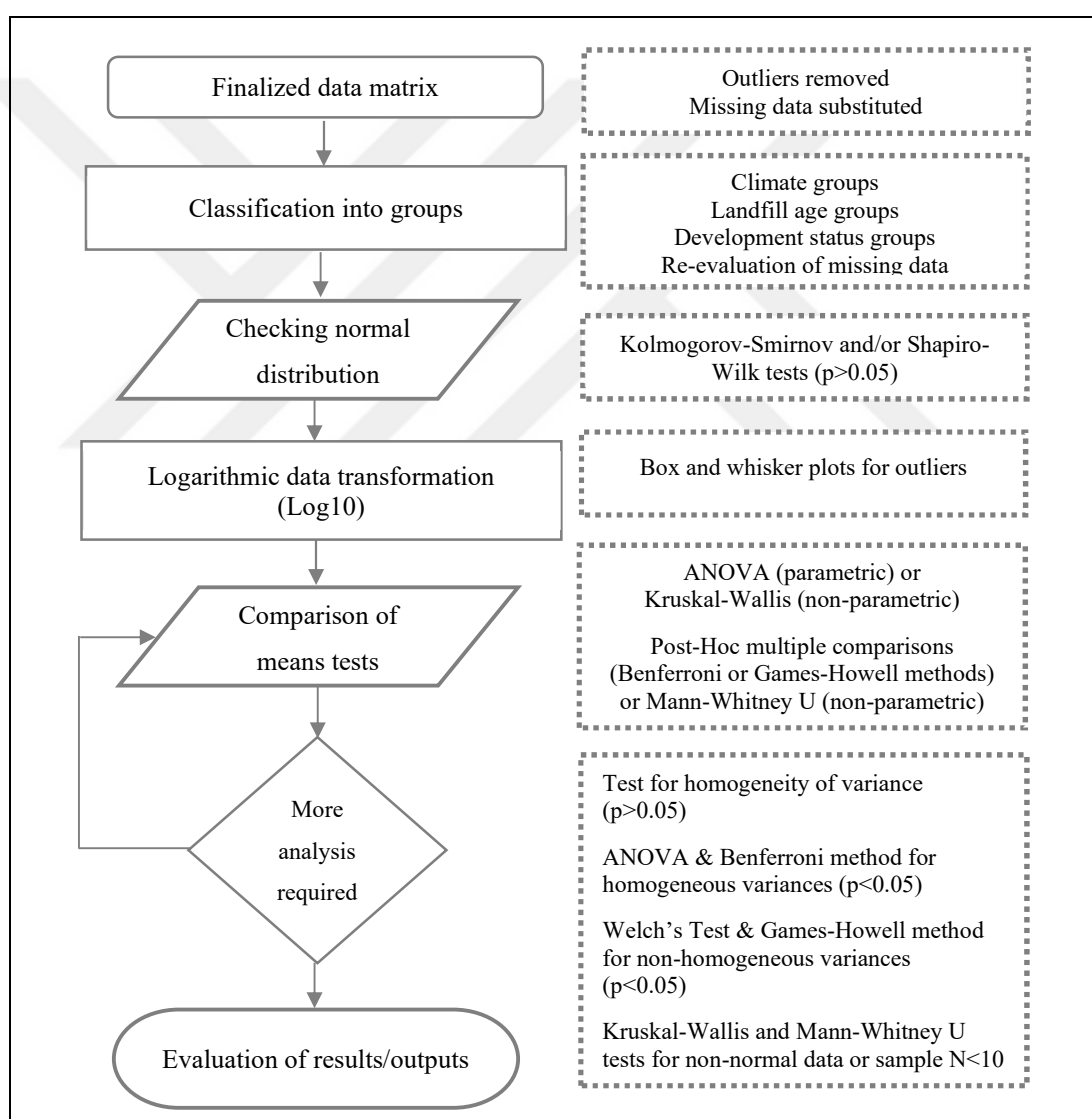
Figure 6.3. Flowchart for data preparation and analysis steps
