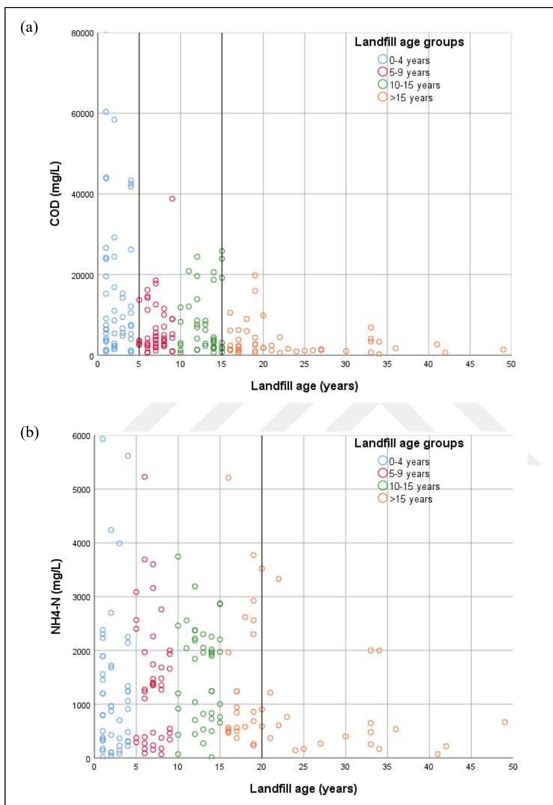
Figure 6.5. Values of leachate (a) COD and (b) NH 4 -N according to the landfill age
