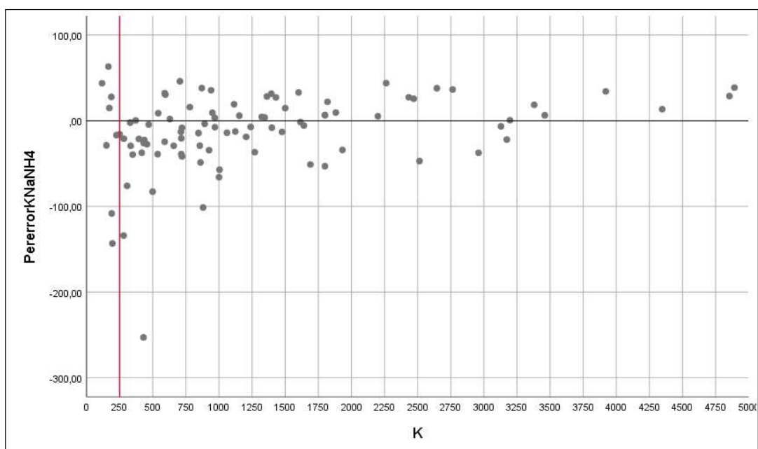
Figure C.7. Percent error chart for K and Na-NH 4 -N regression model
