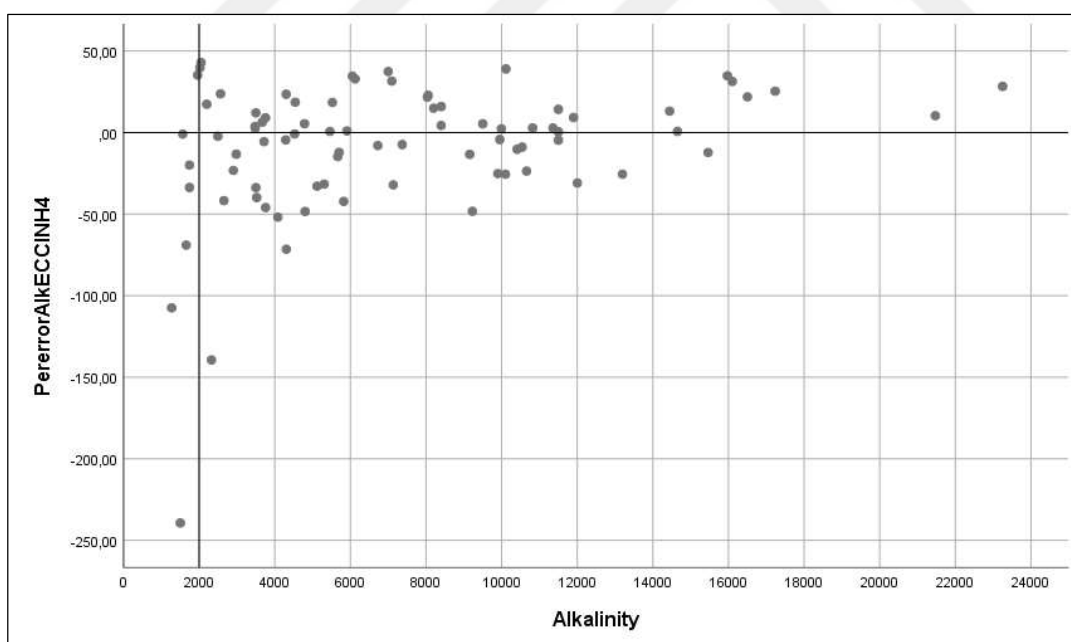
Figure C.4. Percent error chart for Alkalinity and EC-Cl-NH 4 -N regression model
