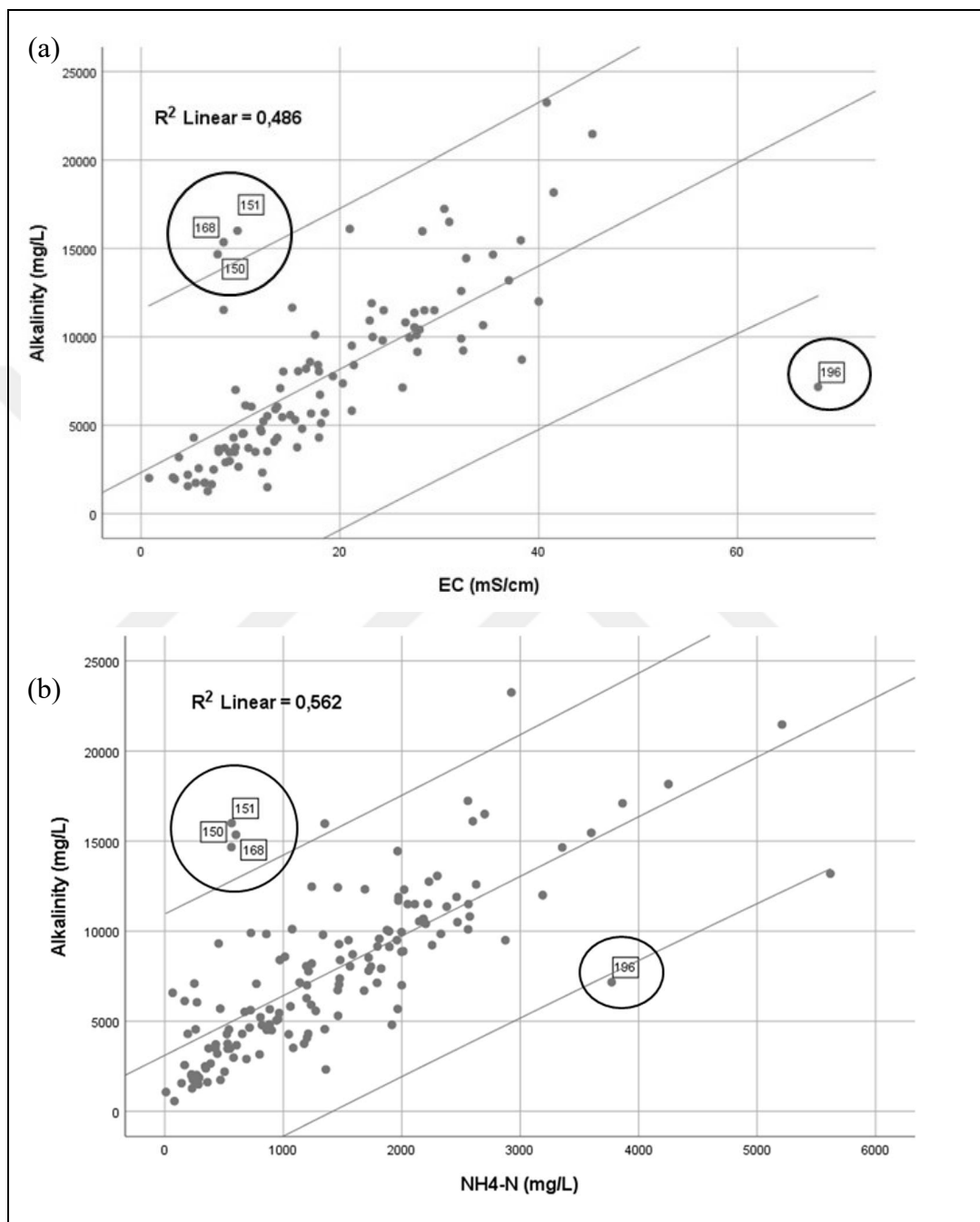
Figure 5.2. Example of outlier data (circled) with scatter plots for (a) EC vs Alkalinity and (b) \text{NH}_4\text{-N} vs Alkalinity (the upper and lower lines show 99% prediction interval; the numbers within boxes indicate landfill ID)
