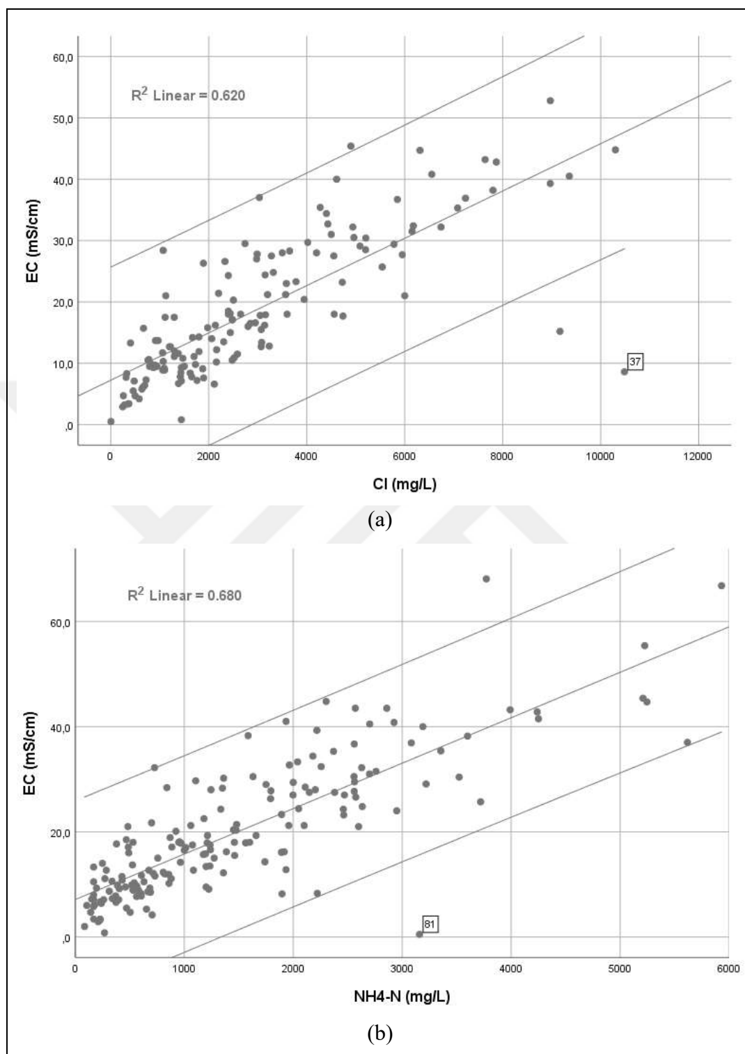
Figure B.1. Outlier data (circled) with scatter plots for (a) Cl vs EC (b) NH 4 -N vs EC (the upper and lower lines show 99% prediction interval; the numbers within boxes indicate landfill ID)
