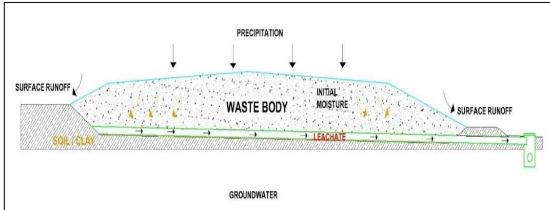
Figure 2.1. General view of leachate formation and collection in landfills
