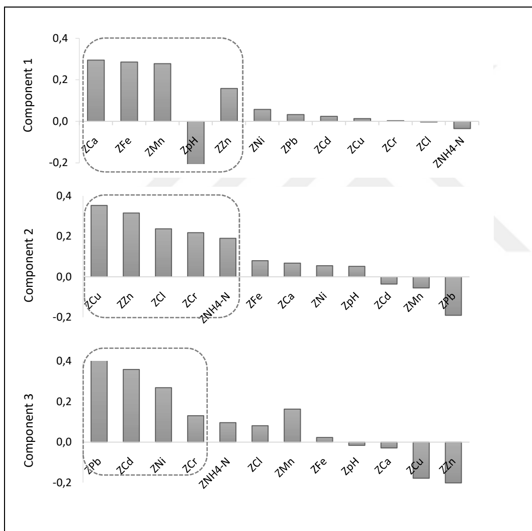
Figure 5.11. Component score charts for the PCA of inorganics and heavy metal content of leachate
