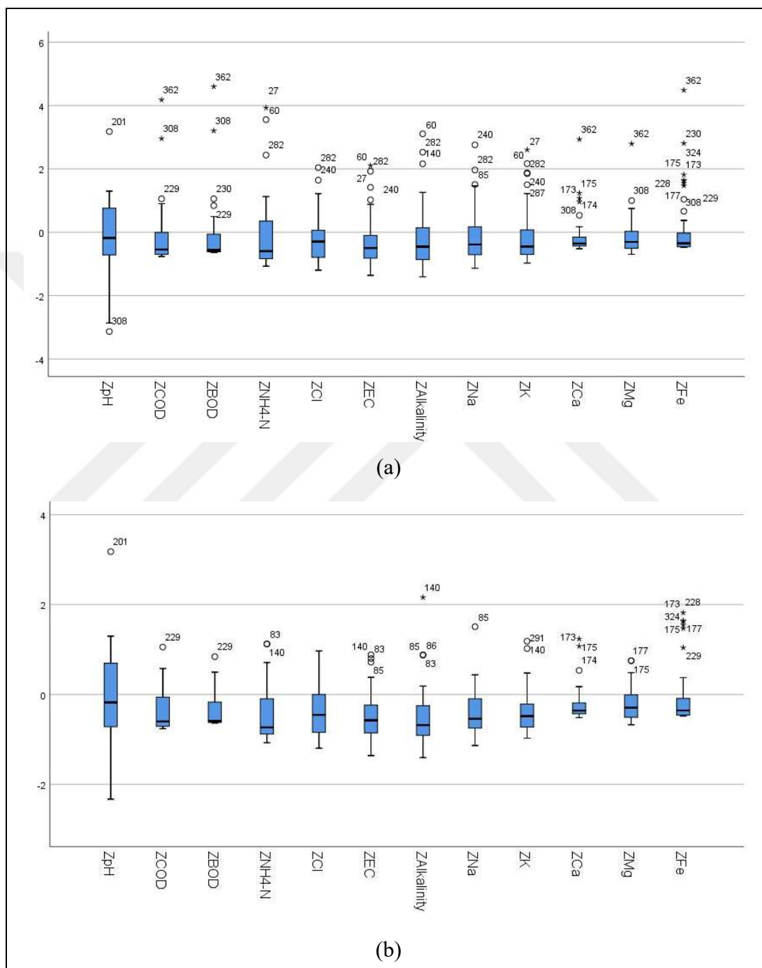
Figure 5.6. Box and whisker plots for the selected 12 leachate parameters (a) with outliers (b) after removal of extreme outliers
