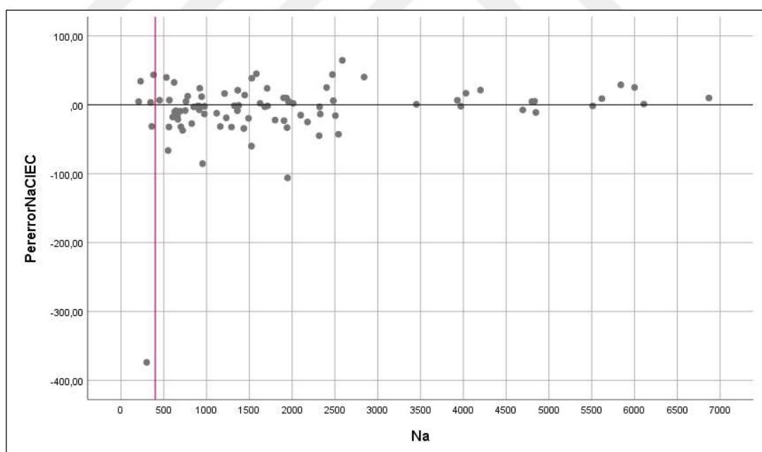
Figure C.6. Percent error chart for Na and Cl-EC regression model
