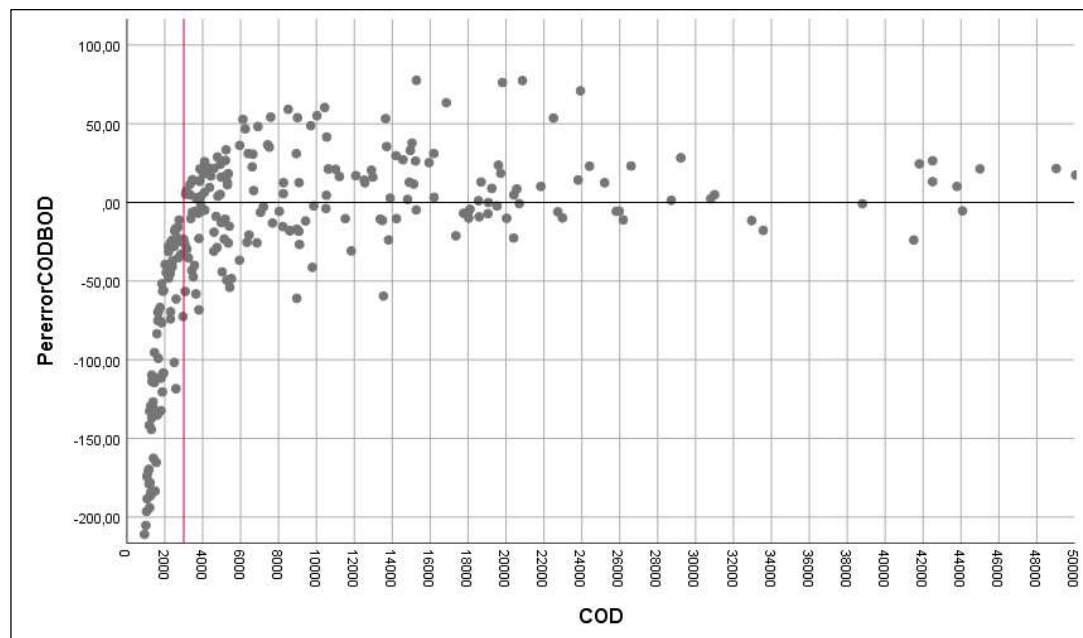
Figure C.2. Percent error chart for COD and BOD regression model
