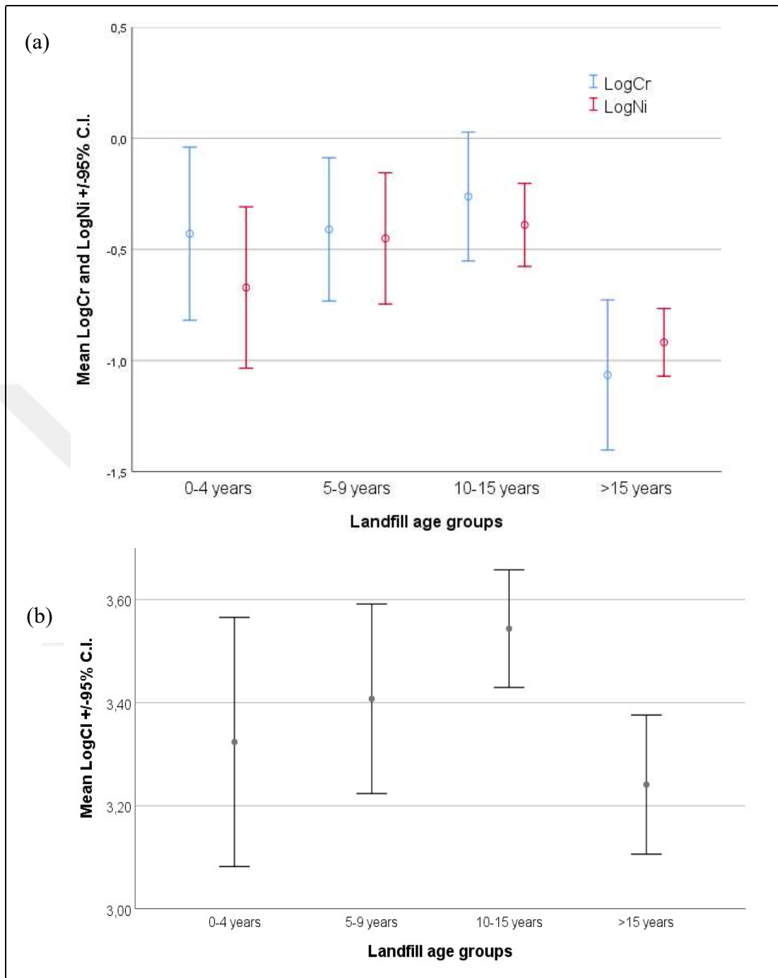
Figure 6.12. Confidence interval for mean values of (a) logCr and LogNi (b) logCl at each landfill age case for the first climate group
