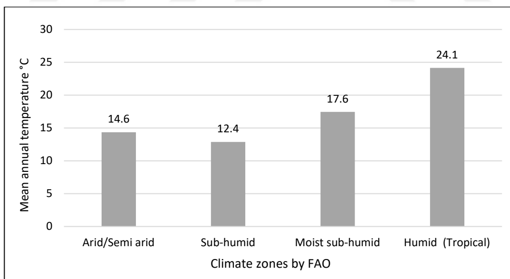
Figure 6.2. Mean temperature values for the landfills included in each climate zone
