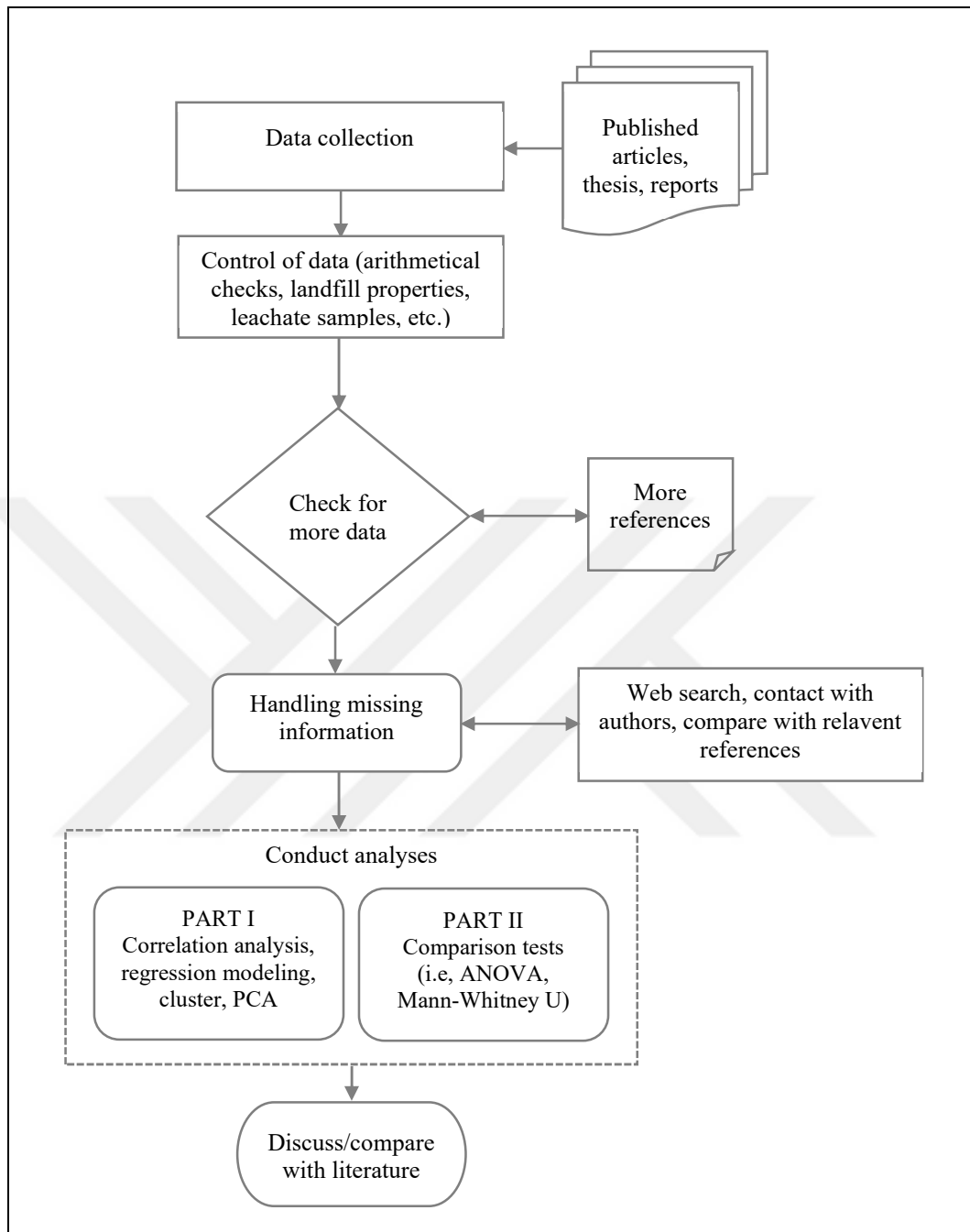
Figure 3.2. Algorithm of major data collection and analysis activities
