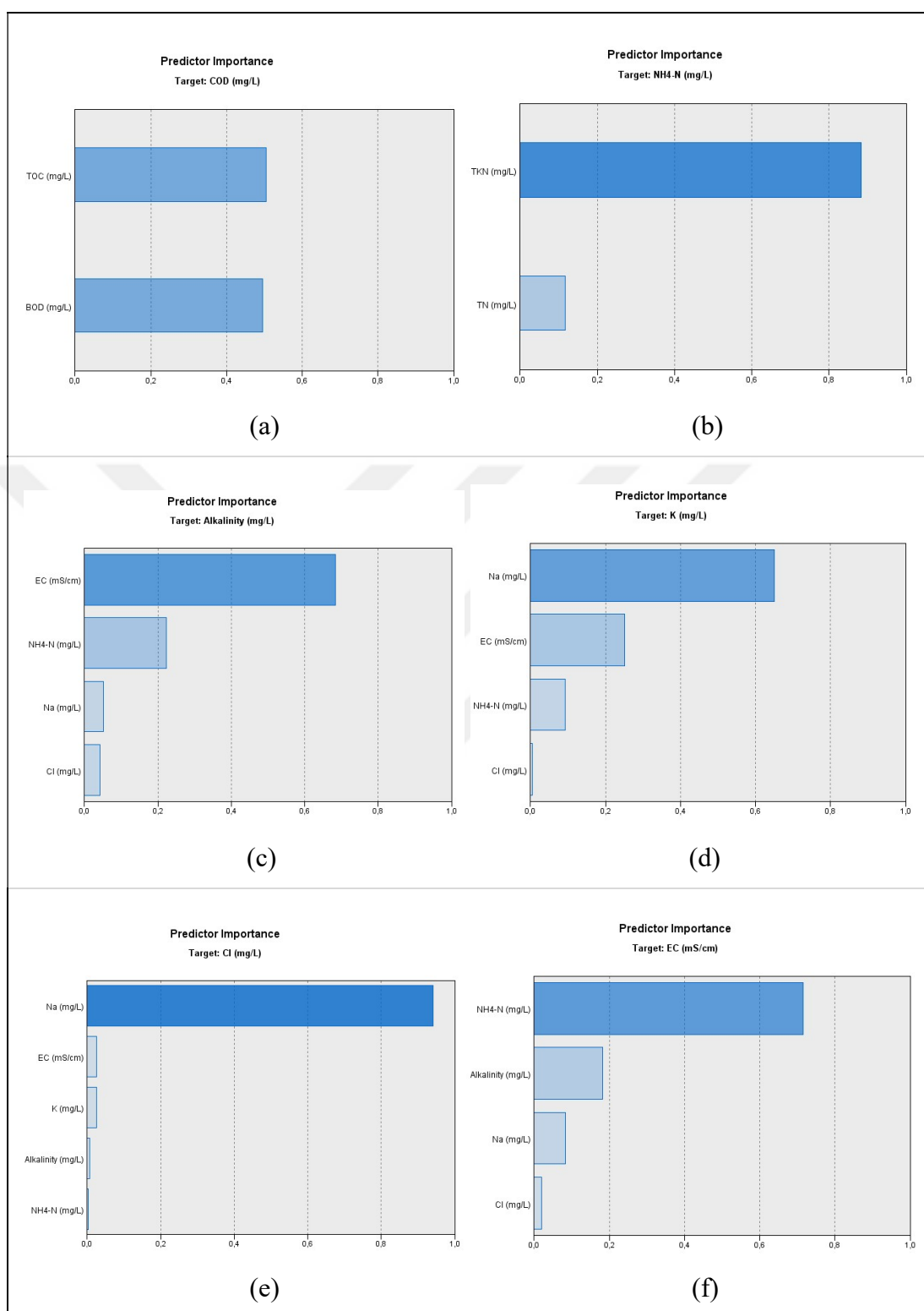
Figure 5.3. Predictor importance charts for the regression model variables as (a) COD (b) NH 4 -N (c) Alkalinity (d) K (e) Cl and (f) EC
