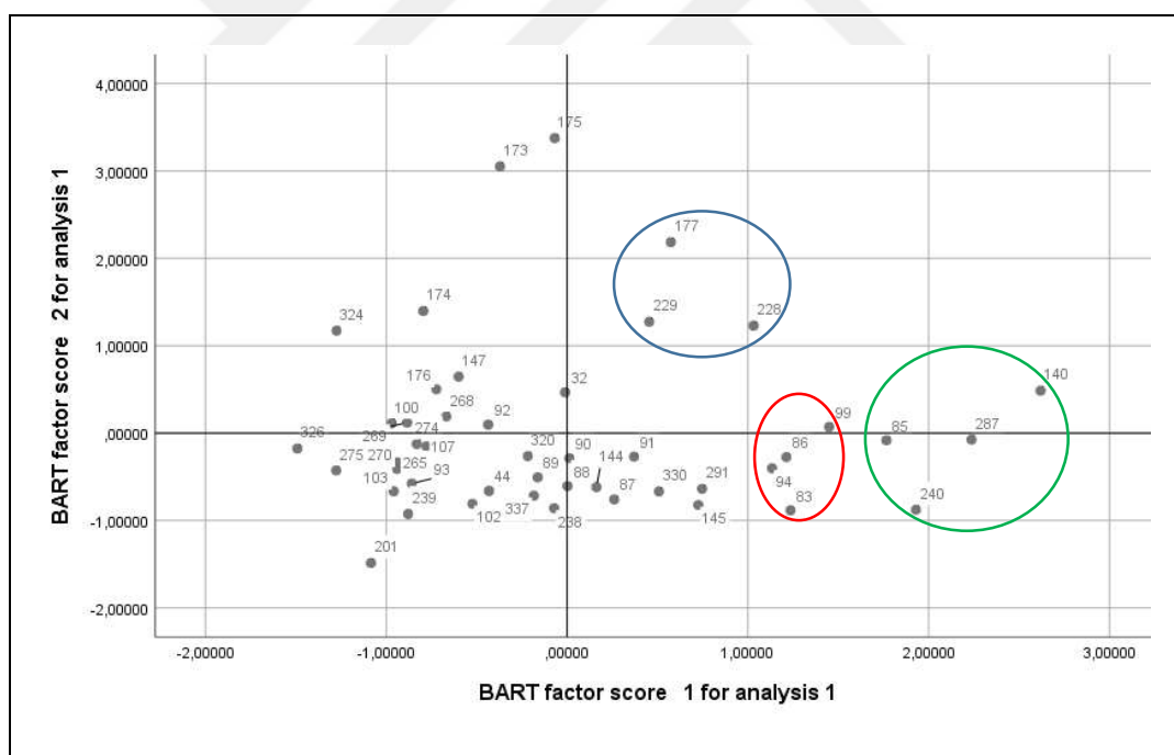
Figure 5.9. Scatter plots of the principal component scores with 10 leachate parameters
