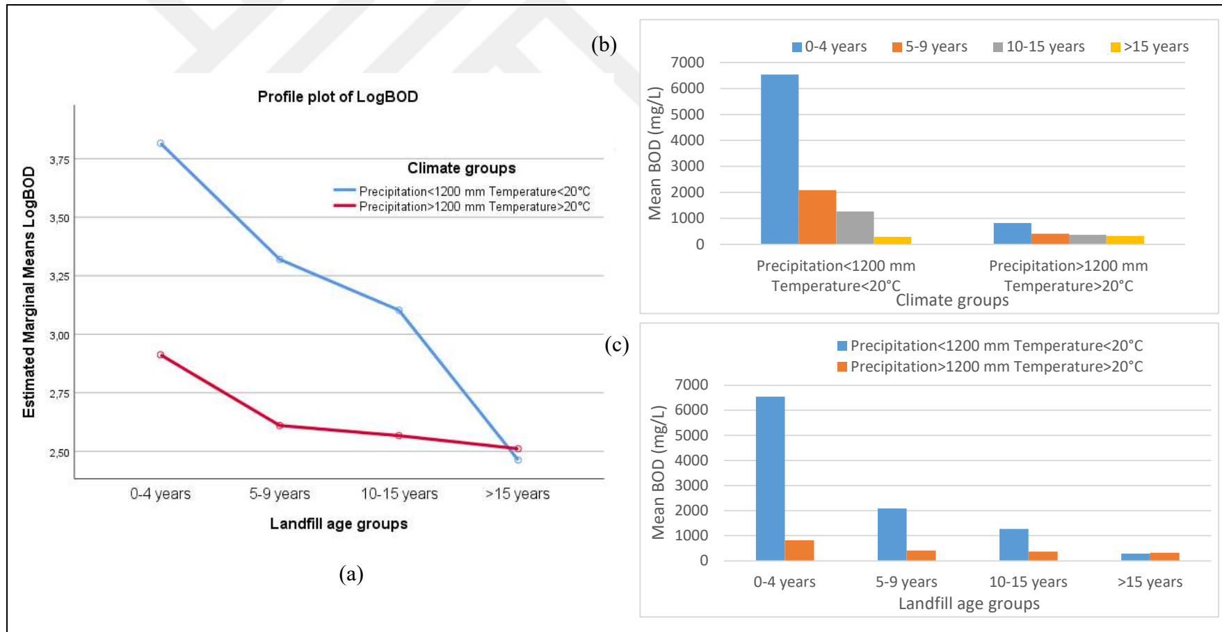
Figure 6.8. ANOVA results for leachate BOD in different age/climate groups (a) Profile plot (b) Mean BOD values according to climate groups (c) Mean BOD values according to landfill age groups
