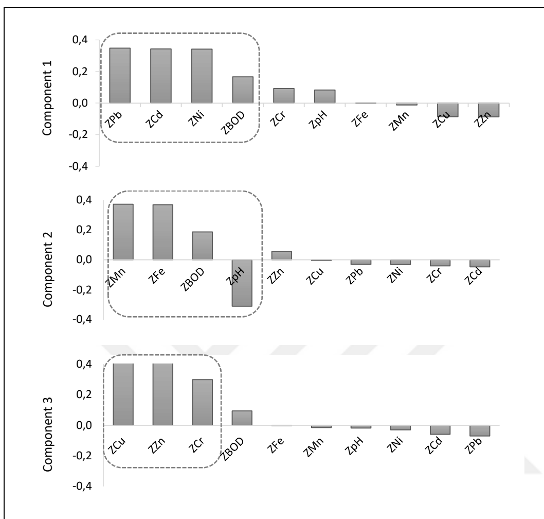
Figure 5.10. Component score charts for the PCA of organics and heavy metal content of leachate
