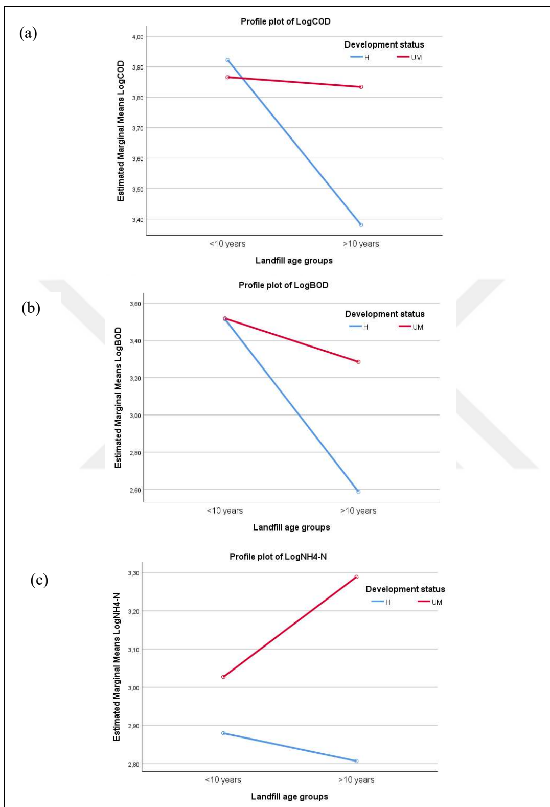
Figure 6.15. Interaction effect of development status and landfill age on leachate parameters of (a) COD (b) BOD (c) \text{NH}_4\text{-N}
