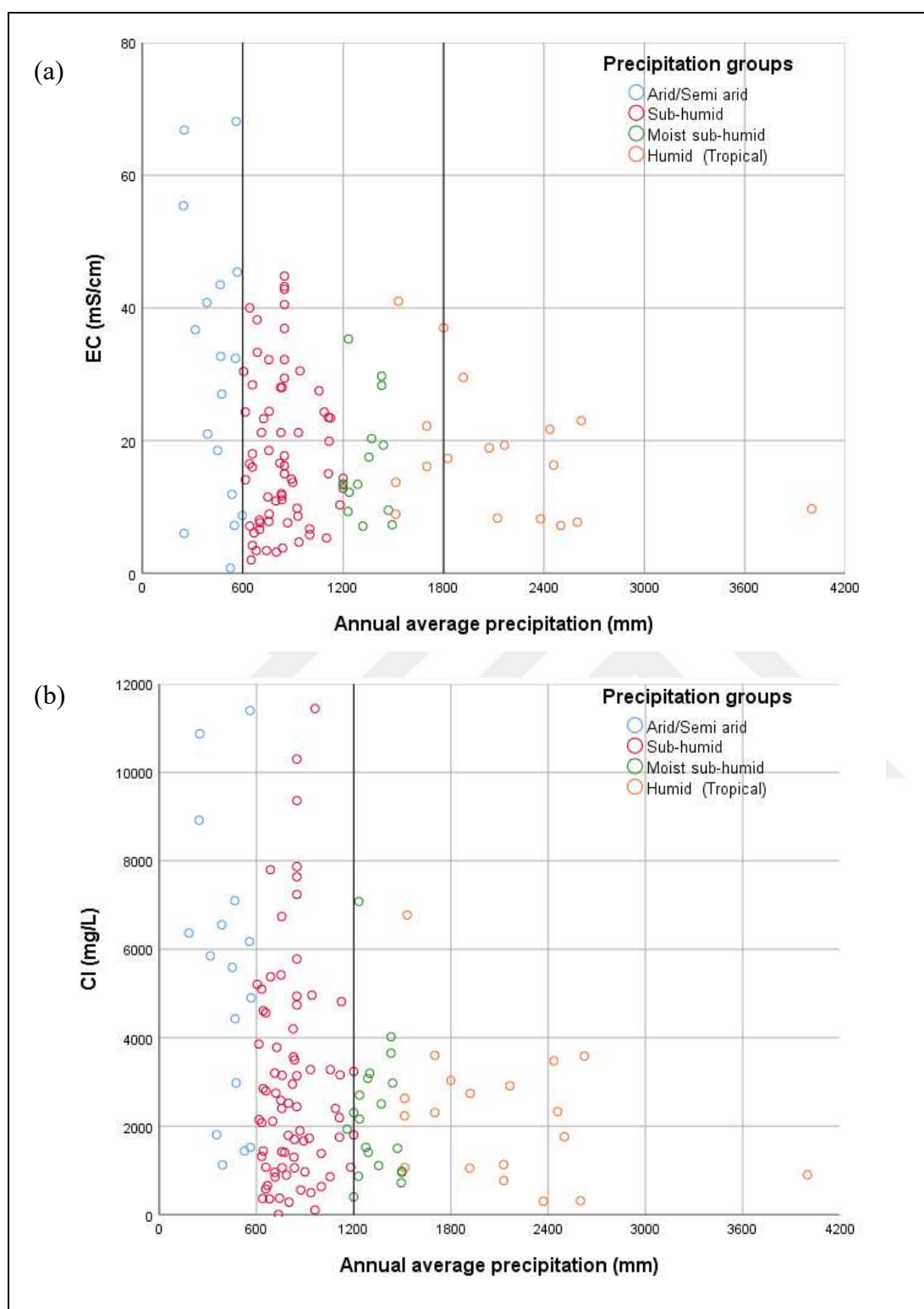
Figure 6.4. Values of leachate (a) EC and (b) Cl according to annual precipitation rates
