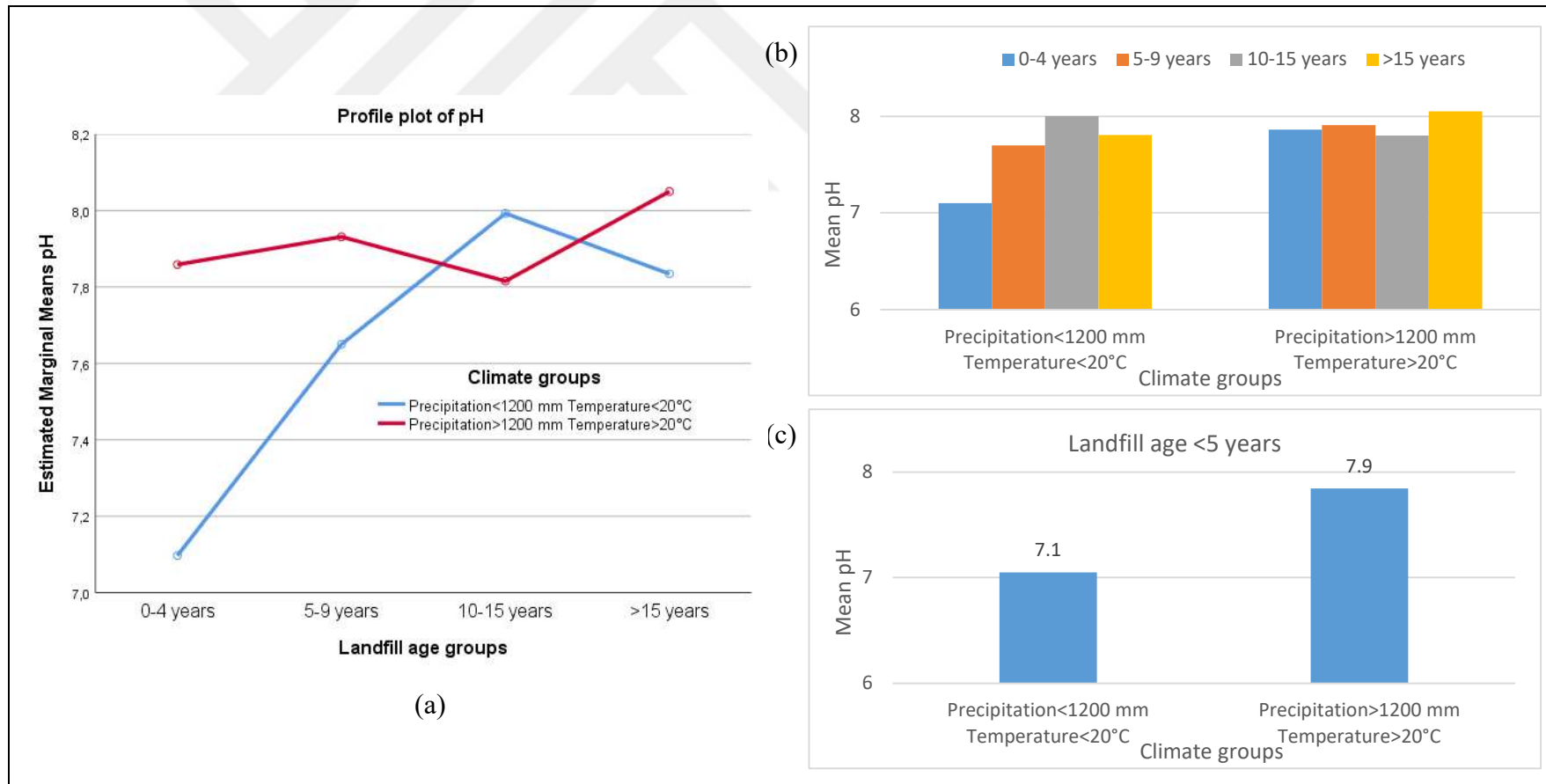
Figure 6.6. ANOVA results for leachate pH in different age/climate groups (a) Profile plot (b) Mean pH values according to climate groups (c) Mean pH values for landfill age<5 years between climate groups
