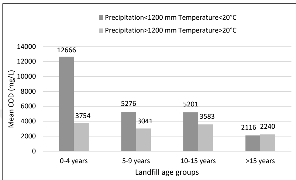
Figure 6.14. Trends of organics in leachate between different climate&age groups
