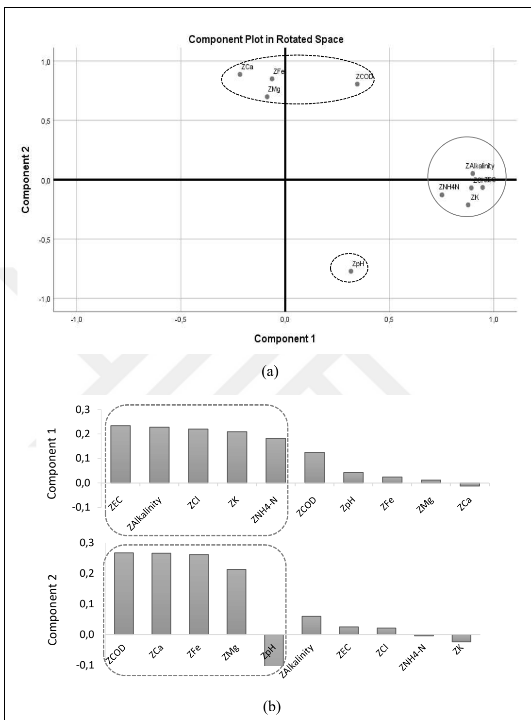
Figure 5.8. PCA results with 10 leachate parameters (a) Component plot (b) Score chart
