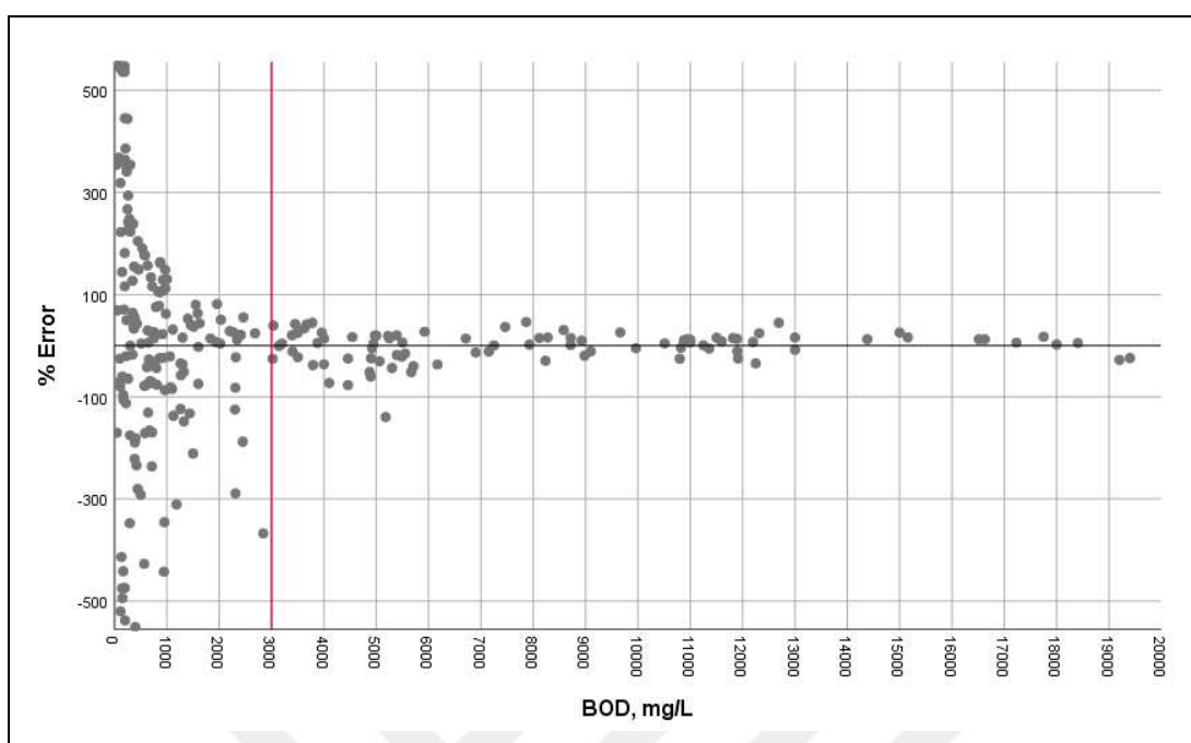
Figure 5.5. Sample % error chart for BOD-COD regression model
