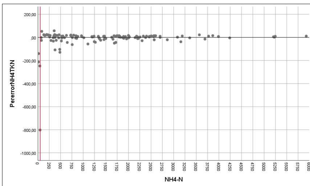
Figure C.3. Percent error chart for NH 4 -N and TKN regression model
