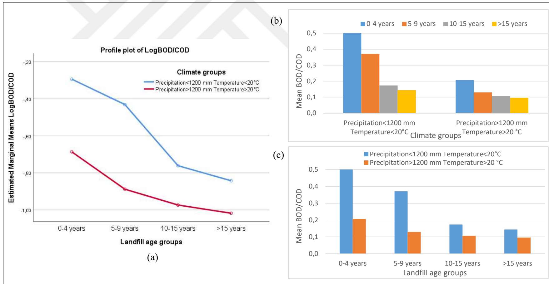
Figure 6.9. ANOVA results for leachate BOD/COD in different age/climate groups (a) Profile plot (b) Mean BOD/COD values according to climate groups (c) Mean BOD/COD values according to landfill age groups
