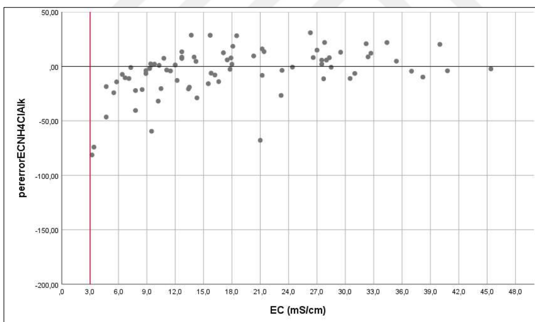
Figure C.8. Percent error chart for EC and NH 4 -N-Cl-Alkalinity regression model
