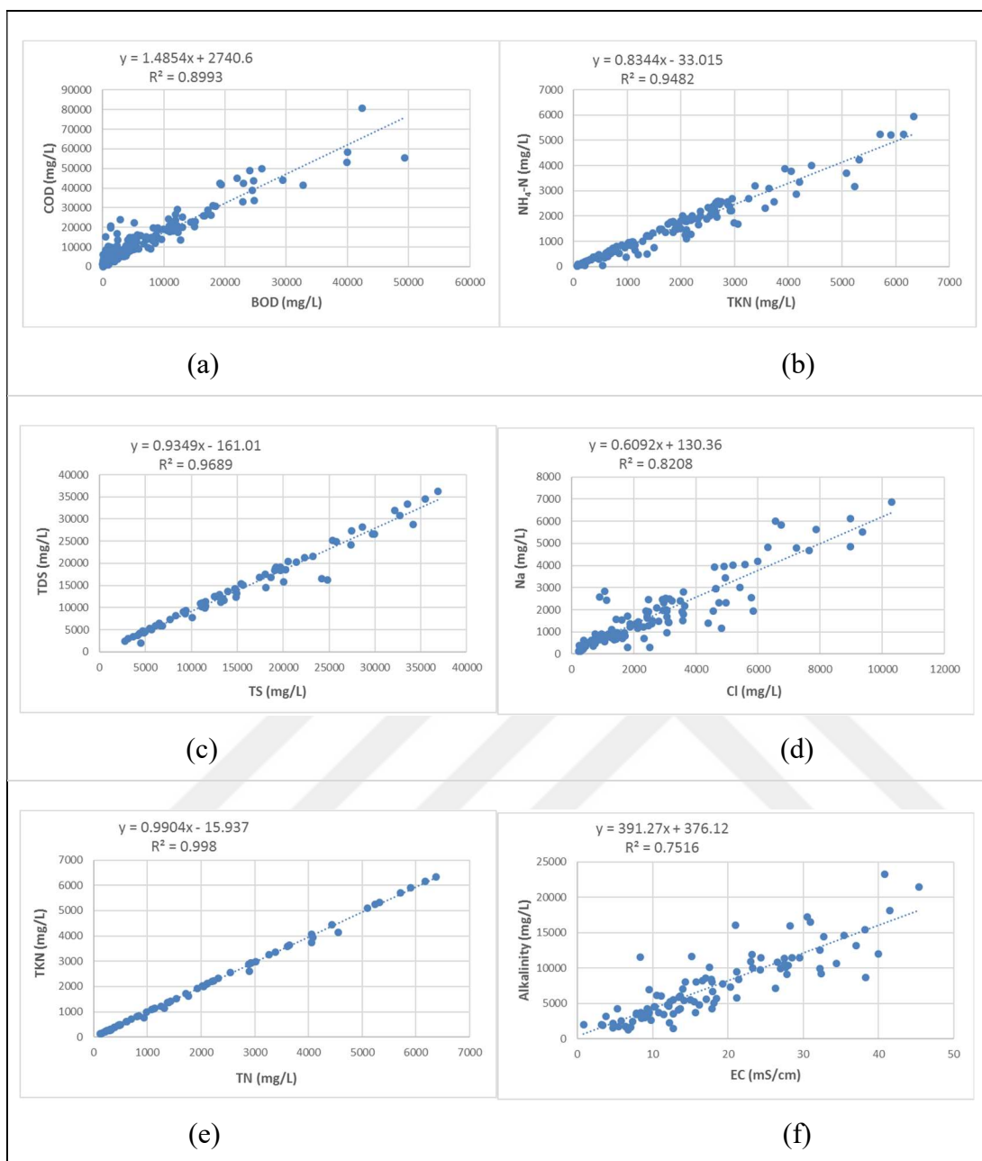
Figure 5.4. Sample regression plots for (a) BOD vs COD (b) TKN vs \text{NH}_4\text{-N} (c) TS vs TDS (d) Cl vs Na (e) TN vs TKN (f) EC vs Alkalinity
