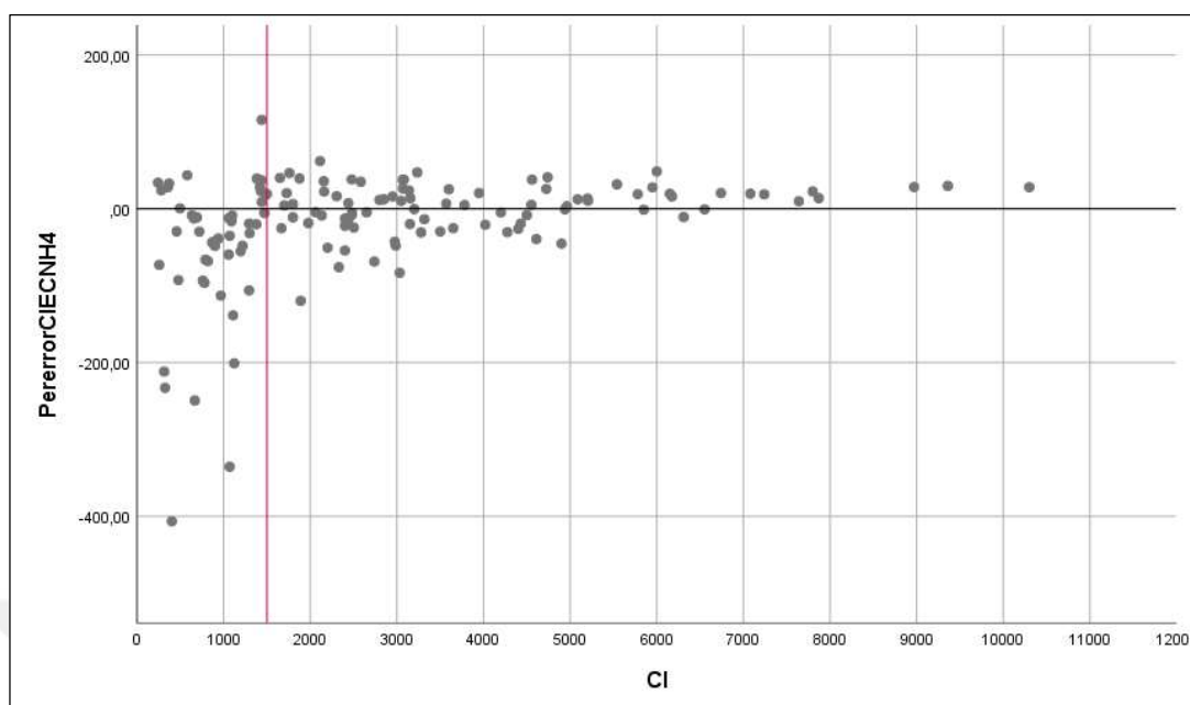
Figure C.5. Percent error chart for Cl and EC-NH 4 -N regression model
