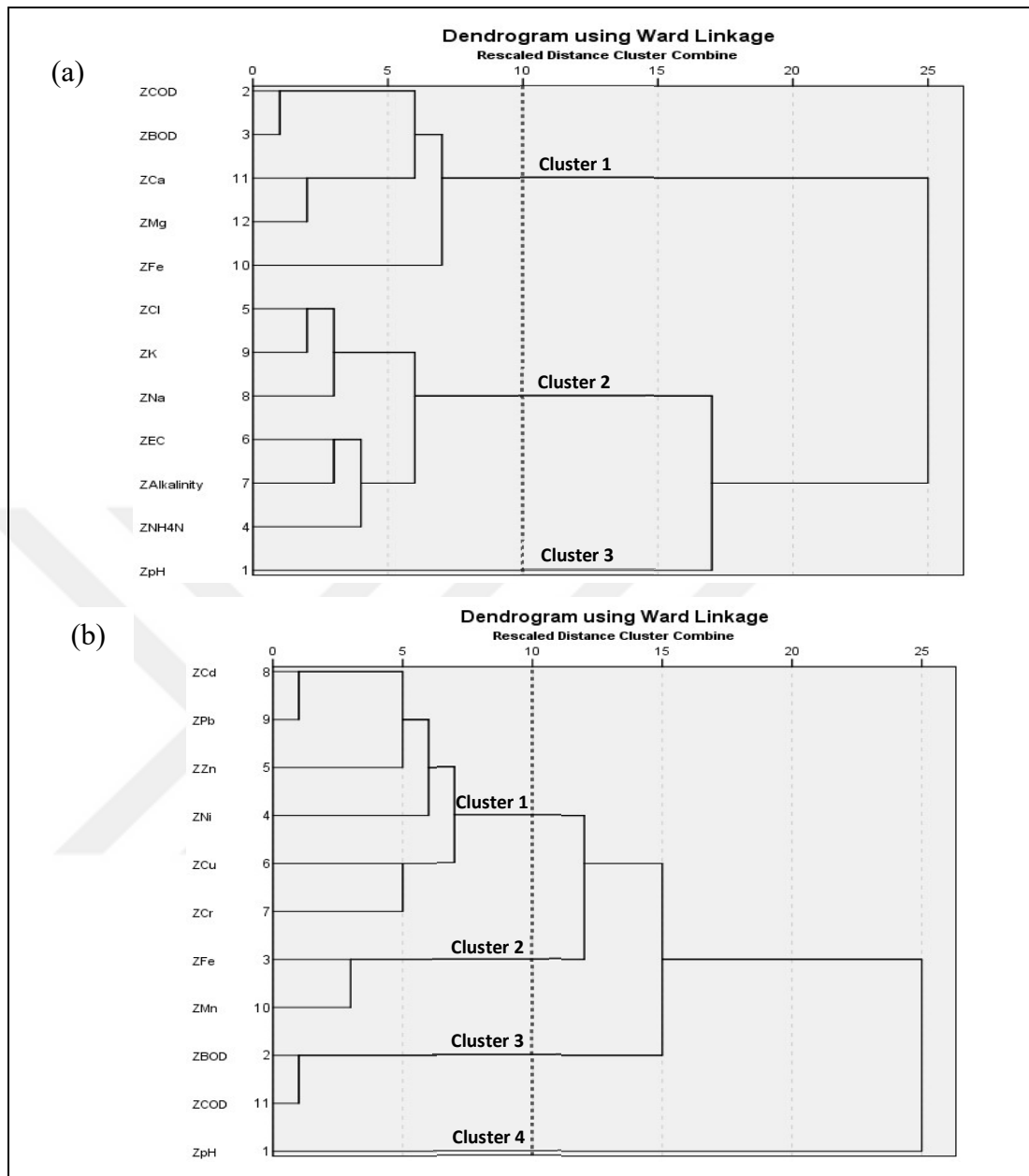
Figure 5.7. Dendrograms showing the clustering of standardized (a) 12 leachate parameters (Sample N=36) (b) leachate parameters including heavy metals (Sample N=63)
