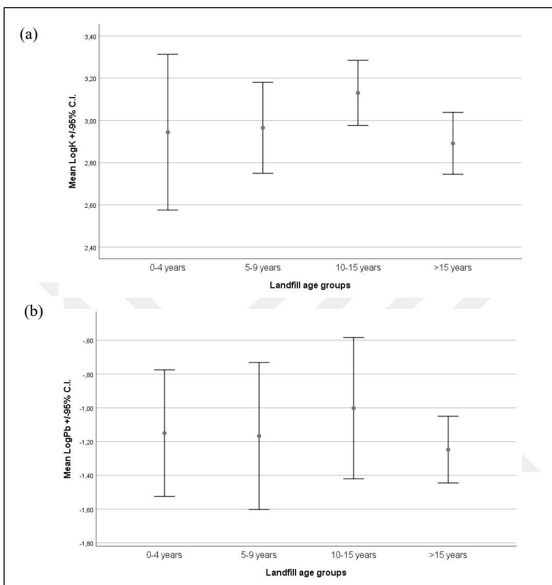
Figure 6.13. Confidence interval for mean values of (a) logK (b) logPb at each landfill age case for the first climate group
