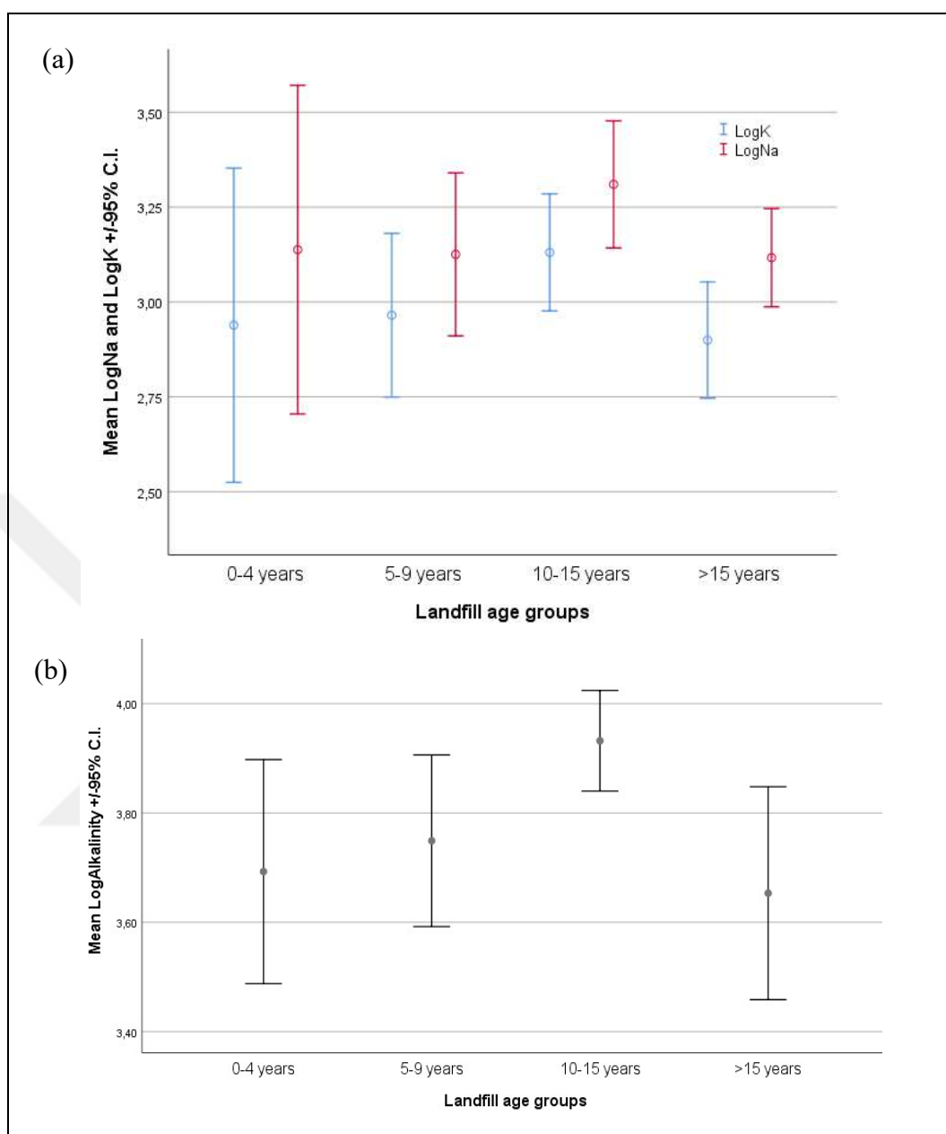
Figure 6.11. Confidence interval for mean values of (a) logK and LogNa (b) logAlkalinity at each landfill age case for the first climate group
