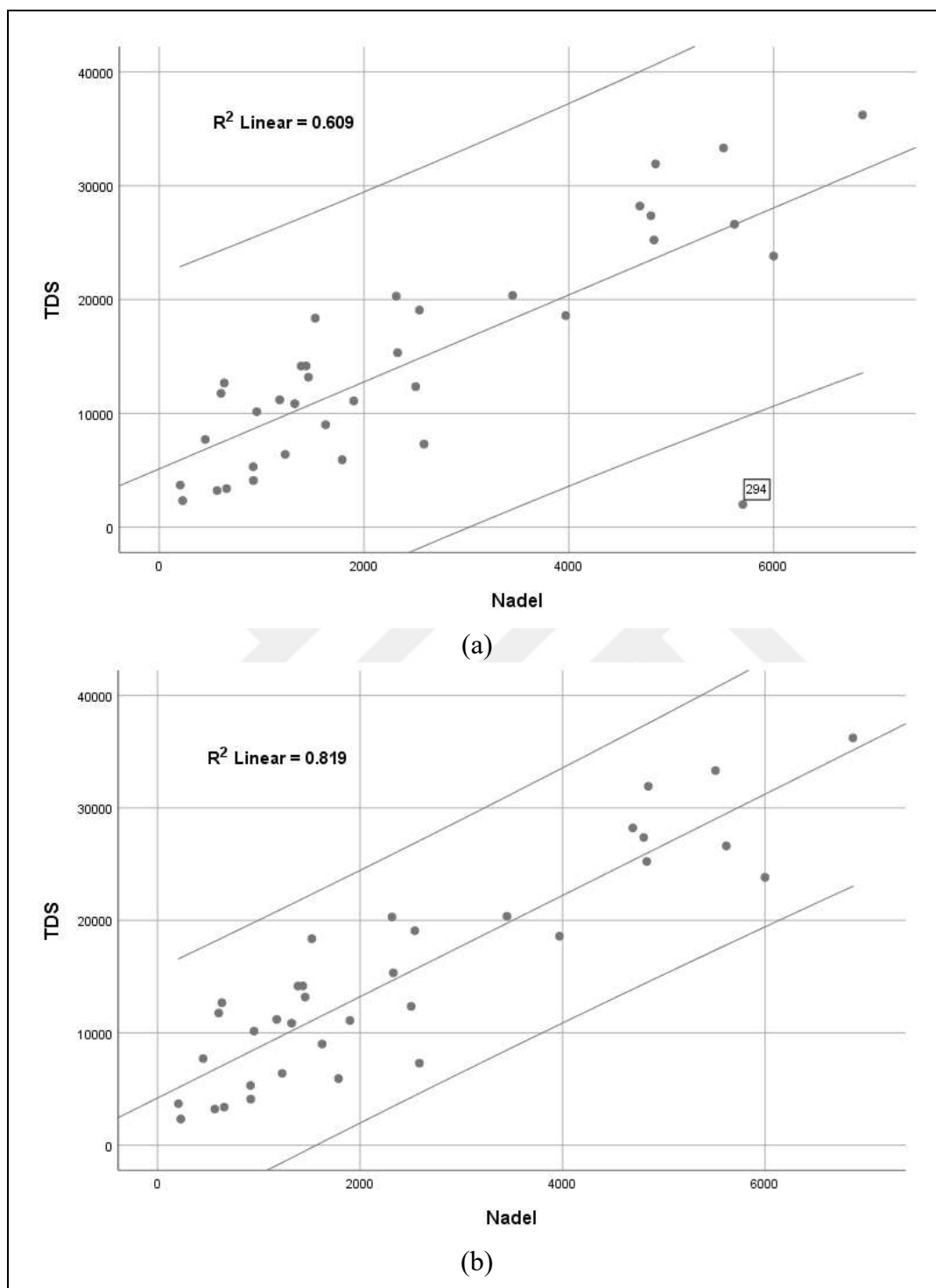
Figure B.4. Outlier data (circled) in scatter plot for Na vs TDS (a) with outlier data (b) After removal of outlier data (the upper and lower lines show 99% prediction interval; the numbers within boxes indicate landfill ID)
