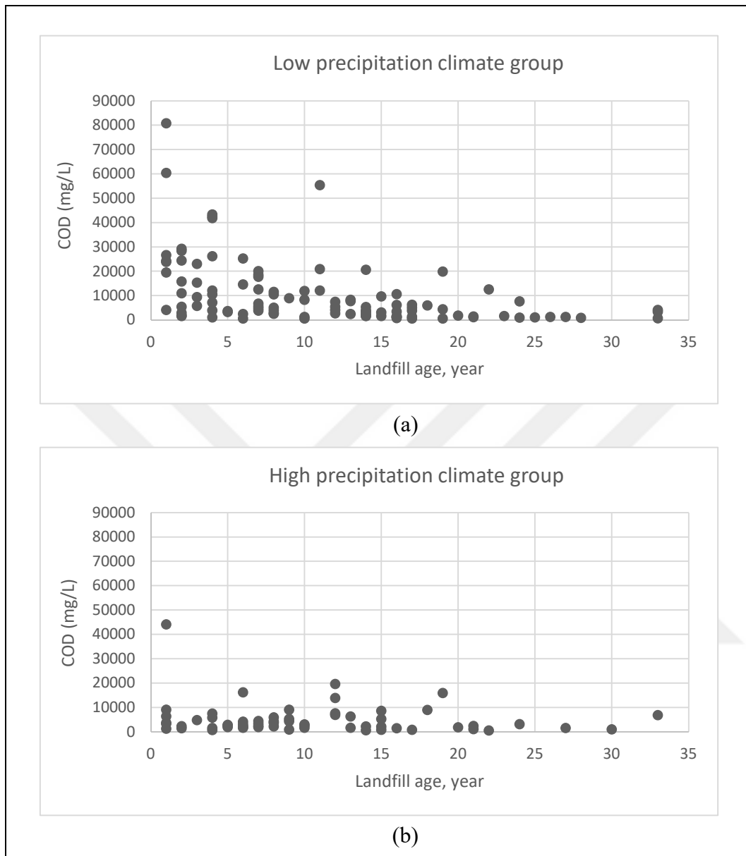
Figure 6.16. Scatter plots for the change in leachate COD content with time in (a) Low precipitation climate (b) High precipitation climate
