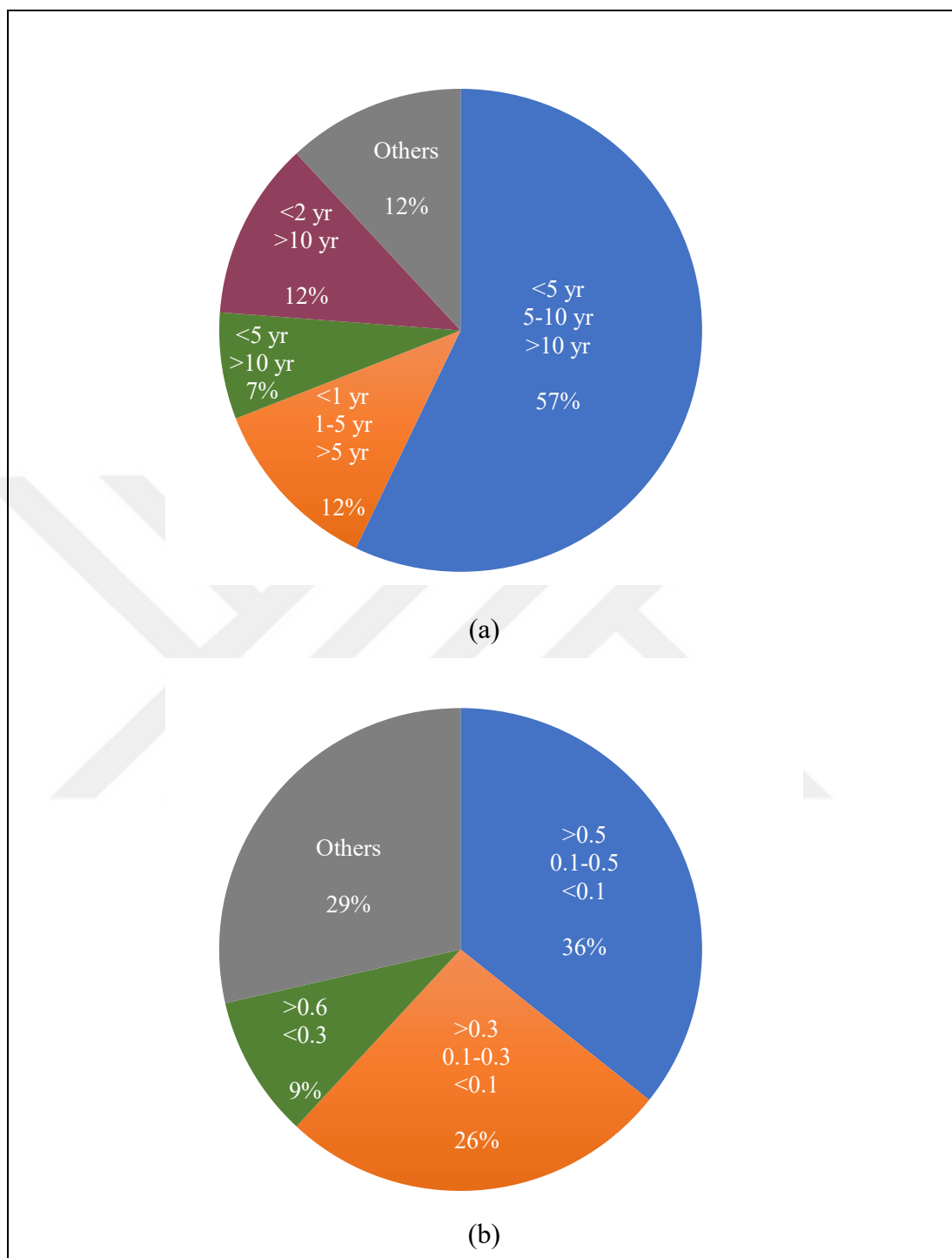
Figure 4.1. Distribution of (a) landfill age criteria (b) BOD/COD ratio used for leachate classification in 42 studies collated from literature
