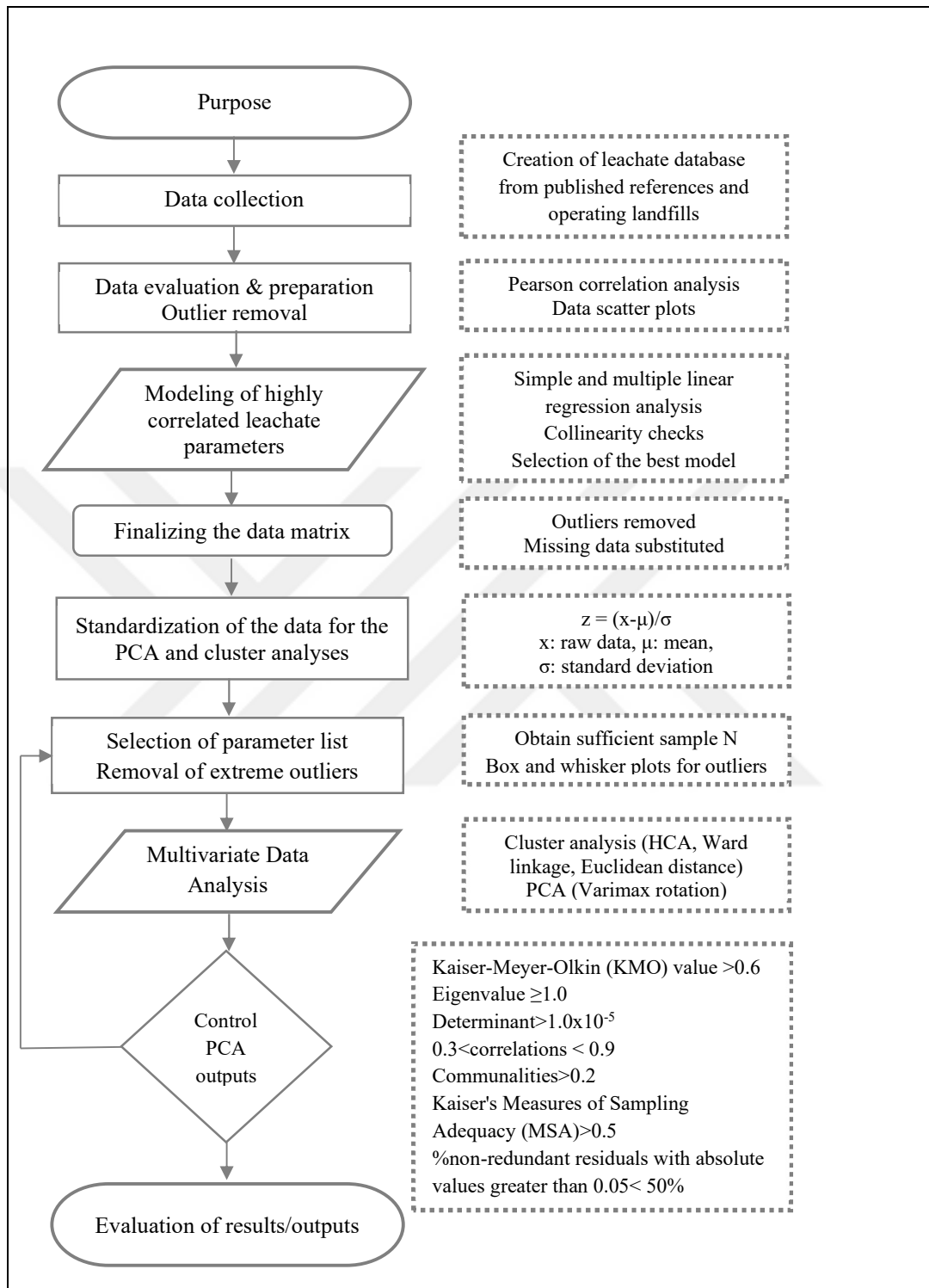
Figure 5.1. Flowchart for data collection, preparation, and analysis steps
