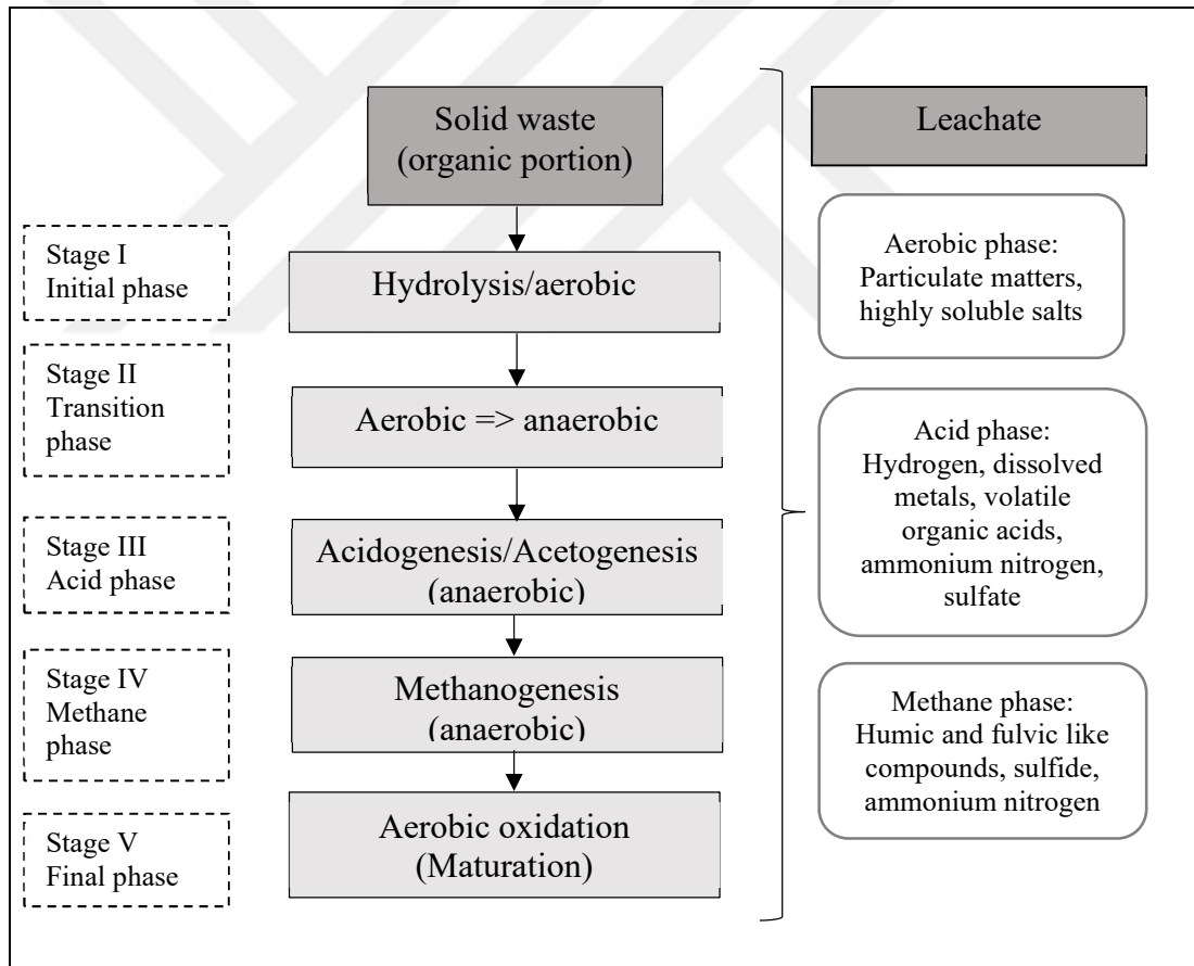
Figure 2.2. Waste decomposition stages in a landfill and related leachate composition
