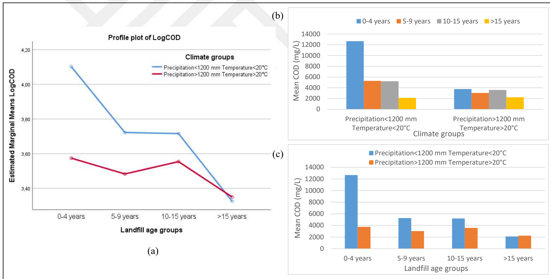
Figure 6.7. ANOVA results for leachate COD in different age/climate groups (a) Profile plot (b) Mean COD values according to climate groups (c) Mean COD values according to landfill age groups
