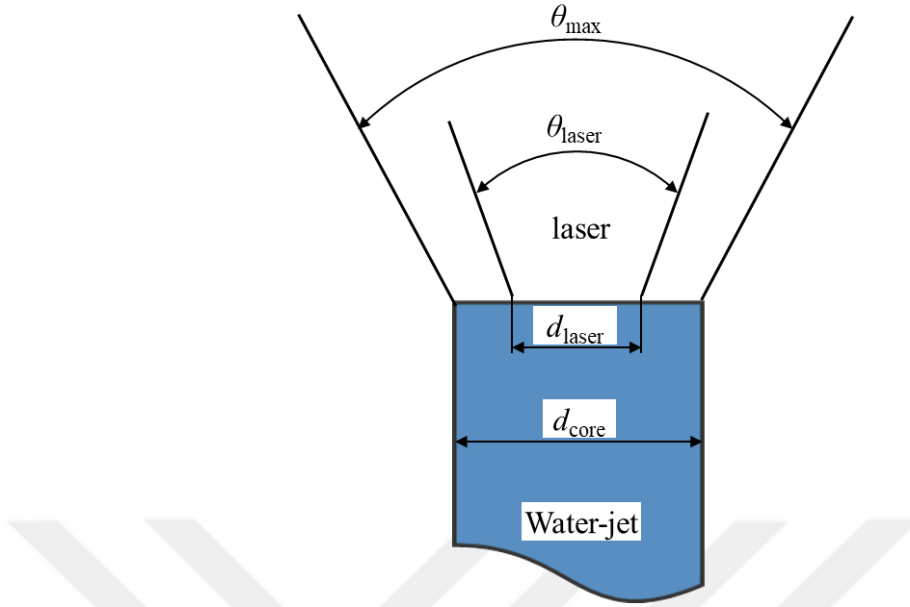
Figure 4.27. Water jet acceptance angle for the laser beam [115]
