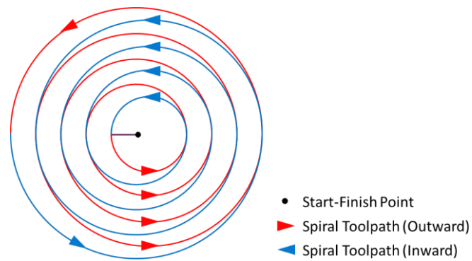
Figure 2.7. Spiral Toolpath
