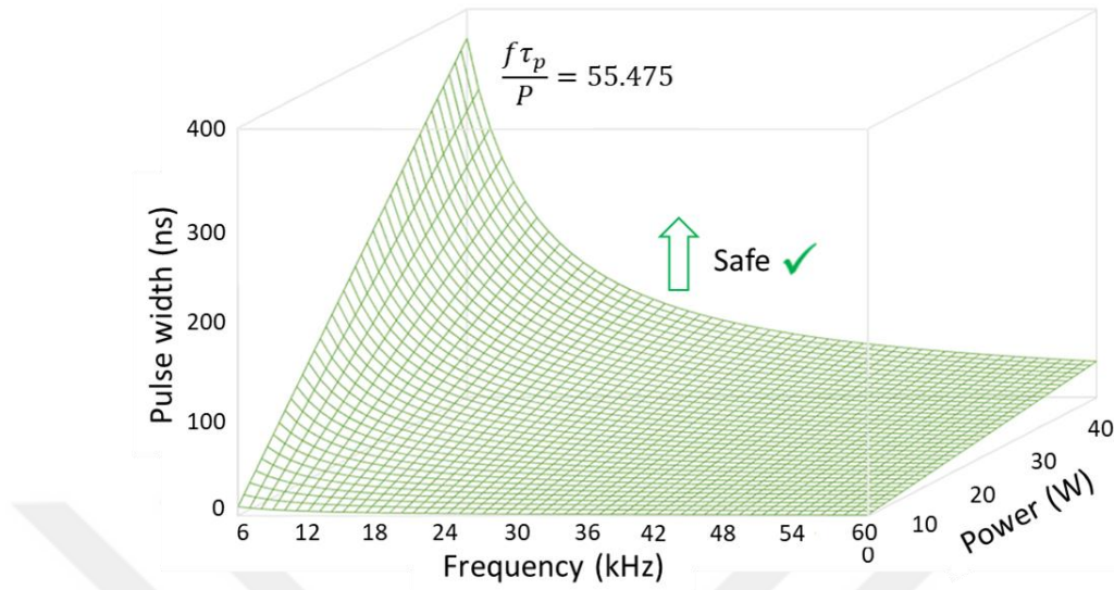
Figure 2.5. Design Space for the Laser Parameters
