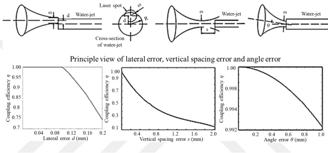
Figure 4.30. The relation of coupling offset error and coupling efficiency [116]
