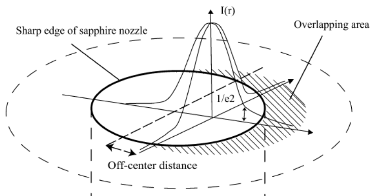
Figure 4.29. Misalignment problem [109]
