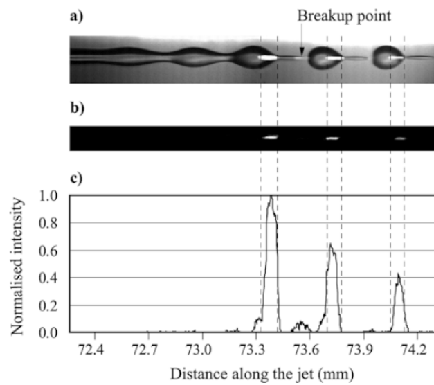
Figure 4.41. Breakup point [111]
