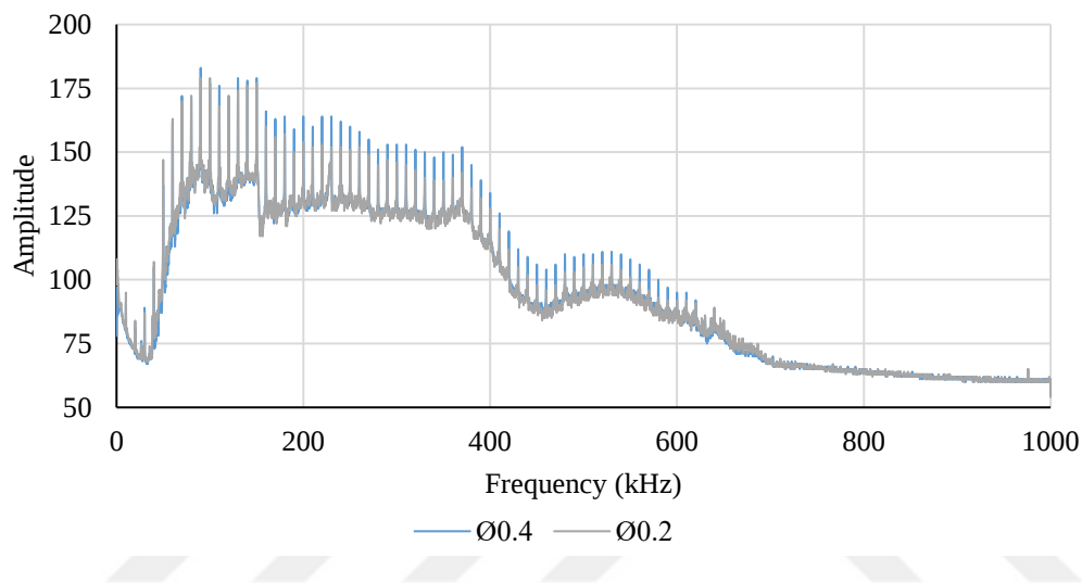
Figure 8.9. PSD comparison between Ø0.2 (mm) and Ø0.4 (mm) holes, 1 st cycles
