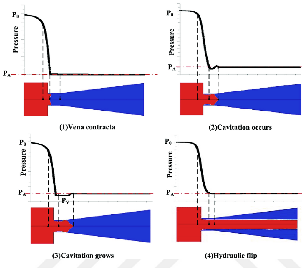
Figure 4.17. Formation of the hydraulic flip [105]
