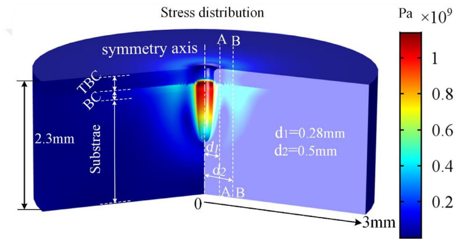
Figure 3.2. The Distribution of Thermal Stress After Five Pulses [20]
