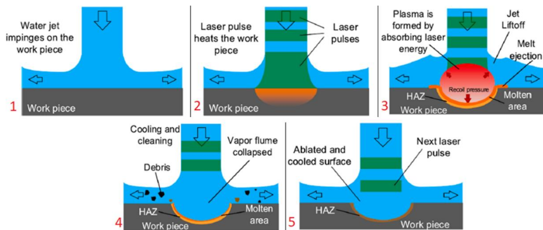
Figure 4.44. Ablation process [105]
