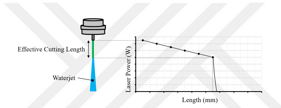
Figure 7.1. Effective cutting length
