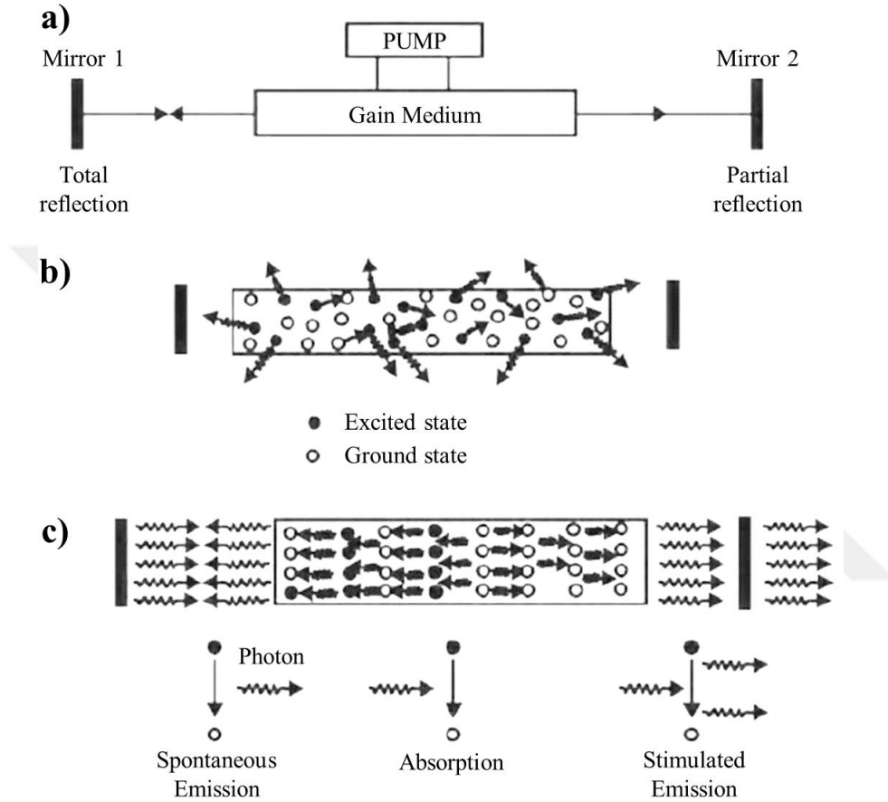
Figure 4.3. Inside a laser device [90]
