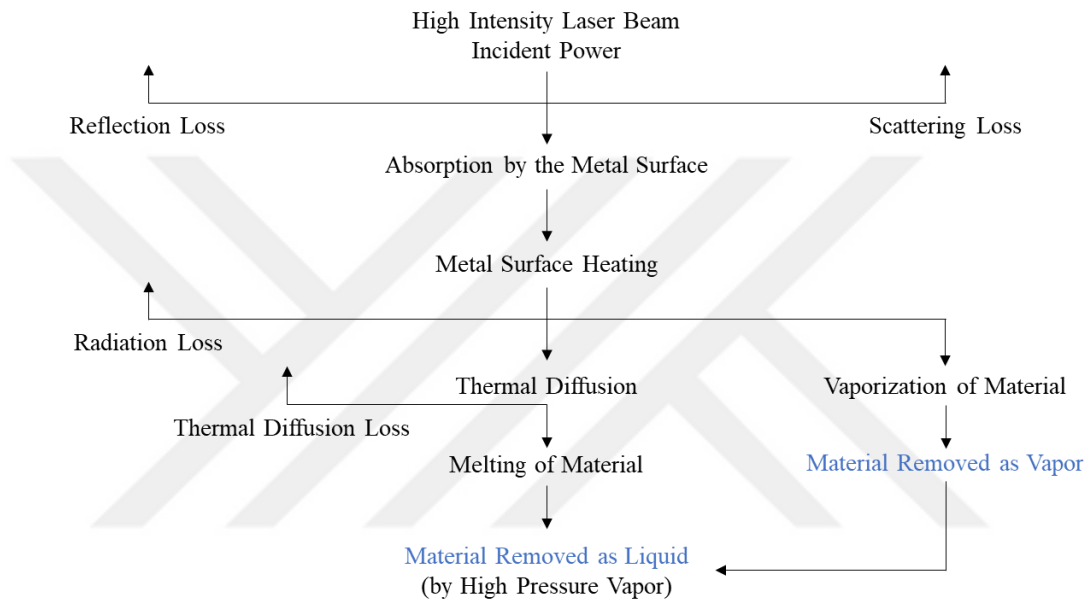
Figure 4.11. Material removal [92]
