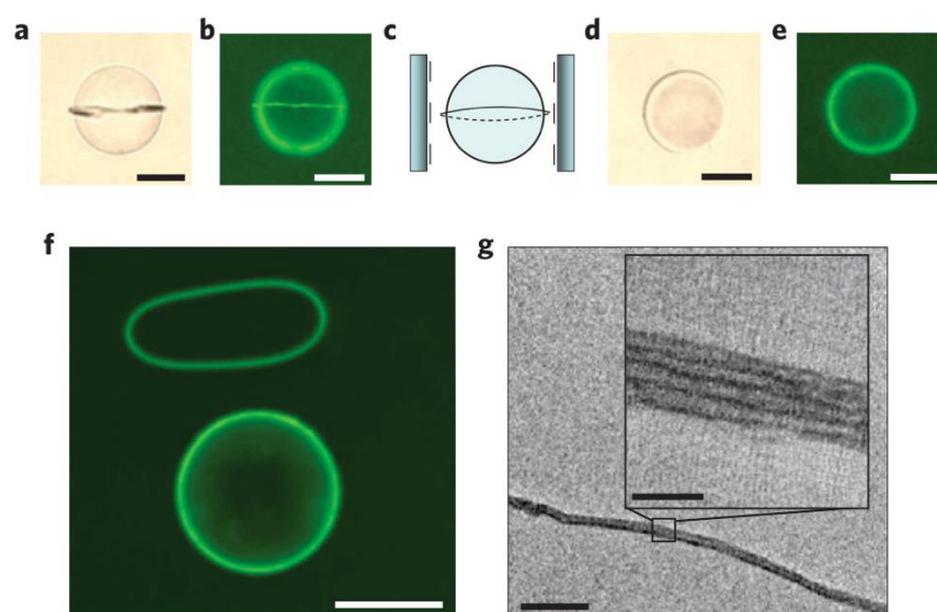
Figure 2.6 Reversible formation and in situ crosslinking of molecular assemblies of amphiphiles templated by a -1/2 'Saturn-ring' disclination line formed about microparticles. (a) Bright-field and (b) fluorescence micrographs representing the fluorescent dye doped photoreactive lipid that adsorbed on the disclination line formed in nematic 5CB, (c) Schematic illustration of a -1/2 'Saturn-ring' defect around particles dispersed in nematic LC with 0^\circ twist. (d) Bright-field and (e) fluorescence micrographs of the fluorescent dye doped photoreactive lipid that
