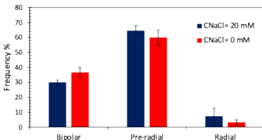
Figure 4.8 The distribution of configuration of 5CB droplets in the case of C_{NaCl}=0 and C_{NaCl}=20 \text{ mM}
