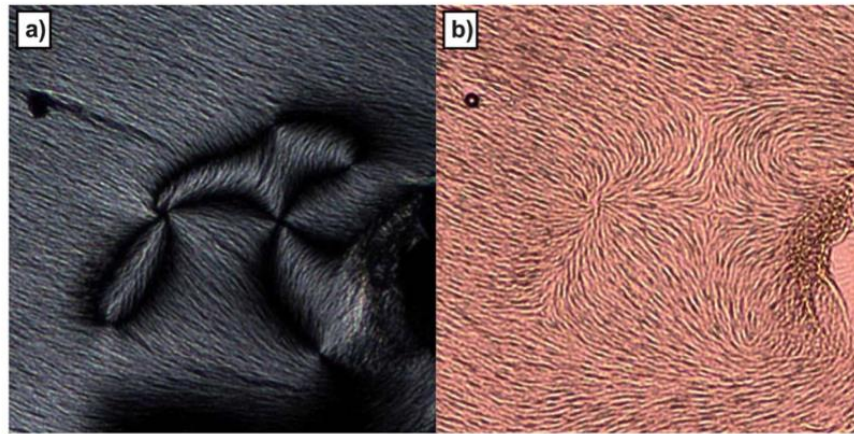
Figure 1.6 The defect director field is visualized through (a) the residual birefringence of LC and (b) reflection microscopy, both of which are non-invasive techniques. The images show the same region of a sample after polymerization of the mixture of 5% RM257 a and E7, illustrating the connection between an s = +1 defect and an s = -1 defect. These defects were formed by rapidly cooling a cell with planar boundary conditions 23 .
