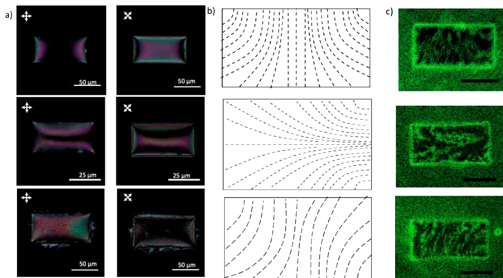
Figure 4.45 a) POM images of 5CB filled epoxy microwells in the case of medium of UP water, b) schematics of configuration of LC confined in epoxy microwells c) fluorescence images of FITC-SiNPs adsorbed on the LC orientation
