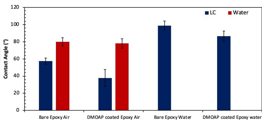
Appendix A.1 Contact Angle of UP water and LC (5CB) on bare and DMOAP coated epoxy surfaces
