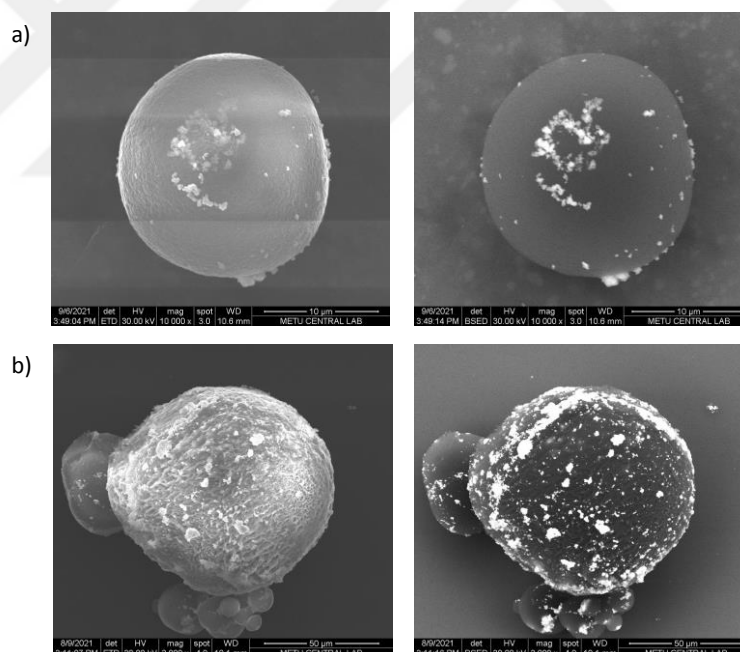
Figure 4.12 Scanning electron microscopy micrographs of polymerized droplets taken after the functionalized gold nanoparticles were adsorbed on droplets with the [COOH:C16] ratio determined as a) [4:1], b) [1:4]
