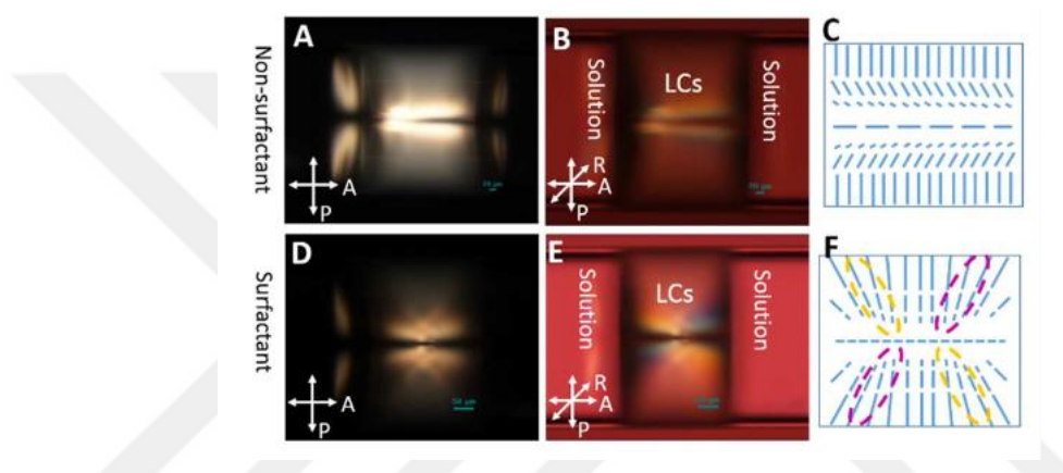
Figure 2.4 (A), (B), and (C) are the optical images and top view schematic of the microcapillary-confined LCs contacting the non-surfactant solutions; (D), (E), and (F) show the optical response and top view schematic of the microcapillary-confined LCs contacting the surfactant solutions. The purple and orange dashed circles in (F) indicate how the four-petal shape is formed. 42
