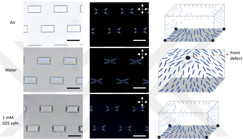
Appendix C.1 Optical microscope images of LC filled PDMS microwells in the case of LC-air, LC-water and LC-1 mM SDS solution and schematics of LC orientation in these microwells Arrows indicate the direction of the polarization of the polarizer and analyzer. Scale bars: 100 \mu\text{m}
