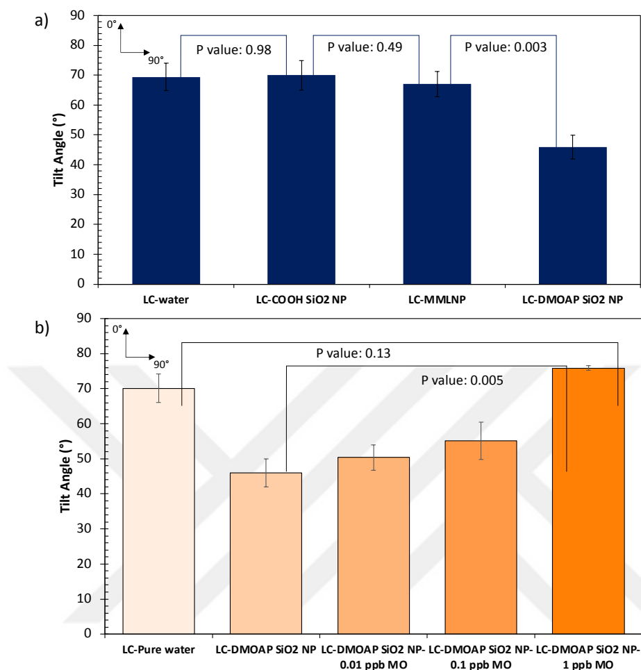
Figure 4.44 Tilt angles calculated from optical retardance in the case of a) adsorption of -COOH-terminated, COOH/DMOAP mixed monolayer coated and DMOAP coated silica nanoparticles. b) adsorption of DMOAP coated silica nanoparticles with MO concentration of 0.01, 0.1, 1 ppb (pH:5.0). The definition of the angles represented with arrows.
