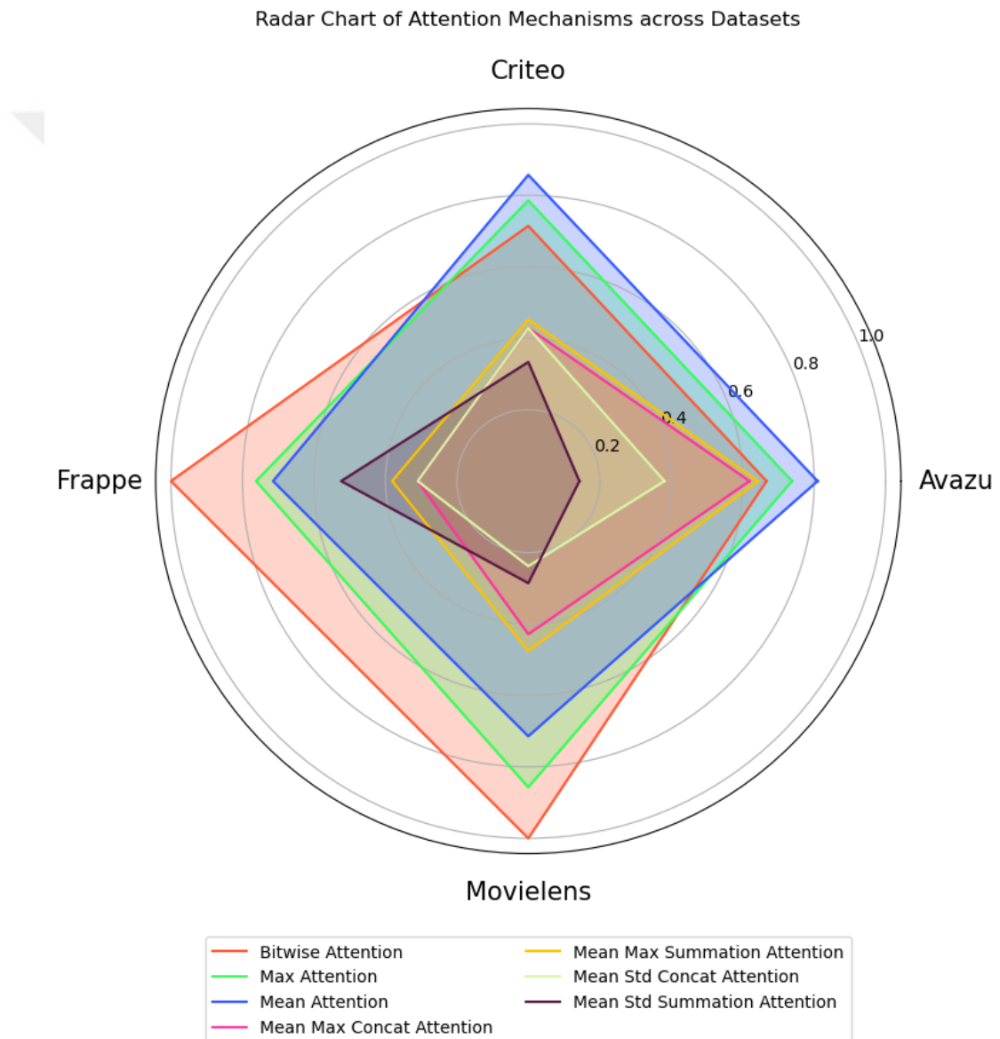
Figure 5.11: Radar Chart of Attention Mechanisms across the Datasets
