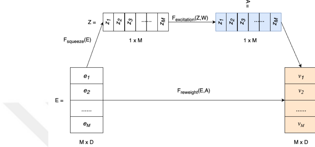
Figure 3.7: Overall architecture of SENet layer
