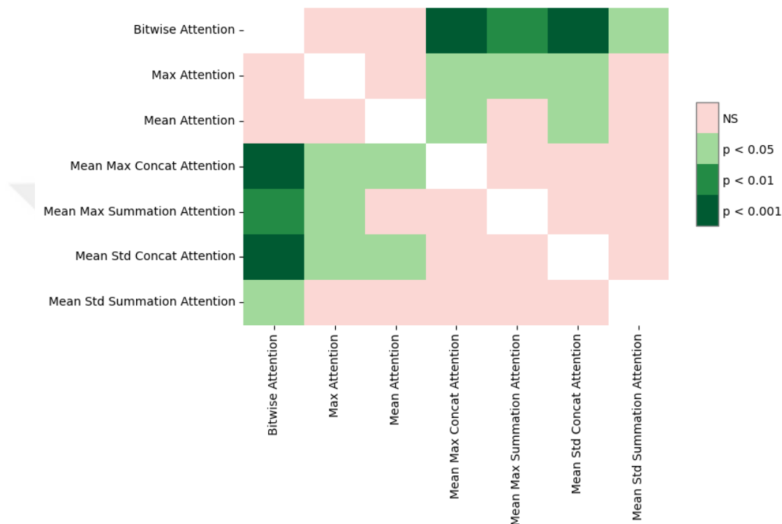
Figure 5.7: Conover posthoc test sign plot of attention mechanisms for Frappe Dataset
