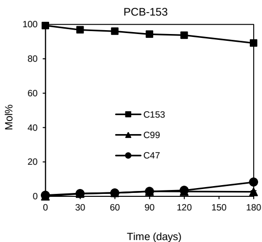
Figure 7.7. Mol% distributions of PCB 153 and its dechlorination products in 180 days of incubation
