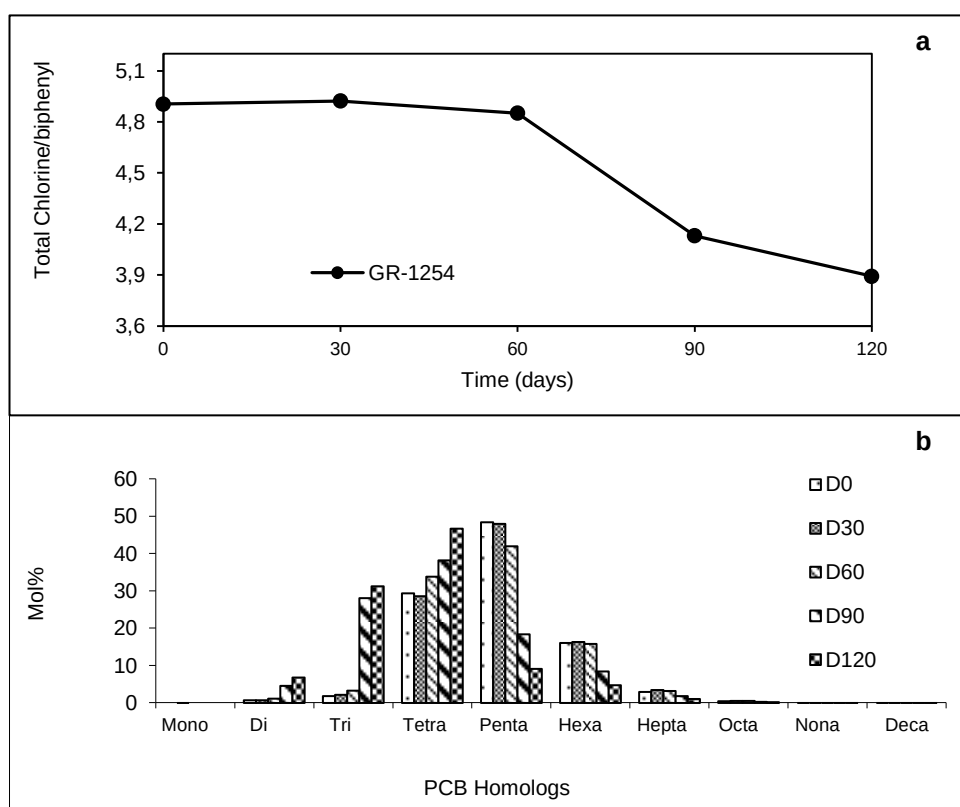
Figure 7.1. a) Changes in total chlorine per biphenyl values of first set of GR microcosms spiked with Aroclor 1254 and b) Homolog chlorine distributions of Aroclor 1254 in GR (D=day).
