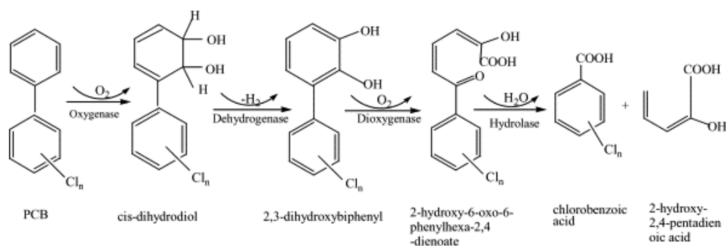
Figure 2.2. Major steps in the conversion of PCBs into chlorobenzoates (Borja et al. , 2005)
