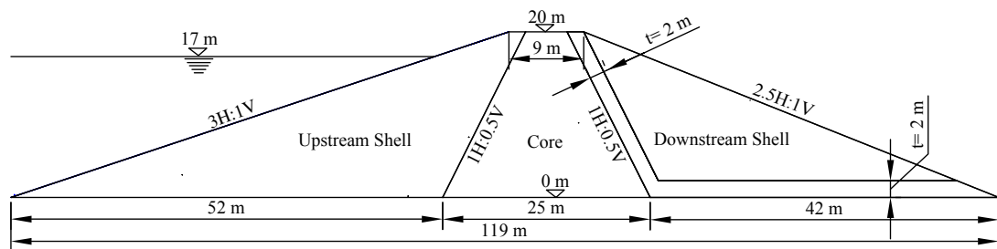
Figure 4.3: Model geometry
