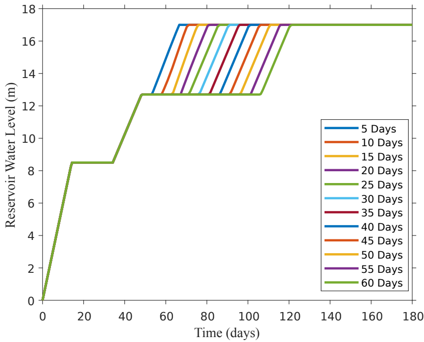
Figure 5.13: Applied boundary condition of filling schedule
