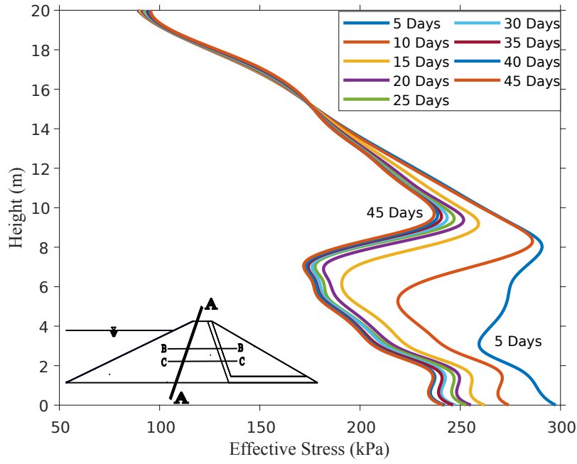
Figure 5.3: Effective stress variations for different first hold durations on section A-A
