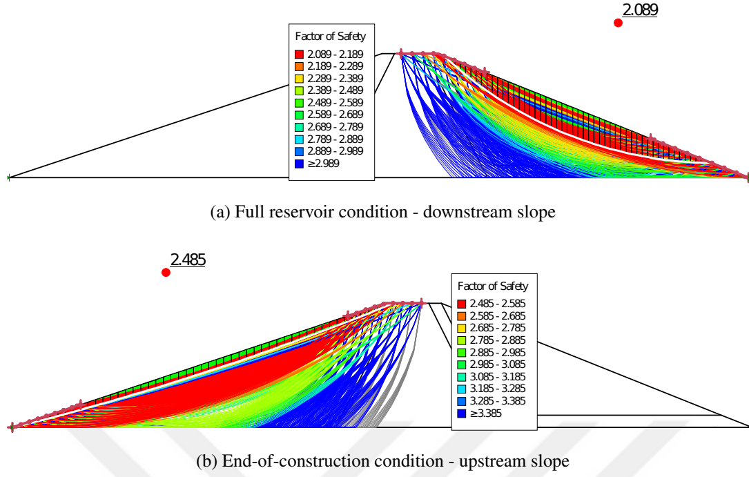
Figure 5.1: Slope stability analyses
