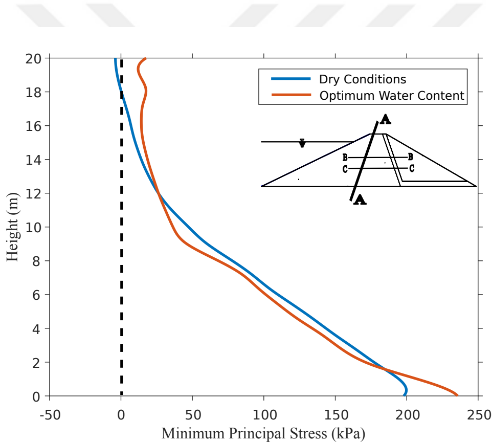
Figure 5.32: Effective stress on section A-A at the end of first hold for different initial conditions
