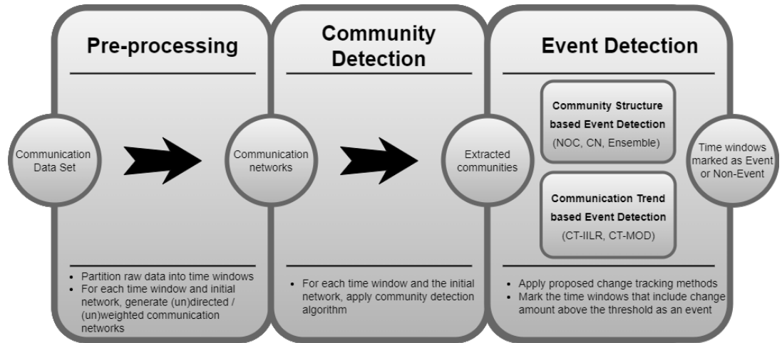
Figure 4.1: The Overview of the Method
