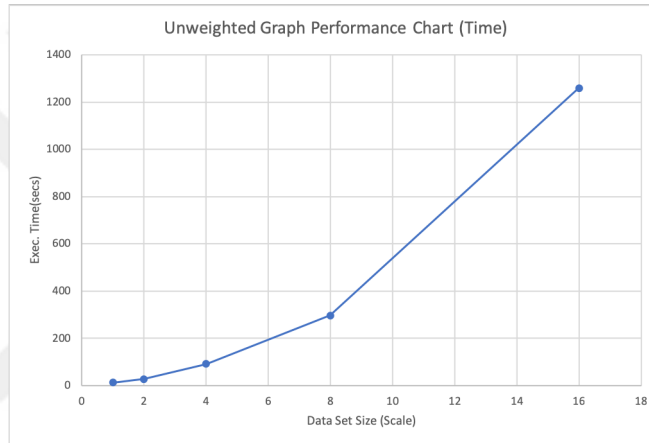
Figure 5.3: Unweighted Graph: Exec. Time/Data Set Size
